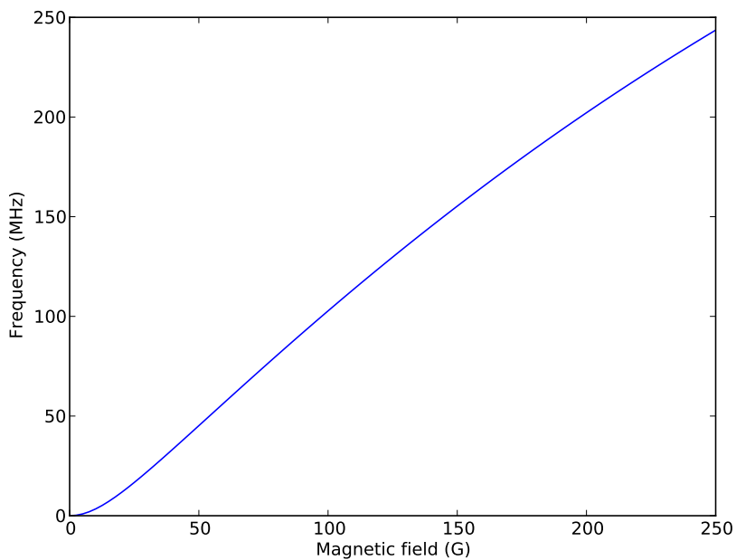
Figure 2.15: Theoretical frequency shift of the 1S_{1/2} \rightarrow 3S_{1/2}(F = 1, m_F = 0) transition as a function of magnetic field. This curve is used to convert the measured m_F = 0 frequency points into magnetic field values.
