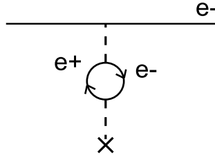
Figure 1.3: Feynman diagram of the one-loop contribution to vacuum polarization. A virtual electron-positron pair appears in the Coulomb propagator.
