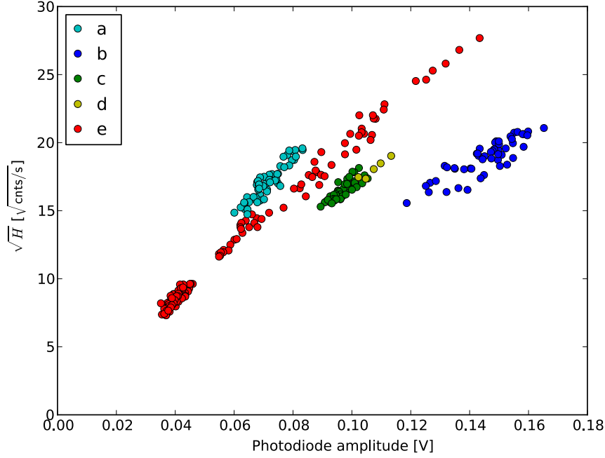
Figure 4.4: Square root of signal height as a function of the UV photodiode amplitude. Each point corresponds to a single run, recorded at zero magnetic field and low pressure. They have been grouped by day. a: first 2 days, b: next 3 days, c: last day before high pressure, d: first day after high pressure, e: four last days where the incoming light power was varied by hand to better quantify the light shift. The build-up cavity mirrors were cleaned just before these last four days, explaining the larger signal height.
