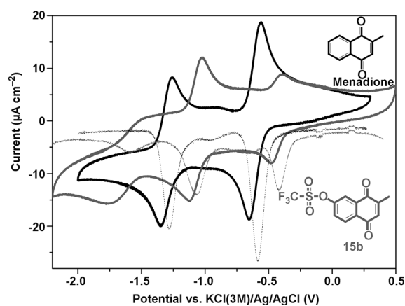
Figure 3. CV and SWV profiles of menadione (1.00 mM) and its 7-triflate substituted analogue 15 b (1.01 mM) measured in DMSO with 0.1 M n -Bu 4 PF 6 electrolyte support at 25 °C. v = 200 mV s -1 ; reference electrode = KCl (3 M)/Ag/AgCl; working electrode = glassy carbon disk of 0.07 cm 2 area; auxiliary electrode = Pt wire.
