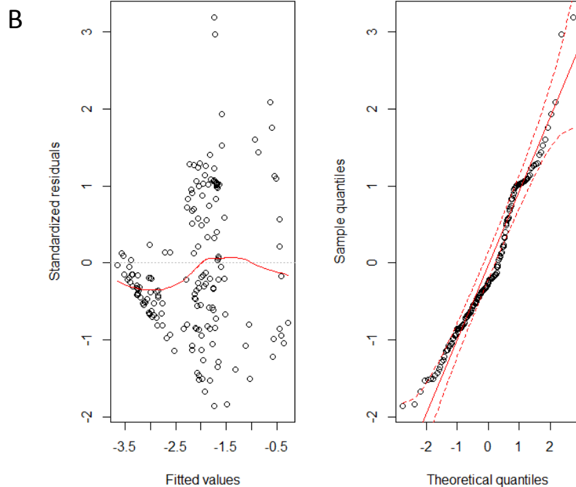
(A) Multi-panel scatterplot for oceanic data (behavioral mode). The upper/right panels show pairwise scatterplots between each explanatory variable (current speed, STT, depth, slope, CHL), and the lower/left panels contain Pearson correlation coefficients (B) Standard model validation graphs are: residuals versus fitted values to verify homogeneity and (left) and a QQ plot of the residuals for normality (right) of the most parsimonious model (LLM).
