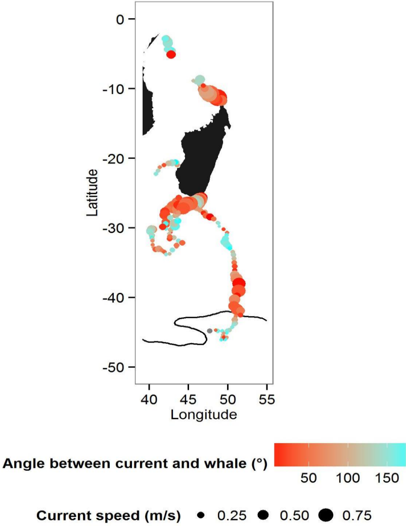
Figure 4.8. Current speed for each whale oceanic location. Color scale show angles between A and C vectors (A-C angles).
