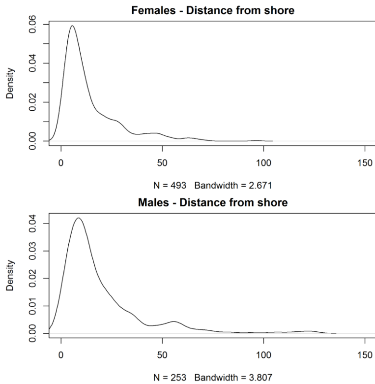
Figure S4.3. Density distributions of the distance from shore for females and males during coastal movements.
