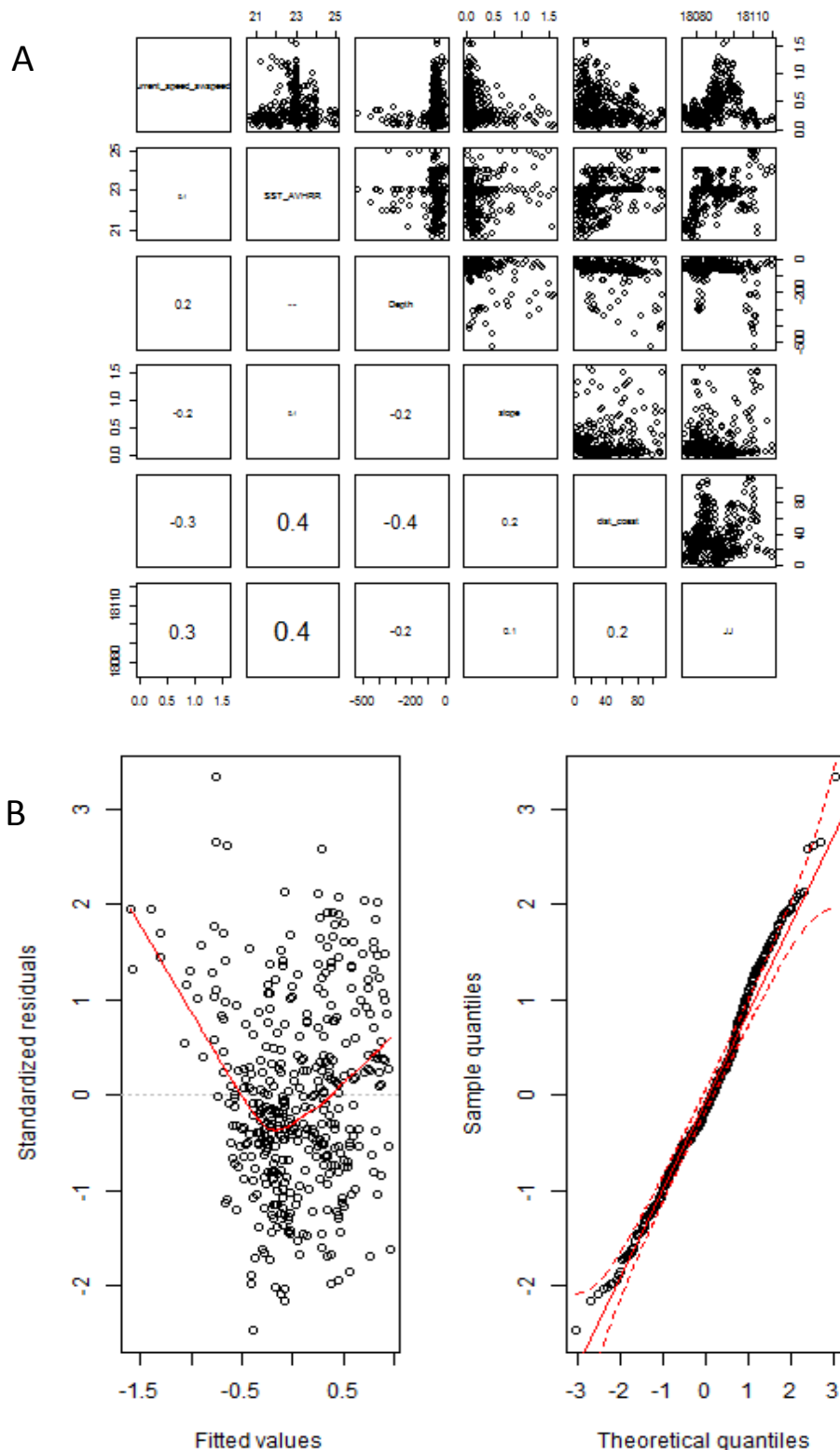
(A) Multi-panel scatterplot for male coastal data (swimming speed) from BSE1. The upper/right panels show pairwise scatterplots between each explanatory variable (current speed, SST, Depth, slope, distance from shore), and the lower/left panels contain Pearson correlation coefficients (B) Standard model validation graphs are: residuals versus fitted values to verify homogeneity and (left) and a QQ plot of the residuals for normality (right) of the most parsimonious model (LLM).
