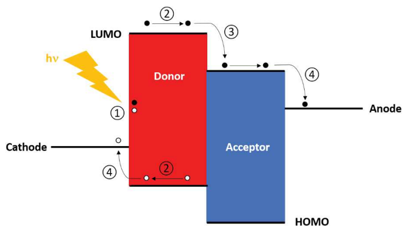
Figure 1.11 Schematic OPV device working principle from light absorption to charge collection.
