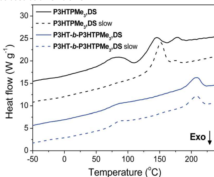
Figure 3.12 RHC thermograms of P3HTPMe 3 ,DS and P3HT- b -P3HTPMe 3 ,DS at 500 \text{ K}\cdot\text{min}^{-1} heating rate, for a preceding cooling rate of either 500 \text{ K}\cdot\text{min}^{-1} (solid lines) or 20 \text{ K}\cdot\text{min}^{-1} (dashed lines). The curves are shifted vertically for clarity.
