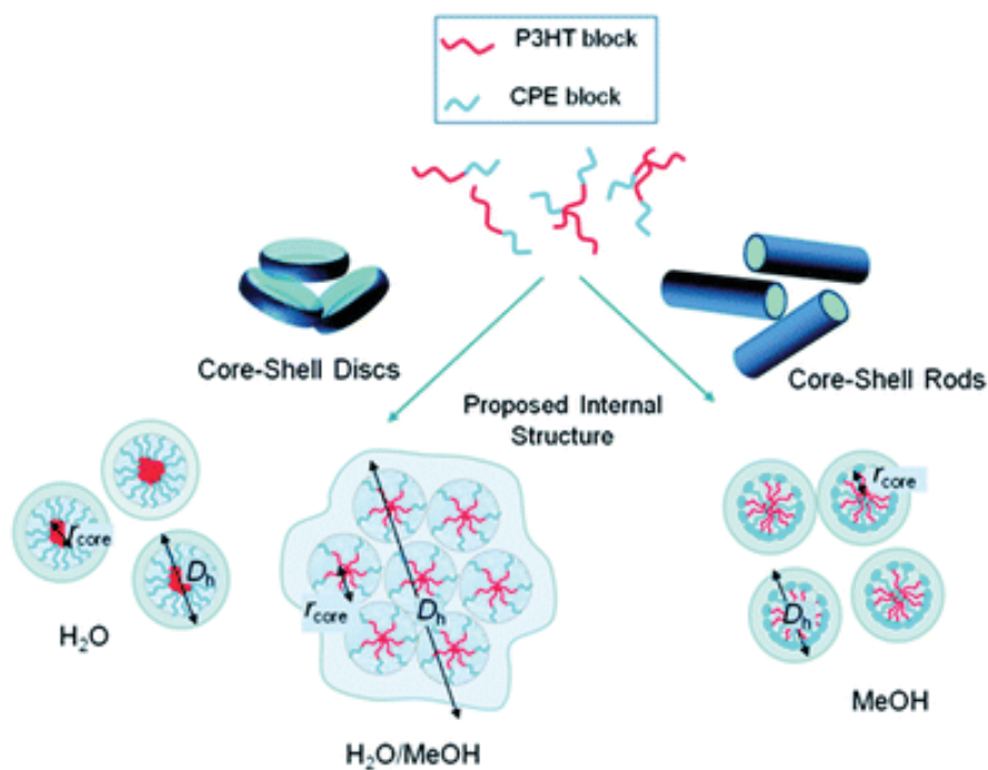
Figure 3.21 Schematic representation of the proposed internal aggregate structures of P3HT- b -CPE,Br in H 2 O, MeOH and H 2 O/MeOH mixtures.
