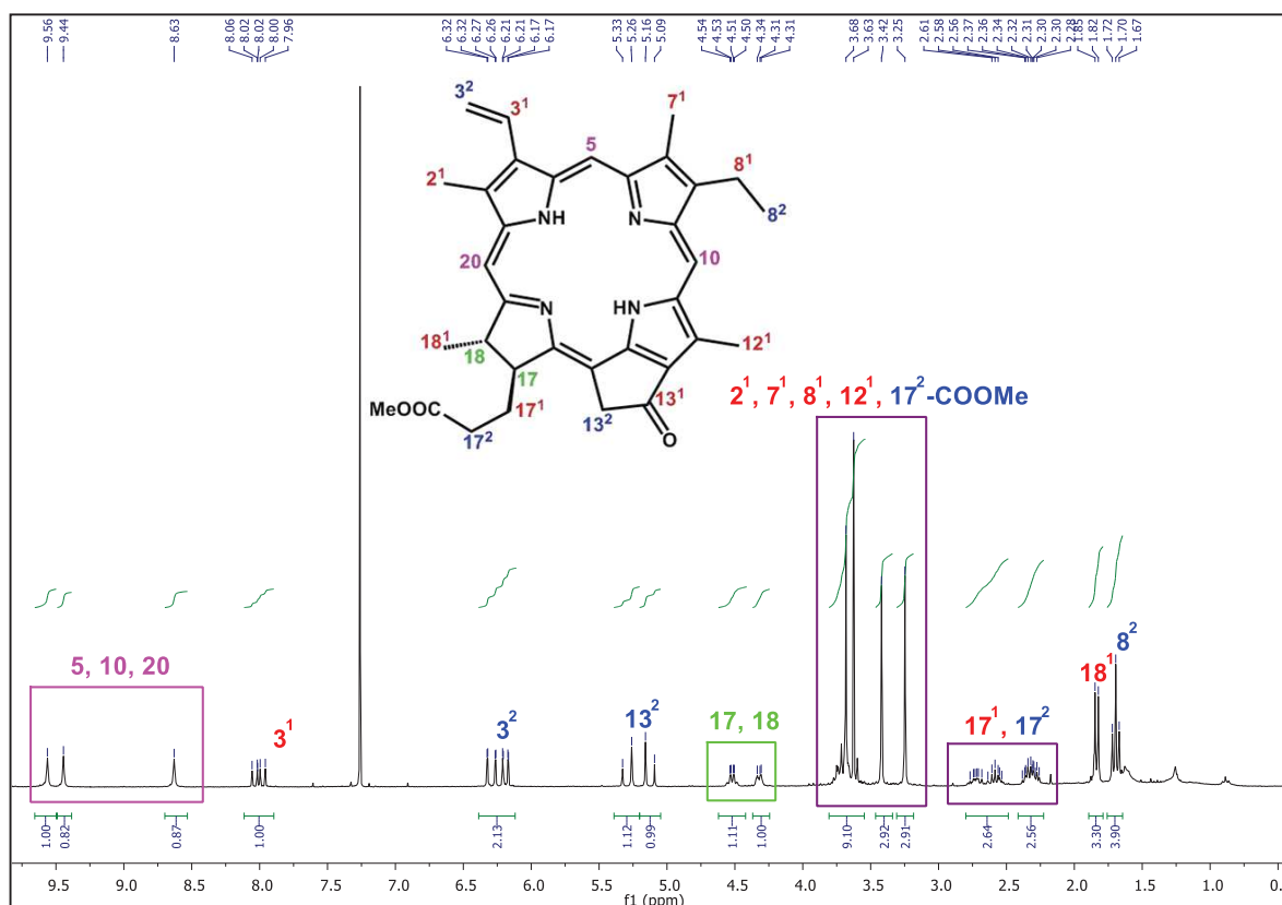
Figure 4.7 ^1\text{H} NMR spectrum of methyl pyropheophorbide- a in \text{CDCl}_3 .
