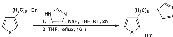
Scheme 2.3 Synthesis of 3-[6'-(1''-imidazolyl)hexyl]thiophene ( TIm ).
