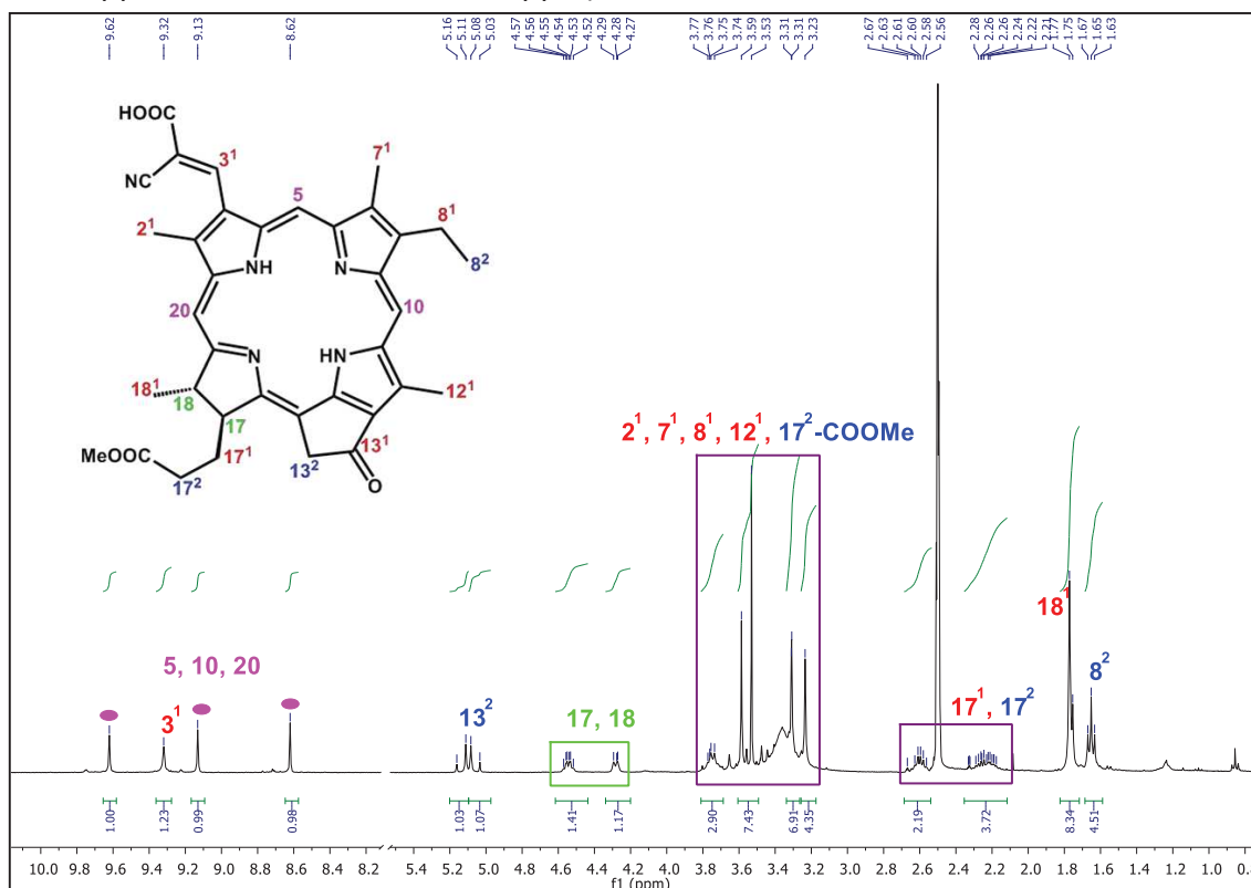
Figure 4.10 ^1\text{H} NMR spectrum of CNCOOH derivative M5 in \text{DMSO-}d_6 .
