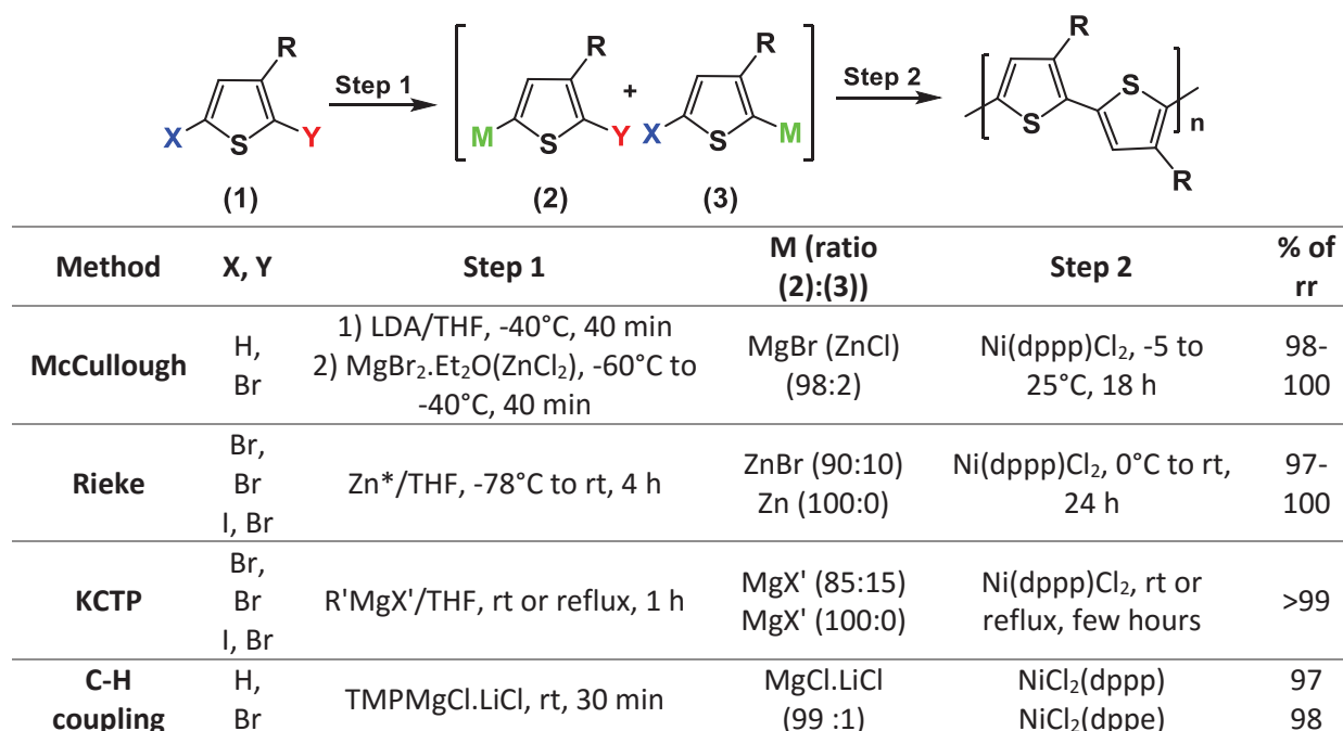
Figure 1.21 McCullough, Rieke, KCTP and C-H coupling methods for the synthesis of rrP3ATs .
