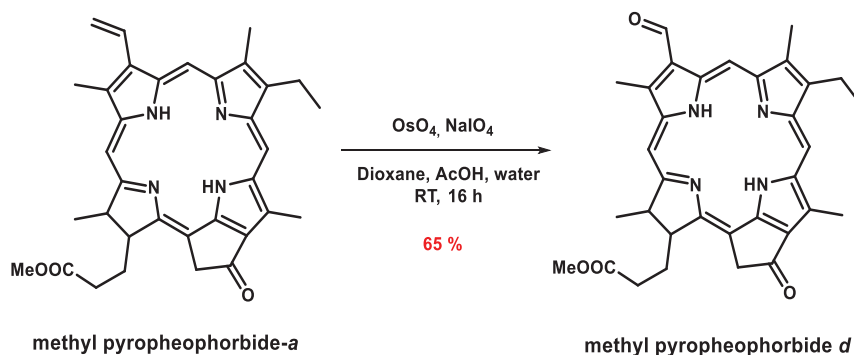
Scheme 4.4 Synthesis of methyl pyropheophorbide- d .
