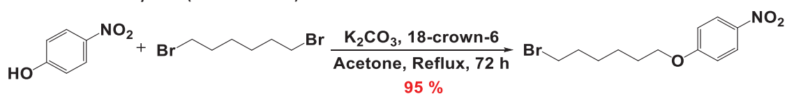
Scheme 2.7 Synthesis of the spacer 1-((6-bromohexyl)oxy)-4'-nitrobenzene.
