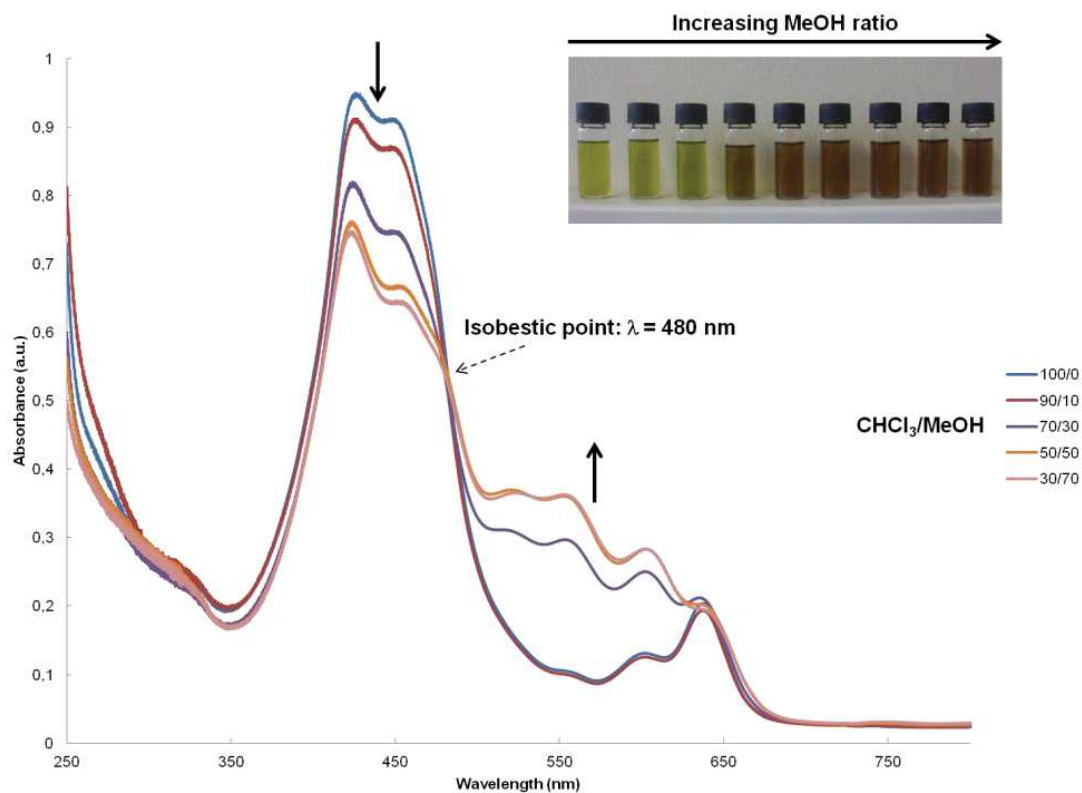
Figure 2.23 Photographs and UV-vis absorption spectra of 3a in chloroform/methanol mixtures from 10/0 to 3/7 ( \text{CHCl}_3/\text{MeOH} = v/v , C = 0.06 \text{ mg}\cdot\text{mL}^{-1} ).
