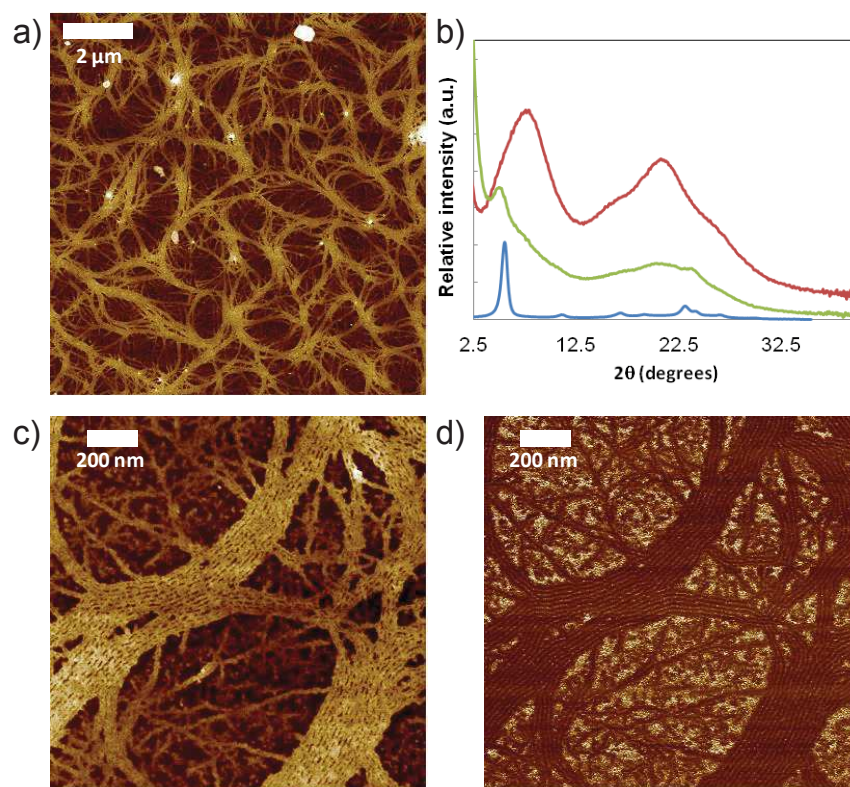
Figure 2.27 (a) 10 x 10 μm 2 Peak Force AFM height image of 3a drop-cast from xylene onto a mica substrate; (b) X-ray diffraction pattern of isocyanide-based porphyrin monomer CN-Spacer-NiTPP (red), P3HT (blue) and 3a (green); (c,d) 1.5 x 1.5 μm 2 Peak Force AFM height (c) and DMT modulus (d) images of 3a showing the fibrillar morphology.
