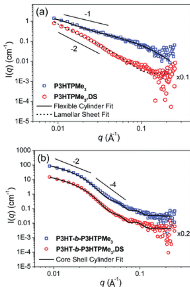
Figure 3.22 SANS data for (a) P3HTPMe 3 ,Br (blue) and P3HTPMe 3 ,DS (red) and (b) P3HT- b -P3HTPMe 3 ,Br (blue) and P3HT- b -P3HTPMe 3 ,DS (red). Total concentration of each sample was 10 mg mL -1 in d4 -MeOD. Solid and dashed lines correspond to the fits to the models described in the text.
