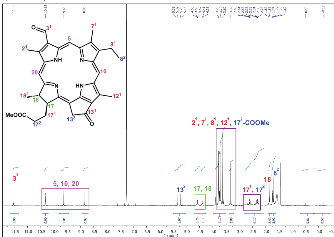
Figure 4.9 1 H NMR spectrum of methyl pyropheophorbide- d in CDCl 3 .
