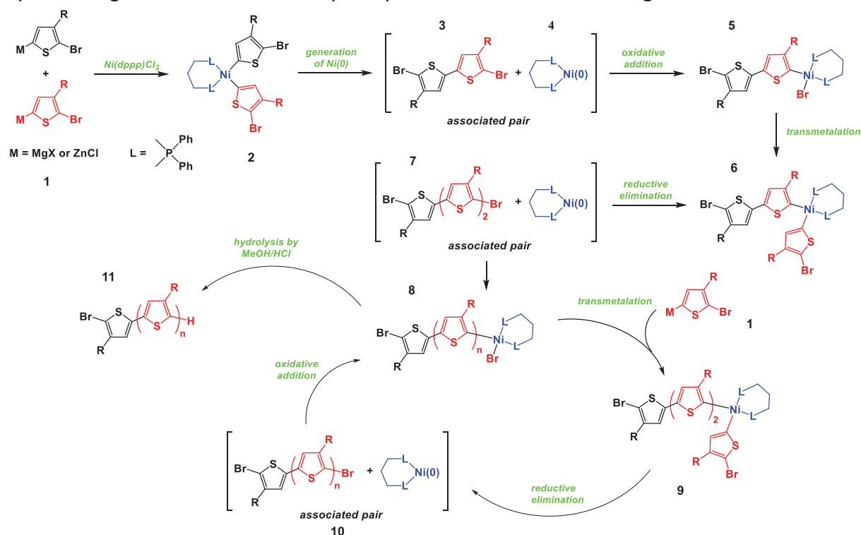
Scheme 1.4 Mechanism of the KCTP method proposed by McCullough and Yokozawa. 83
