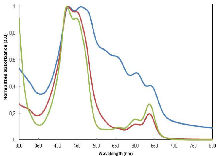
Figure 2.22 Normalized UV-visible absorption spectra of isocyanide-based porphyrin monomer CN-Spacer-NiTPP in chloroform (green curve), 3a in chloroform (red curve) and 3a in solid state (blue curve).
