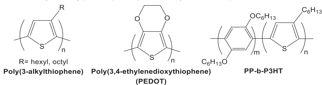
Figure 4.23 Chemical structures of conjugated polymer hole transporting materials.
