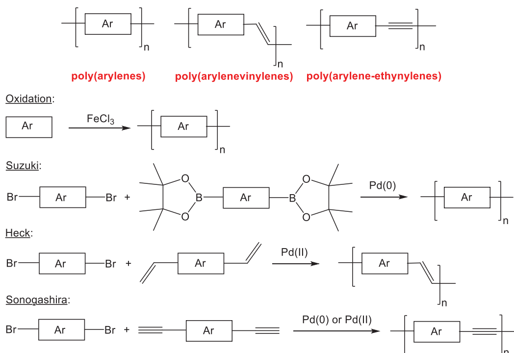
Figure 3.3 Examples of the most widely used polymerization methods; Ar represents aromatic structure.
