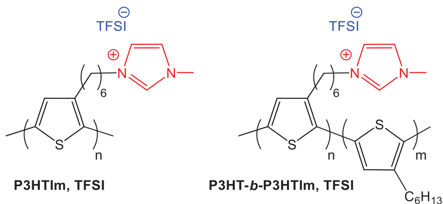
Figure 4.24 Molecular structures of the P3HT-based conjugated polyelectrolytes.
