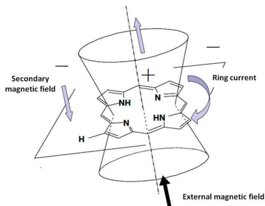
Figure 2.4 Anisotropic shielding effect of the porphyrin.
