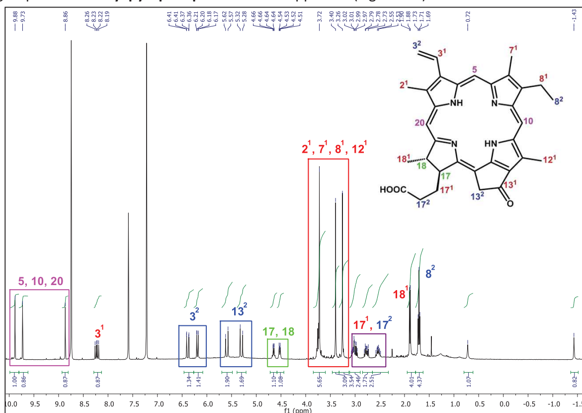
Figure 4.8 ^1\text{H} NMR spectra of the alkyl free-base M1 in deuterated pyridine.
