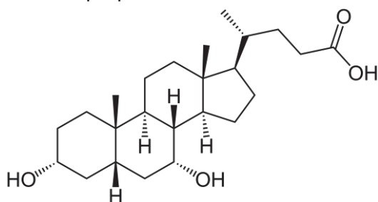
Figure 4.13 Chenodeoxycholic acid structure.
