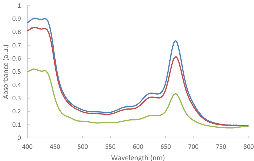
Figure 4.22 UV-Visible absorption spectra of M2 adsorbed onto TiO 2 film with different thickness (1.6 μm: green line; 3.2 μm: red line; 3.6 μm: blue line).
