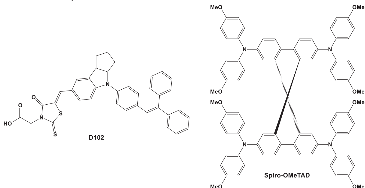
Figure 4.11 Structures of D102 (dye) and spiro-OMeTAD (HTM).
