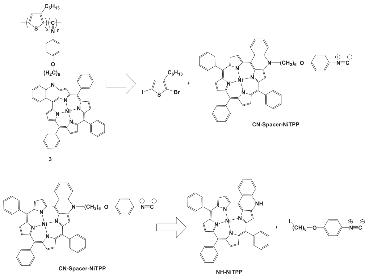
Scheme 2.5 Retrosynthesis of the porphyrin end-functionalized P3HT .
