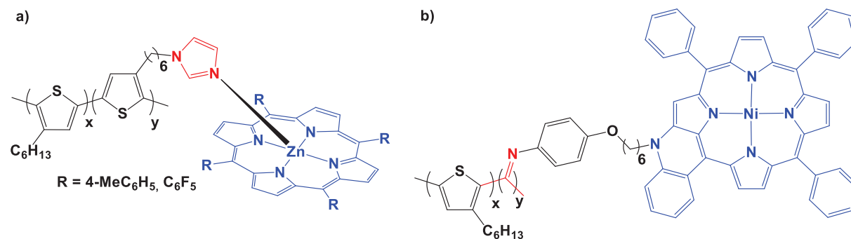
Figure 2.3 Structures of the porphyrin-polythiophene polymers studied in this chapter.
