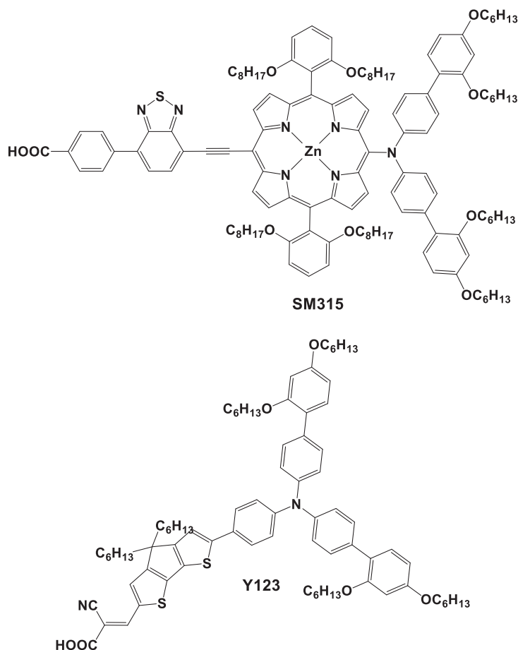
Figure 4.4 Chemical structures of the porphyrin sensitizer SM315 and the co-sensitizer Y123 , which yielded 13 % efficiency.
