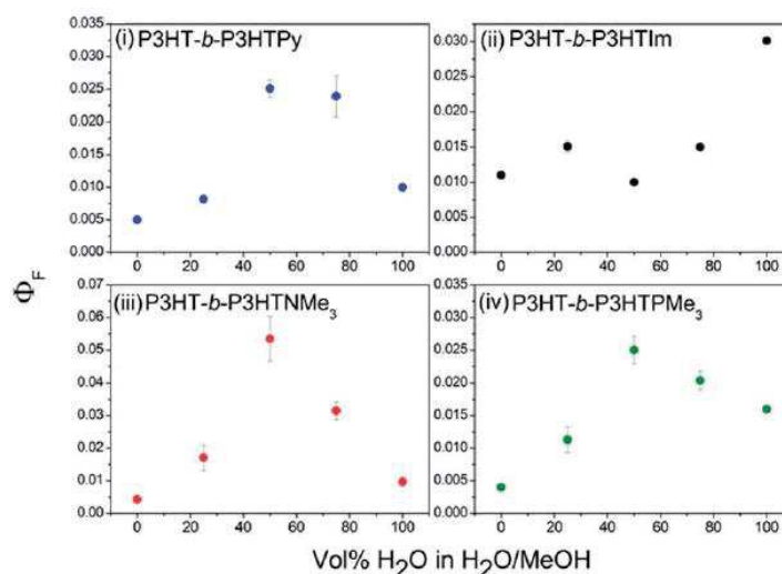
Figure 3.15 Fluorescence quantum yields ( \Phi_F ) of P3HT- b -CPEs,Br in H 2 O/MeOH solvent mixtures (0.35 \mu\text{g}\cdot\text{mL}^{-1} ).
