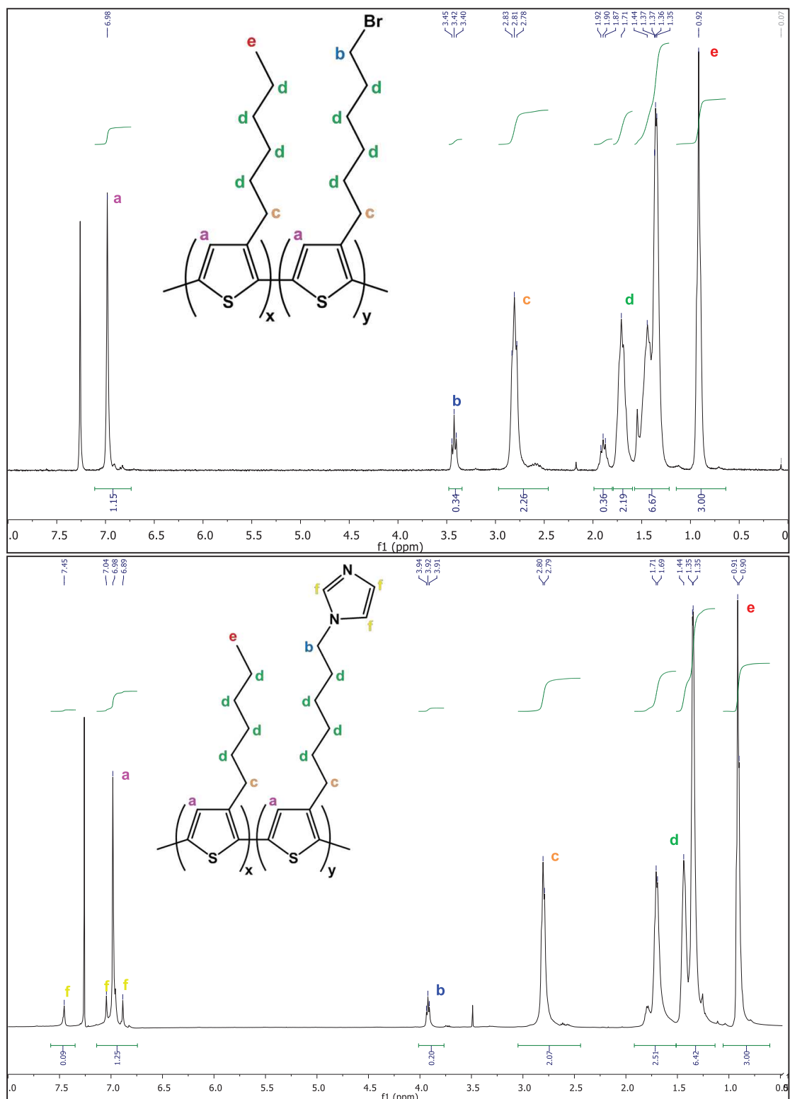
Figure 2.7 1 H NMR spectra of P3HT- r -P3HTBr (top) and P3HT- r -P3HTIm (bottom) in CDCl 3 .
