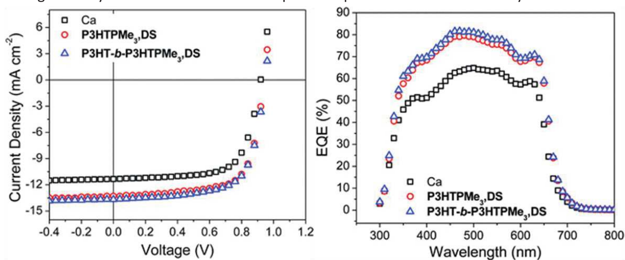
Figure 3.26 J–V (left) and EQE (right) curves for average performance PBDTTPD:PC 71 BM solar cell devices produced with and without CPE interlayers (0.5 mg.mL -1 deposition solution).
