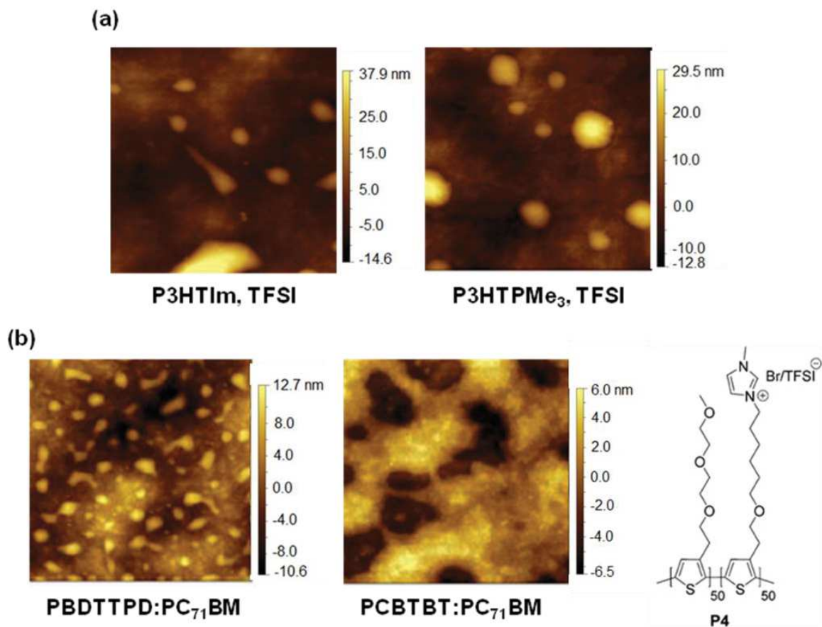
Figure 3.25 1 \times 1 \mu\text{m}^2 (a) AFM height images of the polymer solar cells ( PBDTTPD:PC 71 BM ) integrating P3HTIm,TFSI (left) and P3HTPMe 3 ,TFSI (right) as cathode interfacial layer. (b) AFM height images of devices with P4,TFSI cathode interlayer on the top of PBDTTPD:PC 71 BM (left) and PCDTBT:PC 71 BM (right) photoactive layers.
