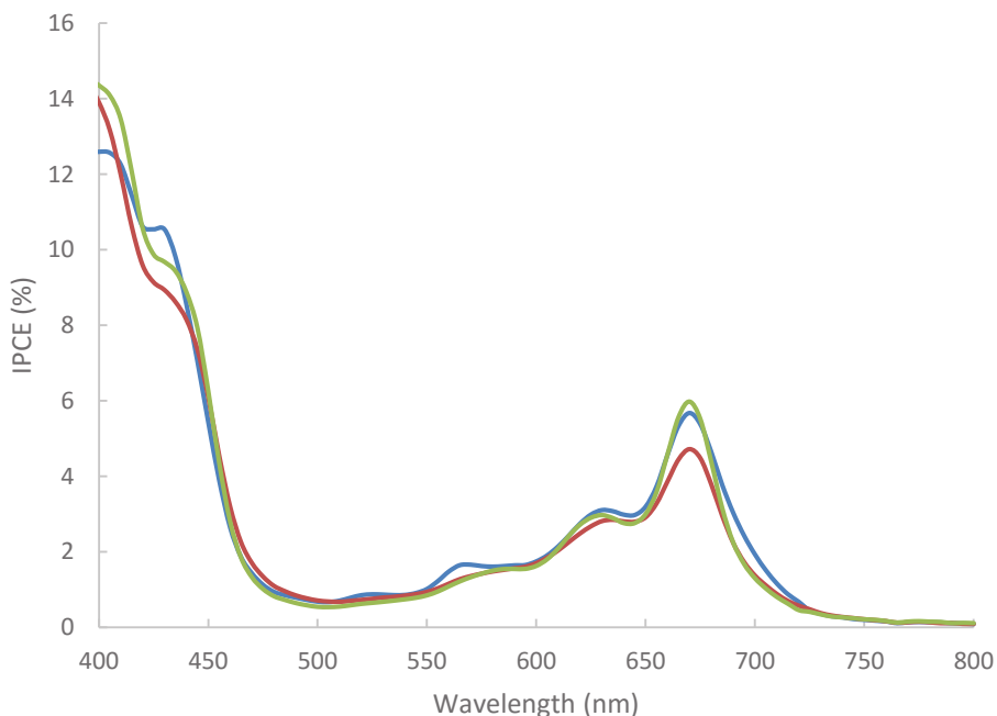
Figure 4.21 IPCE spectra of ss-DSSCs based on chlorin M2 depending on the nature of the solvent (ethanol: blue line, THF: red line and ACN/tBuOH: green line).
