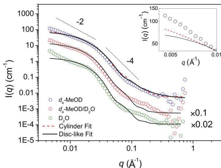
Figure 3.19 SANS data for P3HT- b -P3HTPy, Br in d 4 -MeOD, 50/50 (v/v) d 4 -MeOD–D 2 O and D 2 O (10 mg. mL -1 ). The solid black lines show the disc-like fits obtained using the Core–Shell-Cylinder model for each solvent mixture. Only P3HT- b -P3HTPy,Br in d 4 -MeOD was found to be better fit by rods at low q , as shown by the red dashed line in the inset.
