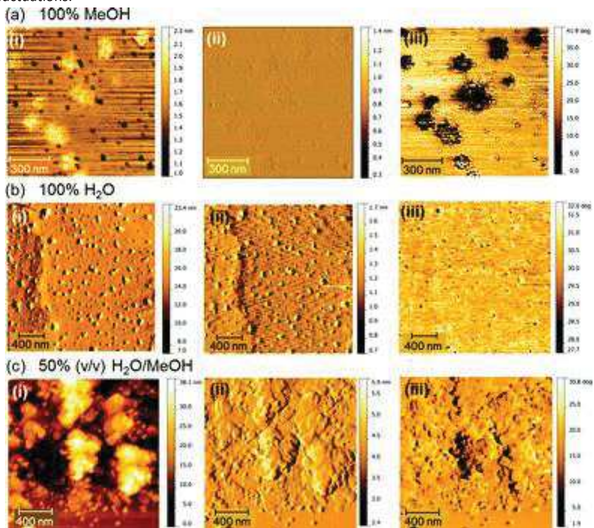
Figure 3.20 AFM tapping mode images of P3HT- b -P3HTIm,Br films drop-cast from (a) 100 % MeOH ( 7 \mu\text{g}\cdot\text{mL}^{-1} ), (b) 100 % H 2 O ( 3.5 \mu\text{g}\cdot\text{mL}^{-1} ) and (c) 50 % (v/v) H 2 O–MeOH ( 3.5 \mu\text{g}\cdot\text{mL}^{-1} ) onto mica: (i) height, (ii) amplitude and (iii) phase images, respectively.
