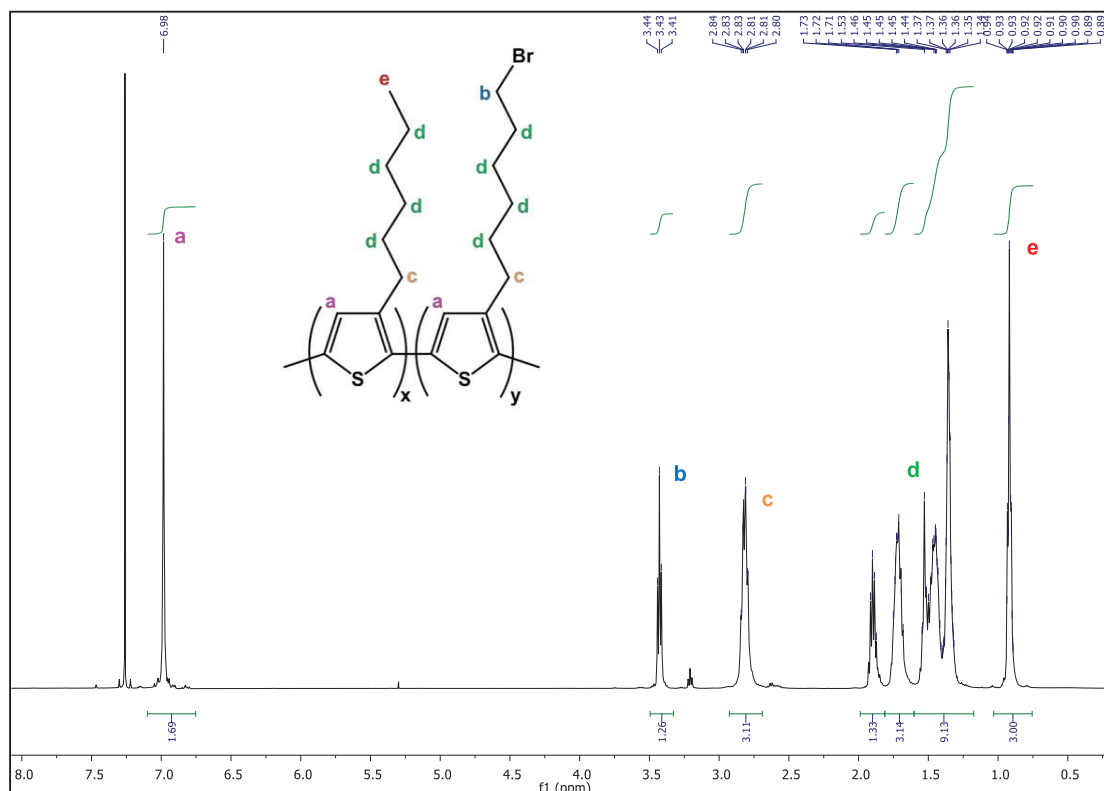
Figure 3.6 1 H NMR spectrum of the P3HT- b -P3HTBr diblock copolymer in CDCl 3 .
