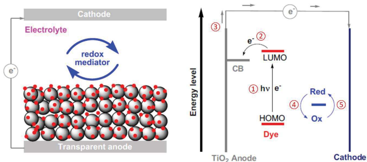
Figure 1.23 Schematic representation (left) and working principle (right) of a dye-sensitized solar cell. After the absorption of a photon (1), dye molecules are promoted to an excited state ( S^0 \rightarrow S^* ), resulting in the electron transfer from the highest occupied molecular orbital (HOMO) to the lowest unoccupied molecular orbital (LUMO). This process is only possible if the incident photons have higher energy than HOMO-LUMO band gap. The dye can thus inject this electron upon oxidation in the conduction band of the metallic oxide on which it is grafted (2). After diffusion into the \text{TiO}_2 layer, the electron is collected by the external circuit via the transparent and conductive electrode: the photoanode (3). The electron transfer into the oxide is governed by diffusion and trapping/entrapping at the grain boundaries and defects. The oxidized dye, i.e. S^+ , is then reduced by the redox couple in the electrolyte to refund its fundamental state, i.e. S^0 (4). The reduced form of the redox couple is regenerated at the counter-electrode that gives one electron from the external circuit (5). In summary, there is no consumption or formation of species under working, i.e. the electrons are the only one to move in the cell under illumination affording a photocurrent.
