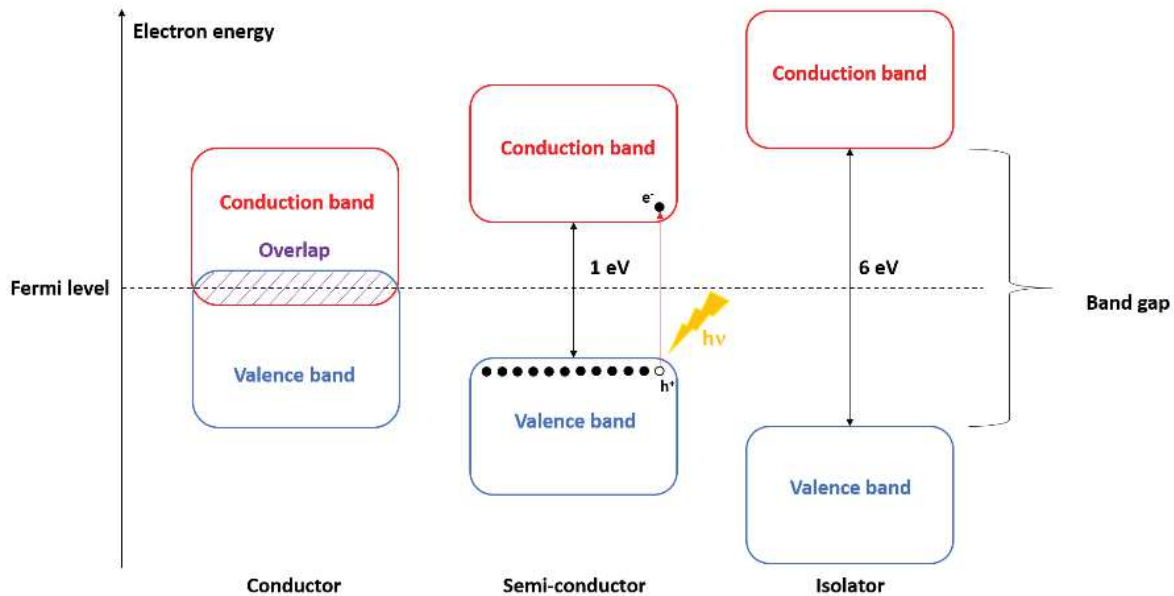
Figure 1.2 Schematic representations of a conductor, a semiconductor and an insulator.
