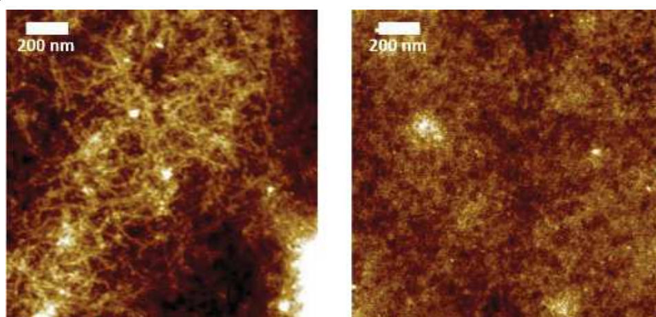
Figure 2.13 TM-AFM height images ( 2.0 \times 2.0 \mu\text{m}^2 ) of thin films of PTIm-1Zn (left) and PTIm-2Zn (right) drop-cast from xylene solutions ( C \sim 0.2 \text{ mg}\cdot\text{mL}^{-1} ).
