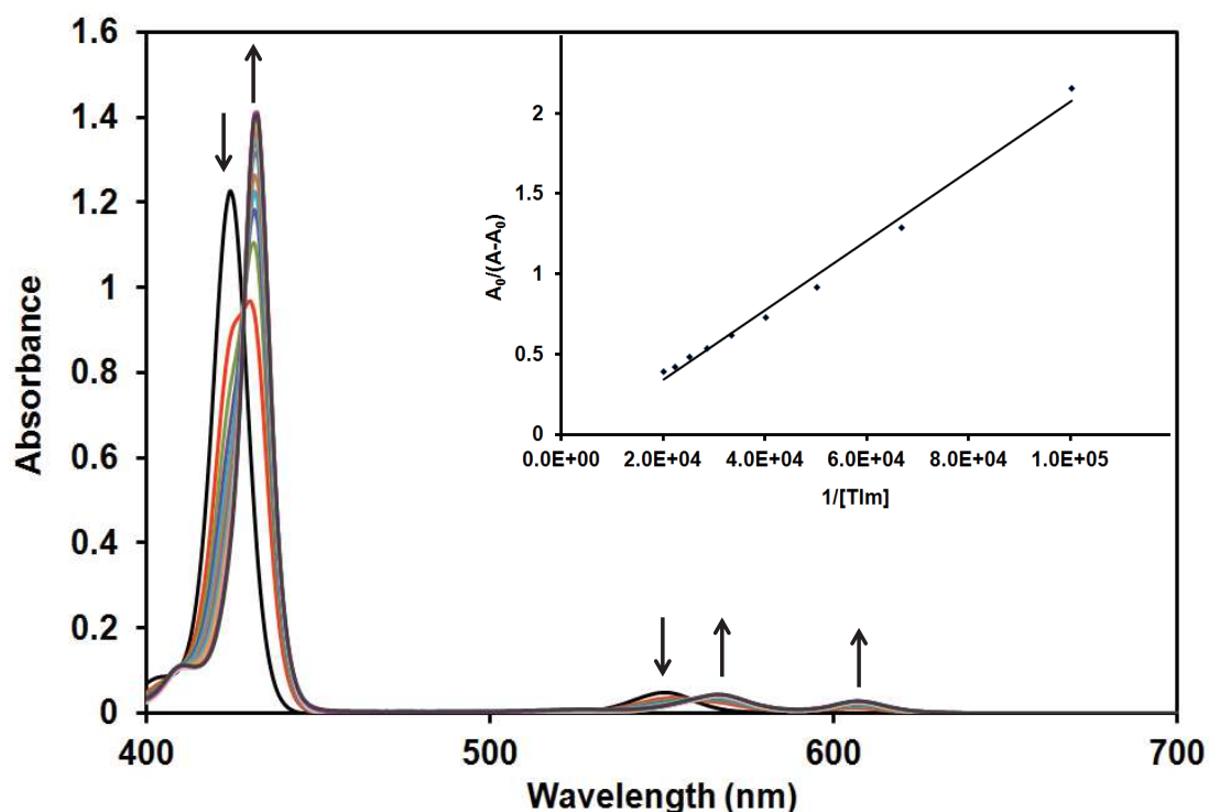
Figure 2.6 UV-vis absorption spectra of 1Zn after successive addition of T1m and determination of the association constant for the complex T1m-1Zn using Benesi-Hildebrand plot (inset) in toluene.
