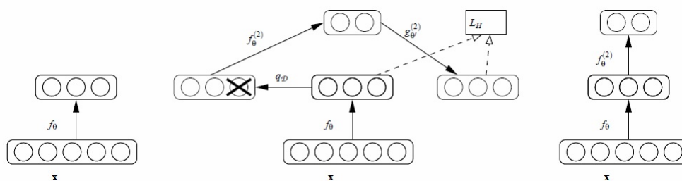
Figure 4.7: Stacked Denoising Auto-encoder. After training a first level denoising autoencoder (Fig. 4.6) its learnt encoding function f_\theta is used on clean input (left). The resulting representation is used to train a second level denoising autoencoder (middle) to learn a second level encoding function f_\theta^{(2)} . From there, the procedure can be repeated (right) [159].
