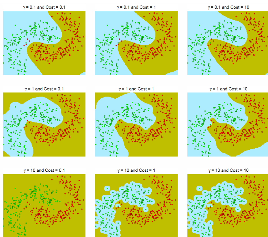
Figure B.5: Decision boundaries for a banana shaped dataset generated by SVM with a RBF kernel for different C and \gamma values.
