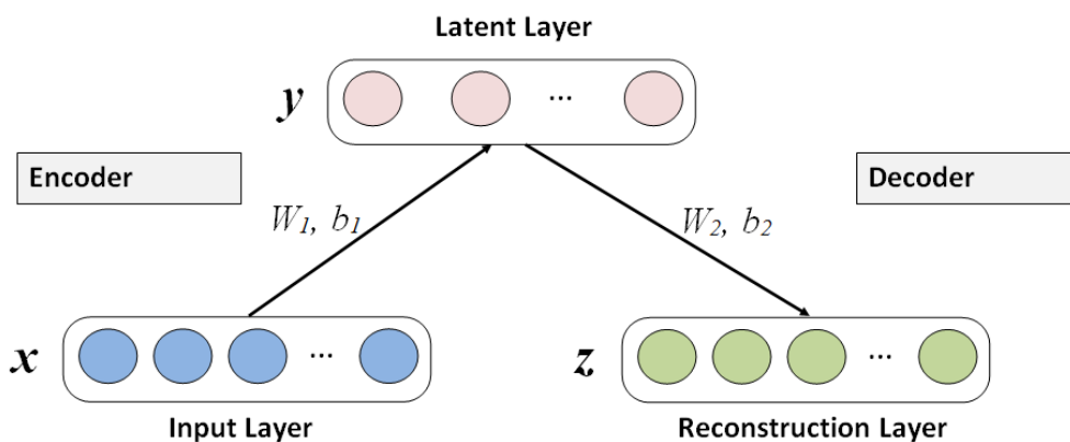
Figure 4.4: Auto-Encoder.
