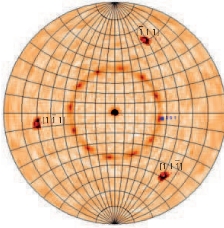
FIGURE 2.20: Schematic of a pole figure measurement.
