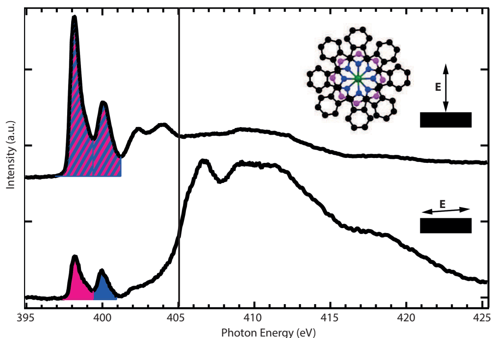
FIGURE 4.4: NEXAFS spectrum of a \sim 1 nm thick LuPc 2 deposited on Au(111). (top) with polarization perpendicular ( 90^\circ ) to the surface (out-of-plane), (bottom) with polarization parallel ( 4^\circ ) to the surface (in-plane). The filling represents the contributions: pyrrolic (blue) and azabridge (purple) N atoms.
