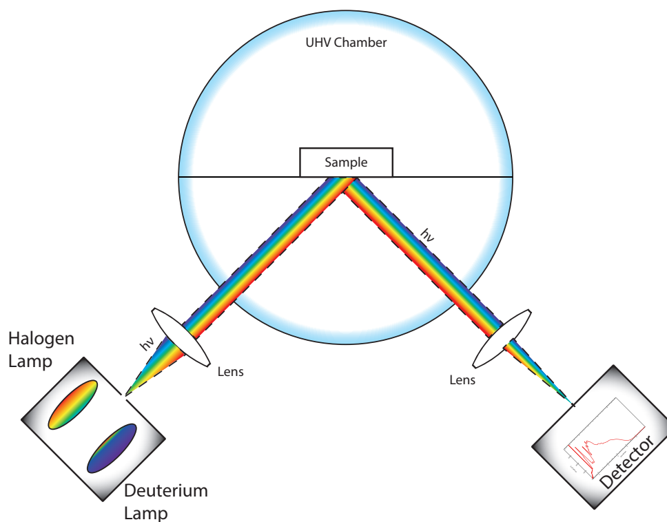
FIGURE 2.14: a) schema depicting the experimental setup used in this work; b) the calculated SDRS spectrum for \text{LuPc}_2 thin film deposited on gold, with the Data relative to a \sim 2 nm thick film obtained experimentally.
