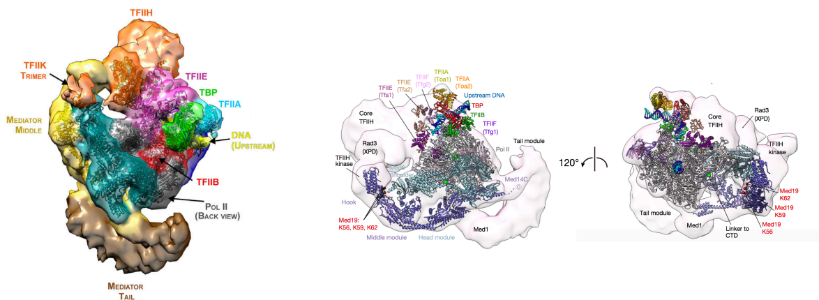
Figure 14 – Structure and model of the PIC-Mediator complex. (Left) A surface representation of the cryo-EM map is shown, where it is possible to identify the interaction between Mediator and components of the PIC. From (Robinson et al. , 2016). (Right) The atomic model of the cPIC–cMed complex obtained by the group of Patrick Cramer (ribbon representation) was placed into the low-resolution cryo-EM map of the PIC–Mediator complex represented on the left. From (Nozawa et al. , 2017).
