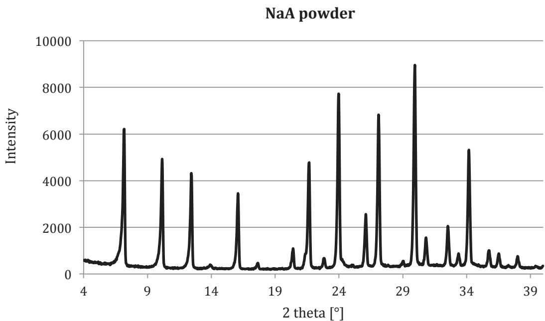
Figure B 3: X-ray diffraction pattern of the NaA powder used for ion exchange.
