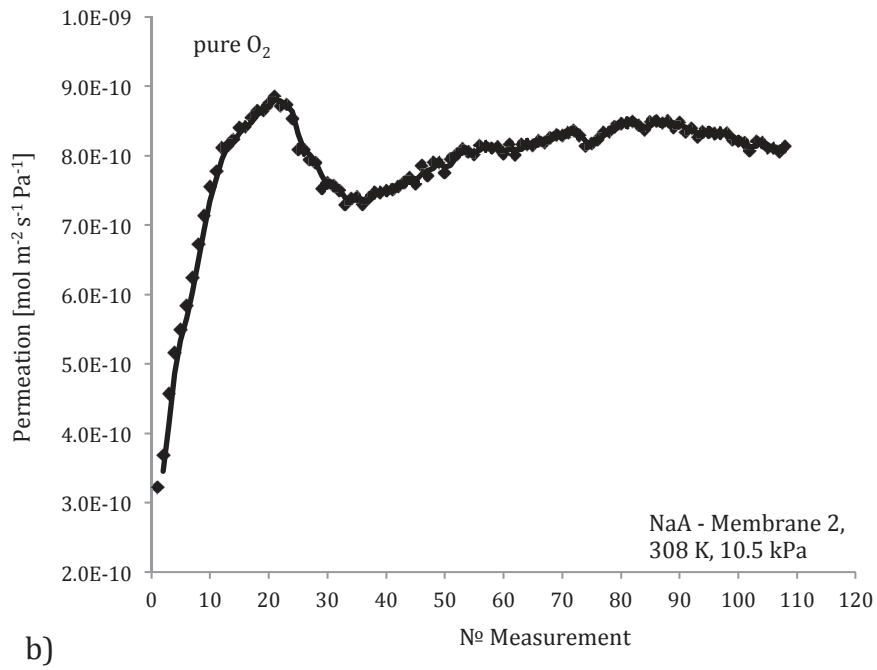
Figure 16: Single gas permeances of a) N_2 and b) O_2 through NaA – Membrane 2 at 308 K and 10.5 kPa pressure drop. The x-axis corresponds to the GC measurements of the permeate composition that were recorded over time with steps between 4 min to 15 min.
