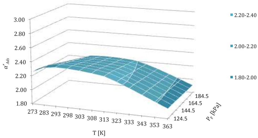
Figure 23: Adsorption selectivity of NaA calculated by a) model (1) and b) model (2) as function of temperature and pressure. Feed pressure is varied, while permeate pressure is constant ( P_p = 124 kPa).
