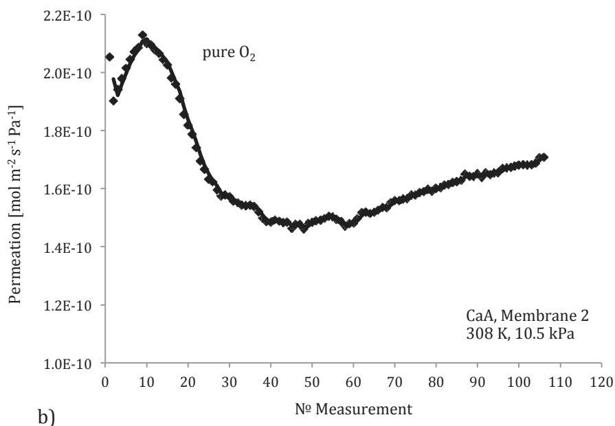
Figure 18: Single gas permeances of a) N_2 and b) O_2 through CaA – Membrane 2 at 308 K and 10.5 kPa pressure drop. The x-axis corresponds to the GC measurements of the permeate composition that were recorded over time with steps between 4 min to 15 min.
