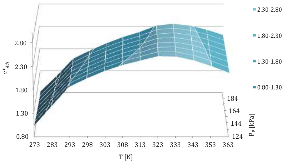
Figure 27: Adsorption selectivity of CaA calculated by a) model (1) and b) model (2) as function of temperature and pressure. Feed pressure is constant ( P_F = 194.5 kPa) and permeate pressure is varied.
