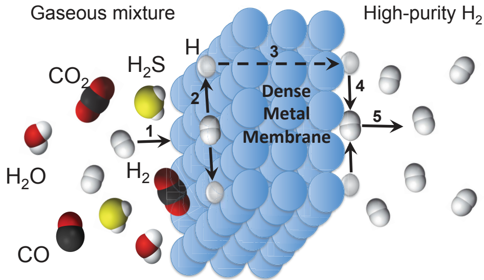
Figure 4: Schematic representation of the multistep H_2 transport mechanism through a dense metal membrane. Step 1: External diffusion; Step 2: Dissociation of H_2 and dissolution of H atoms; Step 3: Internal diffusion; Step 4: Re-association of H atoms and desorption of H_2 ; Step 5: External diffusion.
