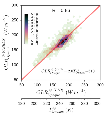
Figure E4. As Fig. E3e but with multilayer cloud considered in the computation of T_{\text{opaque}}^{\circ} , considering that the cloud layers above the optically opaque cloud (below) have an equivalent emissivity \varepsilon_{\text{above}} = 0.3 : T_{\text{opaque}}^{\circ} = (1 - \varepsilon_{\text{above}}) T_{\text{below}}^{\circ} + \varepsilon_{\text{above}} T_{\text{above}}^{\circ} where T_{\text{below}}^{\circ} = \frac{T_{\text{topbelow}}^{\circ} + T_{\text{zopaque}}^{\circ}}{2} and T_{\text{above}}^{\circ} = \frac{T_{\text{topabove}}^{\circ} + T_{\text{baseabove}}^{\circ}}{2} .
