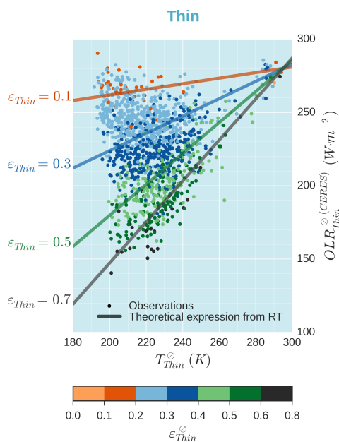
Figure E1. Comparison between observed and lidar-derived OLR, on a CERES footprint scale, as a function of T_{\text{thin}}^{\ominus} and \varepsilon_{\text{thin}}^{\ominus} . Results obtained from CERES (dots) and CALIOP (lines) collocated measurements. Theoretical expressions are from Eq. (4). Same results as in Fig. 6b but only for measurements where \text{OLR}_{\text{clear}}^{\ominus} is close to 280 \text{ W m}^{-2} selected ( \text{OLR}_{\text{clear}}^{\ominus} \in [275\text{--}285] \text{ W m}^{-2} ), in order to only see the contribution of T_{\text{thin}}^{\ominus} and \varepsilon_{\text{thin}}^{\ominus} on the OLR. Only nighttime conditions over ice-free oceans for January 2008 are considered.
