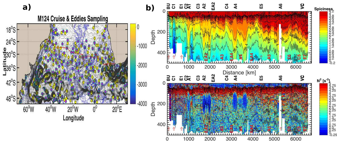
Figure 5.2: (a) Track of the 124 Cruise carried out in the Southeastern Atlantic between February and March 2016 onboard the German RV Meteor. (b) Vertical sections of spiciness (top) and stratification (bottom) along an Agulhas Ring trajectory in the Cape Basin, as sampled during this oceanographic campaign (Courtesy of Sabrina Speich). The bottom section shows homogenized patches of low stratification at around 200 m deep, indicating the subduction of a local variety of mode waters that we defined as Agulhas Ring Mode Water (ARMW).
