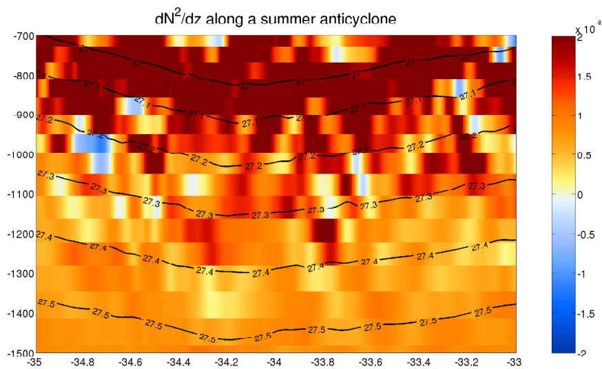
719 Figure 15. Meridional section of the vertical gradient of stratification ( dN^2/dz , [ \text{s}^{-1} ]) plotted at 9.2^\circ\text{E} 720 along a summer anticyclone for the intermediate depths of the water column ( \sim 700 - 1500 m). Black contours 721 are for isopycnals ranging from 27 to 27.5 \text{ kg/m}^3 .
