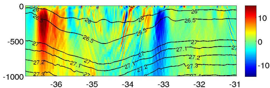
Figure 5.4: Instantaneous sections of potential vorticity (top) and vertical velocity (bottom), along a summer anticyclone crossing the domain of our nested configuration (AGU12_36_108).
