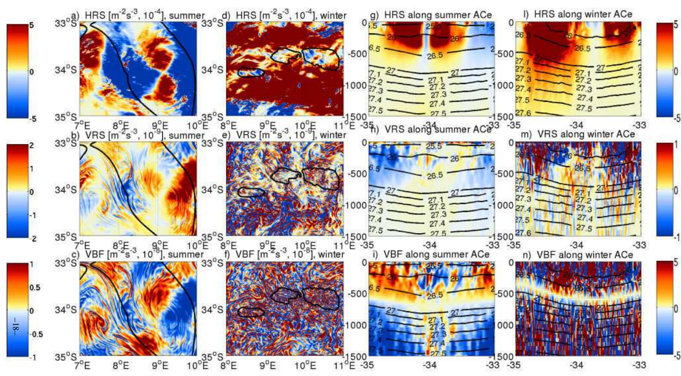
431 Figure 6. Left panel: Snapshots of horizontal and vertical shear (HRS and VRS, [m^{-2}s^{-3}] ) and vertical buoyancy flux (VBF, [m^{-2}s^{-3}] ) plotted along an ACe detected within the HR 432 simulation in summer (on the left) and winter (on the right). Black contours define the outer limits of the detected eddy. Right panel: meridional sections of the same metrics, extracted 433 at 9.2^{\circ}E with black contours for isopycnals ranging from 26 to 28 \text{ kg/m}^3 . Note that the maps of the left panel (a-f) share the colorbars on the left, while the ones on the right are for the 434 sections of the right panel (g-n).
