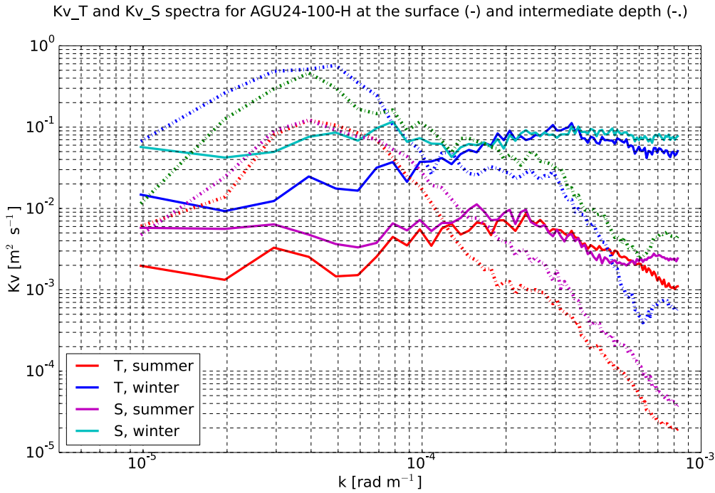
610 Figure 11. Horizontal spectra of the diffusion coefficients of temperature and salinity, computed for 611 AGU24.100.H at the surface (continuous line) and at intermediate depth (dashed) in summer and winter.
