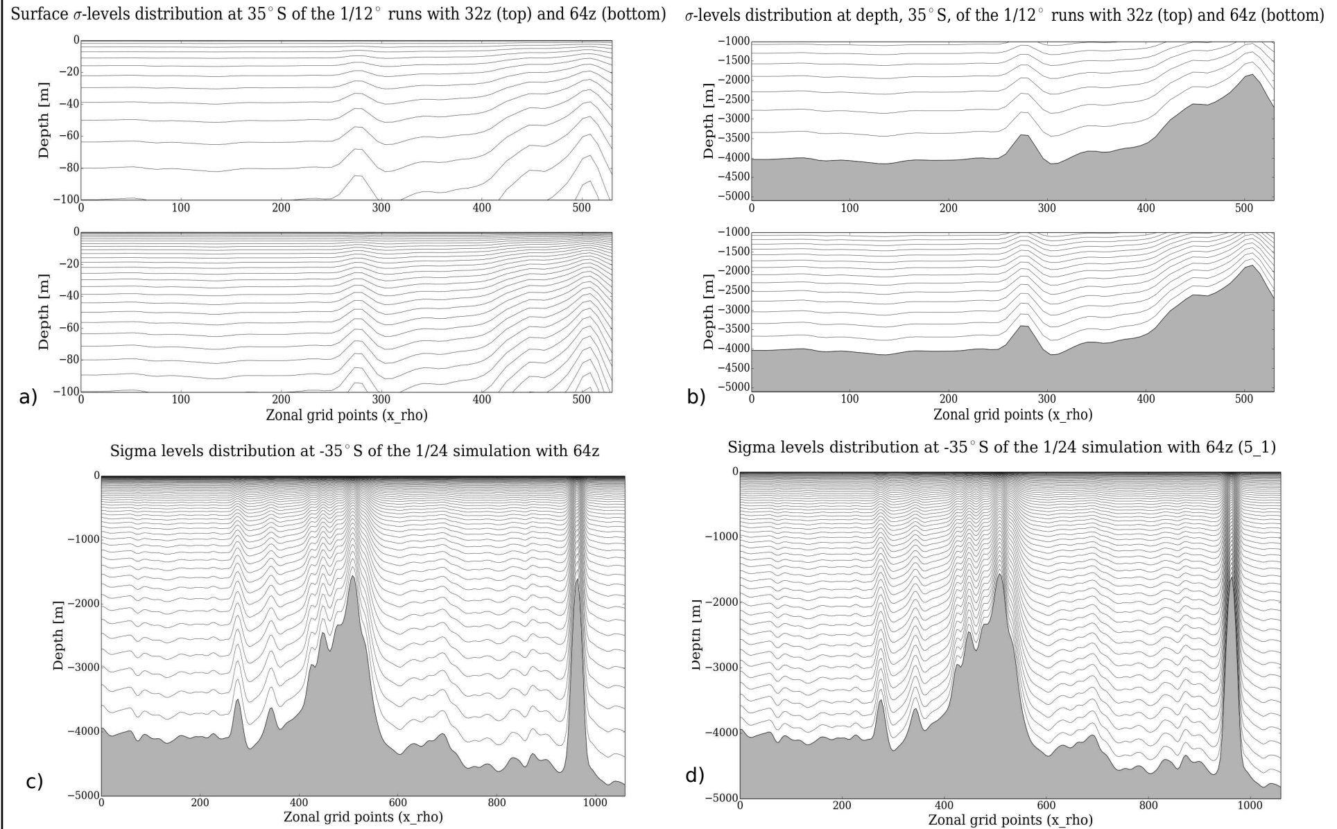
Figure 3.2: Sections showing the differences in the vertical distribution of the sigma levels between the simulations with 32z and 64z in the upper layers (a) and at depth (b), and between the ones having values of Theta-S and Theta-B at 6 and 0 (c) and those having them at 5 and 1 (d).
