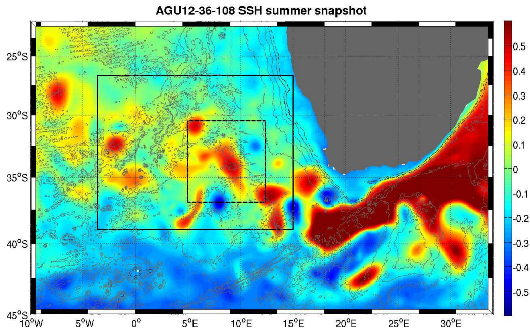
Figure 3.4: Same as Figure 3.1 but for the nested configuration (AGU12_36_108), showing as well the geographical extensions of the three domains of this simulation.
