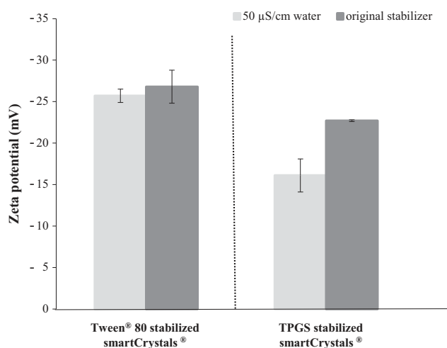
Fig. 4. Zeta potential of quercetin nanosuspensions. Zeta potential of quercetin nanosuspensions with Tween® 80 and TPGS produced by bead milling for 5 min followed by 2 cycles of high pressure homogenization at 300 bar. Reacting media 50 µS/cm water and original stabilizer solution.
