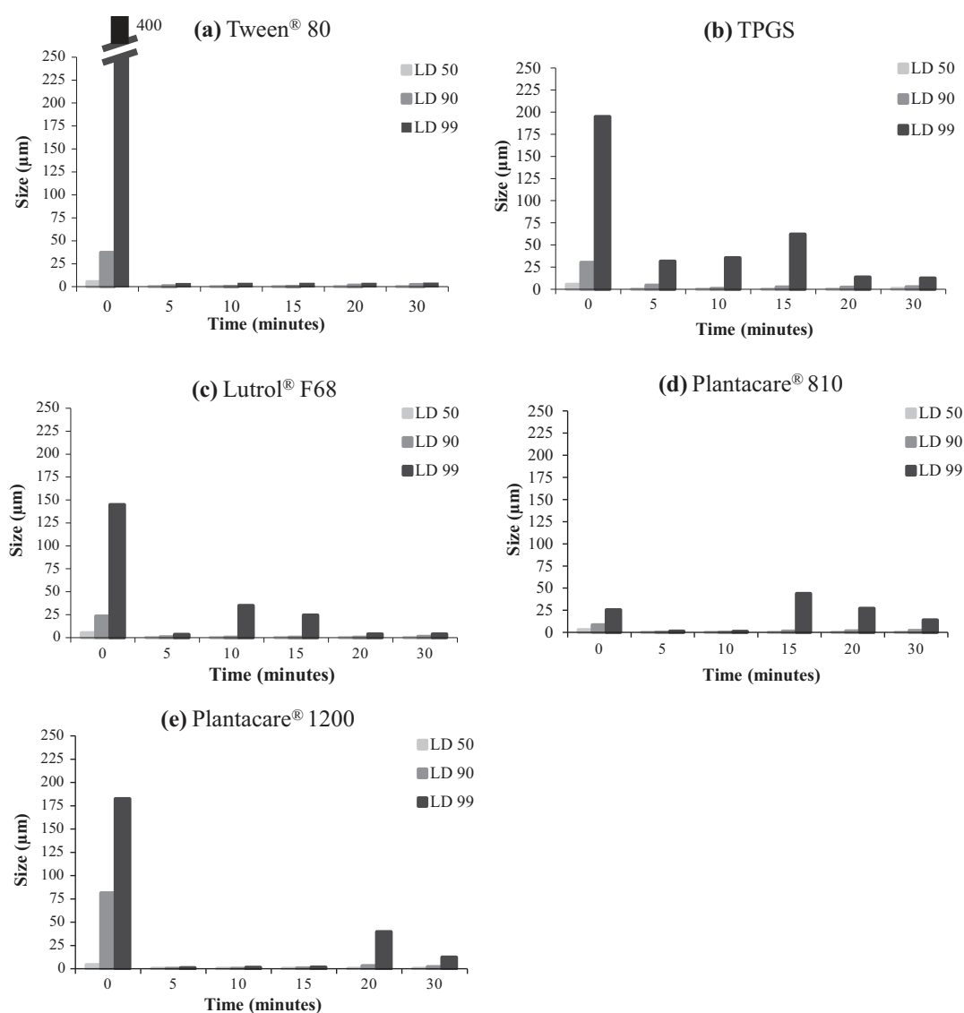
Fig. 2. Quercetin suspension size distribution evaluation using LD. LD size distribution as a function of milling time in the bead mill of suspensions stabilized with (a) Tween ® 80, (b) TPGS, (c) Lutrol ® F68, (d) Plantacare ® 810 and (e) Plantacare ® 1200.
