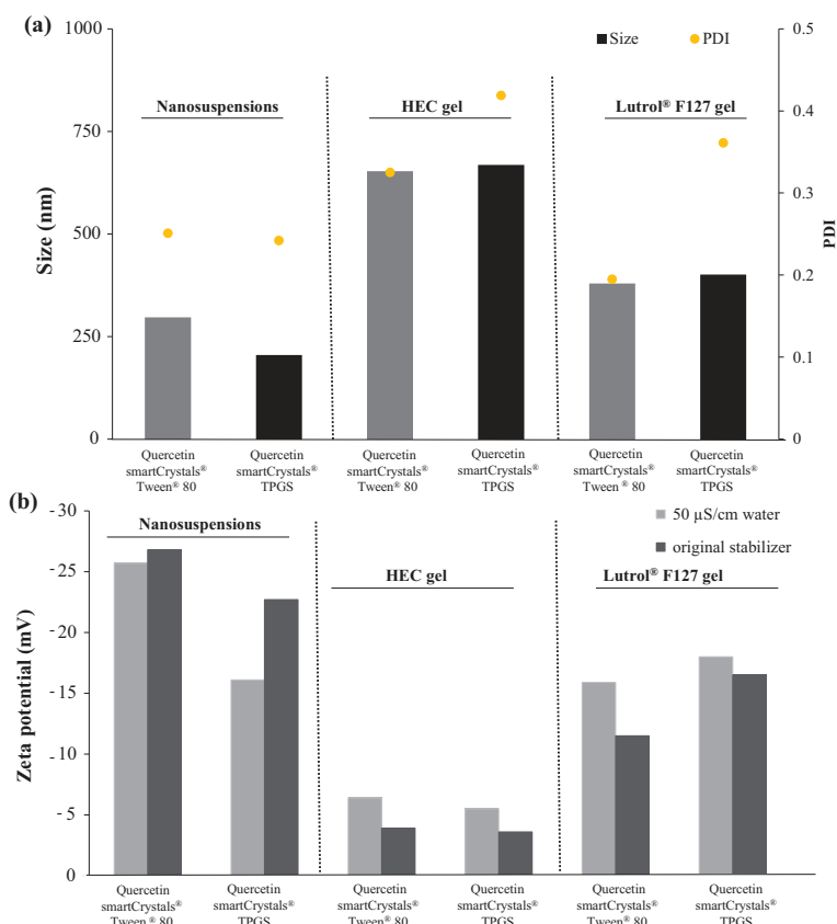
Fig. 9. Quercetin smartCrystals® associated with nonionic gels results PCS. Quercetin smartCrystals® formulated into HEC 1.7 w/w% gel and Lutrol® F127 16.7 w/w% gel, (a) average particles size and polydispersity index (PDI), (b) Zeta potential (absolute value).
