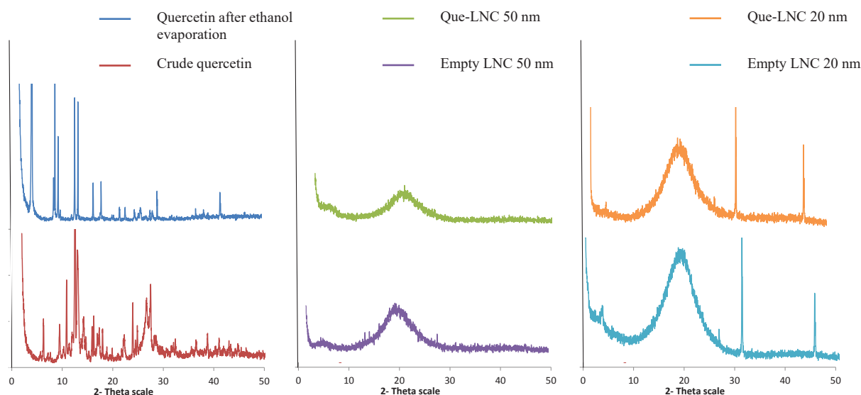
Fig. 3: X-ray diffractograms for crude quercetin (left), quercetin LNC 50 nm (middle) and quercetin LNC 20 nm (right).
