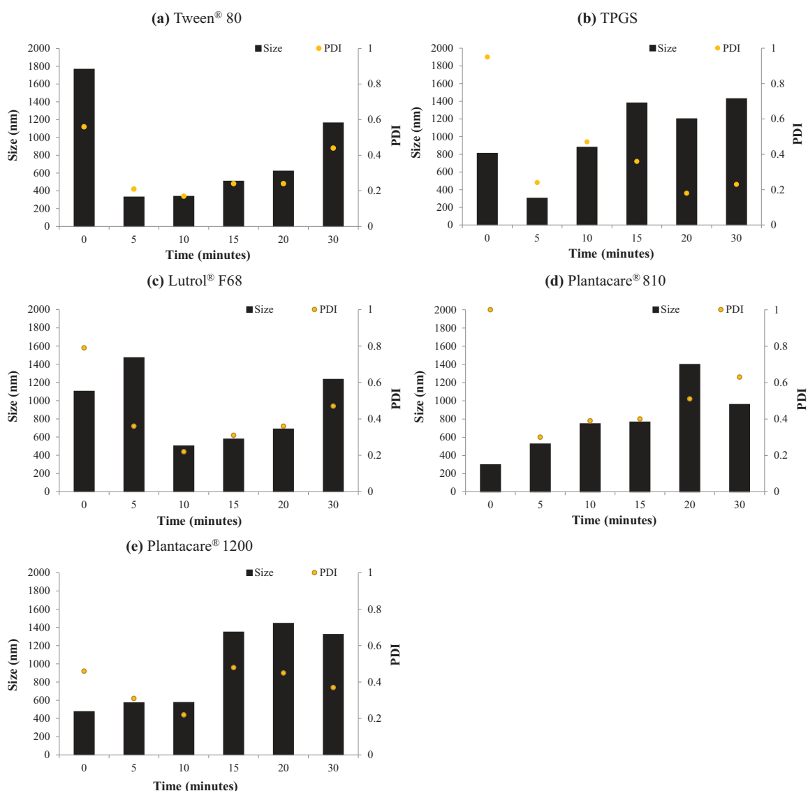
Fig. 1. Quercetin suspension size and PDI evaluation using PCS. PCS size and polydispersity index (PDI) as a function of milling time in the bead mill of suspensions stabilized with (a) Tween® 80, (b) TPGS, (c) Lutrol® F68, (d) Plantacare® 810 and (e) Plantacare® 1200.
