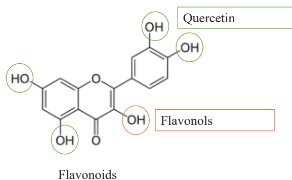
Fig. 1: Chemical structure of flavonoids, flavonols (orange) and quercetin (green).
