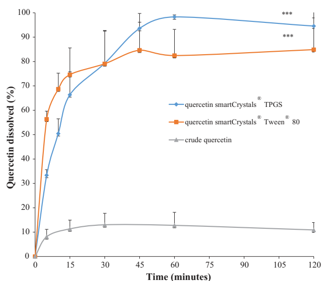
Fig. 7. Dissolution profiles of crude quercetin/quercetin smartCrystals ® nanosuspensions stabilized with Tween ® 80 and TPGS. Quercetin dissolved percentage normalized to total quercetin quantity \pm SD ( n = 3 ), t -test and Kolmogorov–Smirnov test showed significant difference between crude quercetin and quercetin smartCrystals ® , * = P < 0.05 , ** = P < 0.01 and *** = P < 0.005 .
