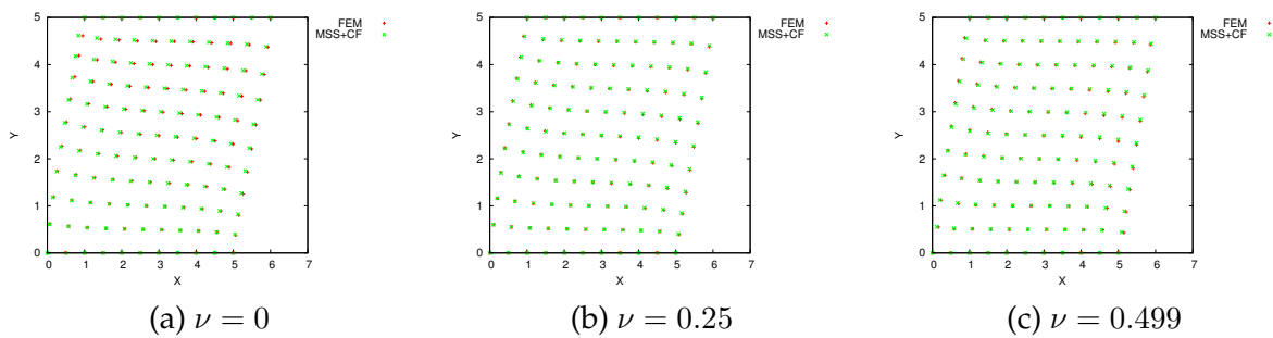
FIGURE 5.11: Alignment of cross-sectional view on points in a shearing experiment with big (20 %) deformation at different Poisson's ratios, E = 10,000 ; comparison between MSS-CF and FEM.
