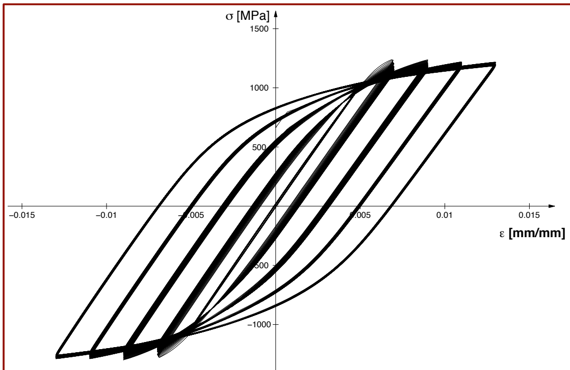
Figure 2.5: Multi-level cyclic test performed at R_\epsilon = -1 in the LMT lab
