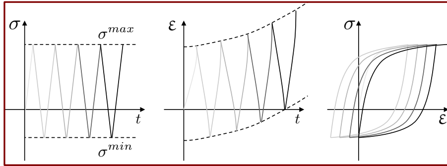
Figure 1.7: Ratcheting principle
