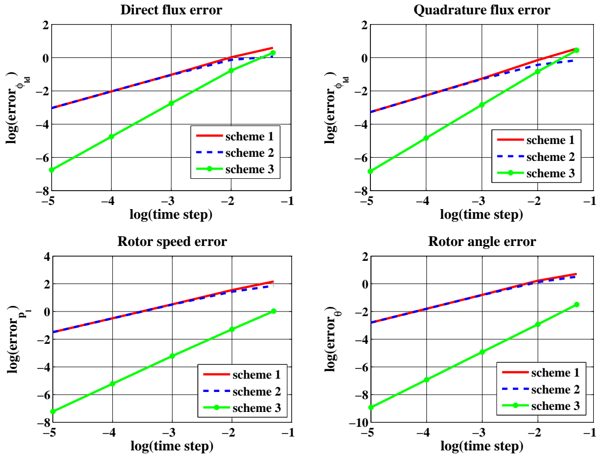
Figure 3.3.1: The state variable errors of the energy-preserving discretization schemes for the electro-mechanical elevator.
