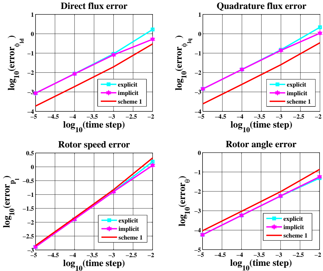
Figure 3.3.4: The state errors of the electro-mechanical elevator by using the explicit Euler (ex), implicit Euler (im), energy-preserving (st) methods.
