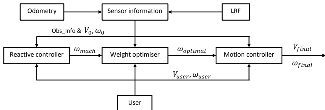
FIGURE 2.4: The Qinan Li et al. (2011)'s architecture of the dynamic shared control
