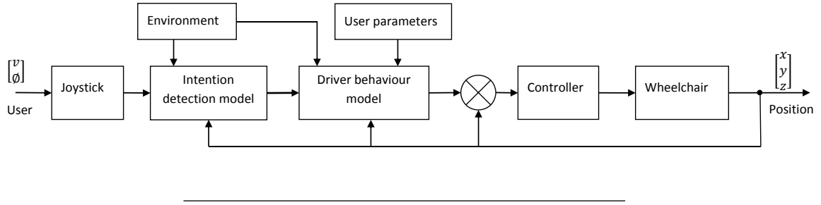
FIGURE 5.1: The control diagram of a wheelchair with integrated driver behaviour model and intention detection model.
