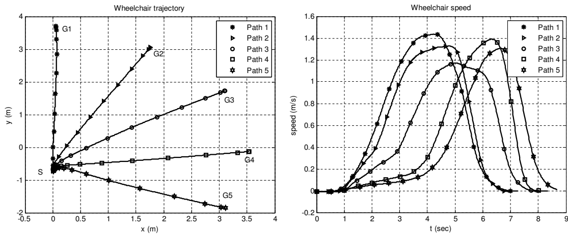
FIGURE 4.5: Wheelchair trajectories and speeds observed in a risk free environment.
