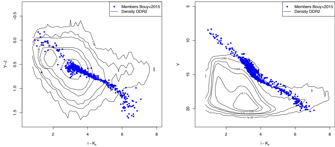
Figure 2.15: Candidate members of Bouy et al. (2015), blue dots, together with the density of the Restricted Pleiades DANCe Data Release 2 (RDDR2) data set, black contours, in the colour-colour diagram Y - J vs. i - K_s (left) and CMD Y vs i - K_s (right).
