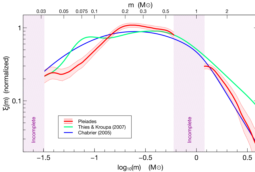
Figure 2.11: Pleiades present day mass distribution from Bouy et al. (2015) (red). IMF’s from Chabrier (2005) (blue) and Thies & Kroupa (2007) (green) are also shown. Reproduced from Figure 9 of Bouy et al. (2015), The Seven Sisters DANCe. I. Empirical isochrones, luminosity, and mass functions of the Pleiades cluster , A&A, Vol. 577.
