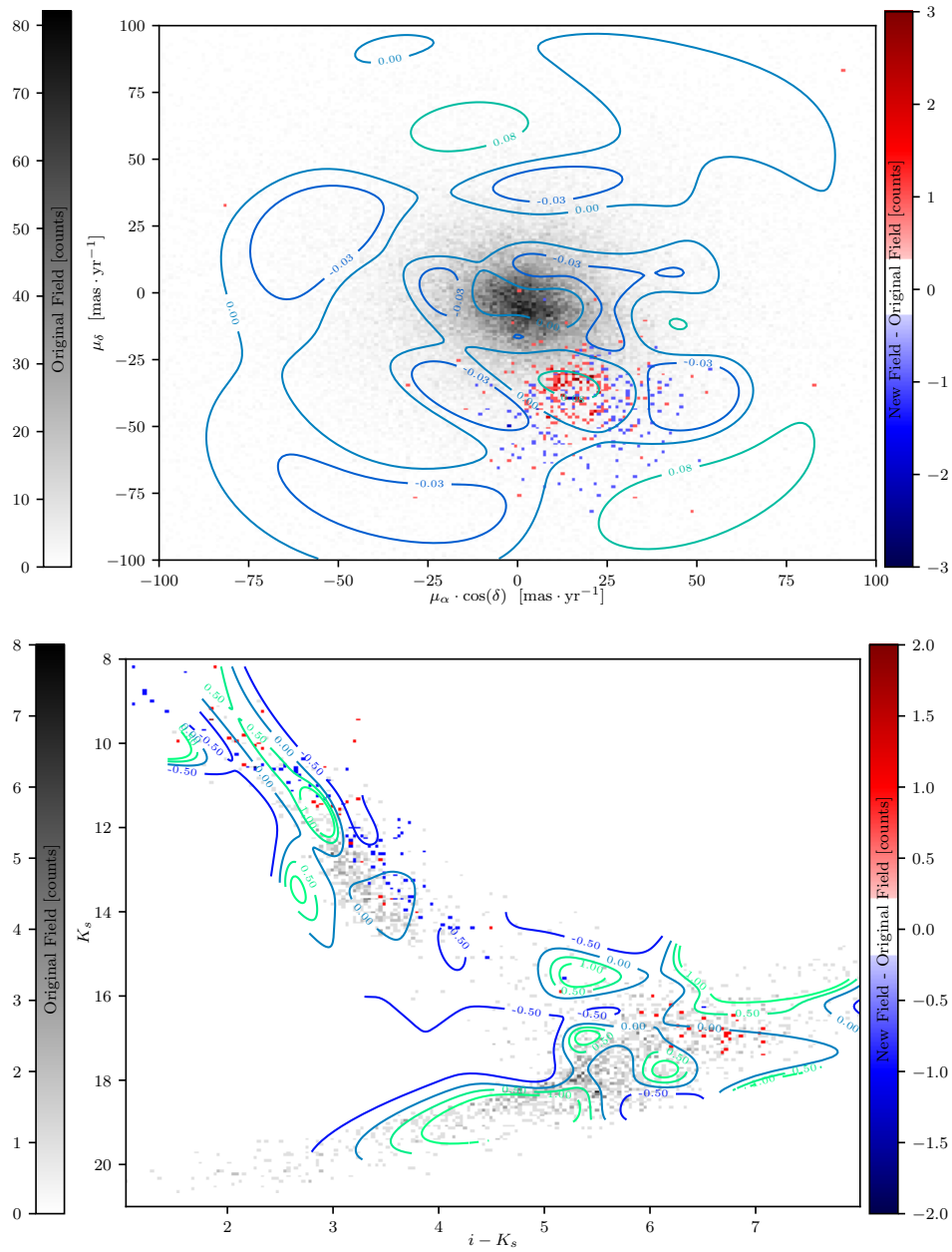
Figure 4.35: Proper motions and K_s vs i - K_s CMD showing: the absolute difference between the Original field (grey scale) and the New field (blue and red scale), and the absolute relative difference in the densities resulting from the New and Original field models.
