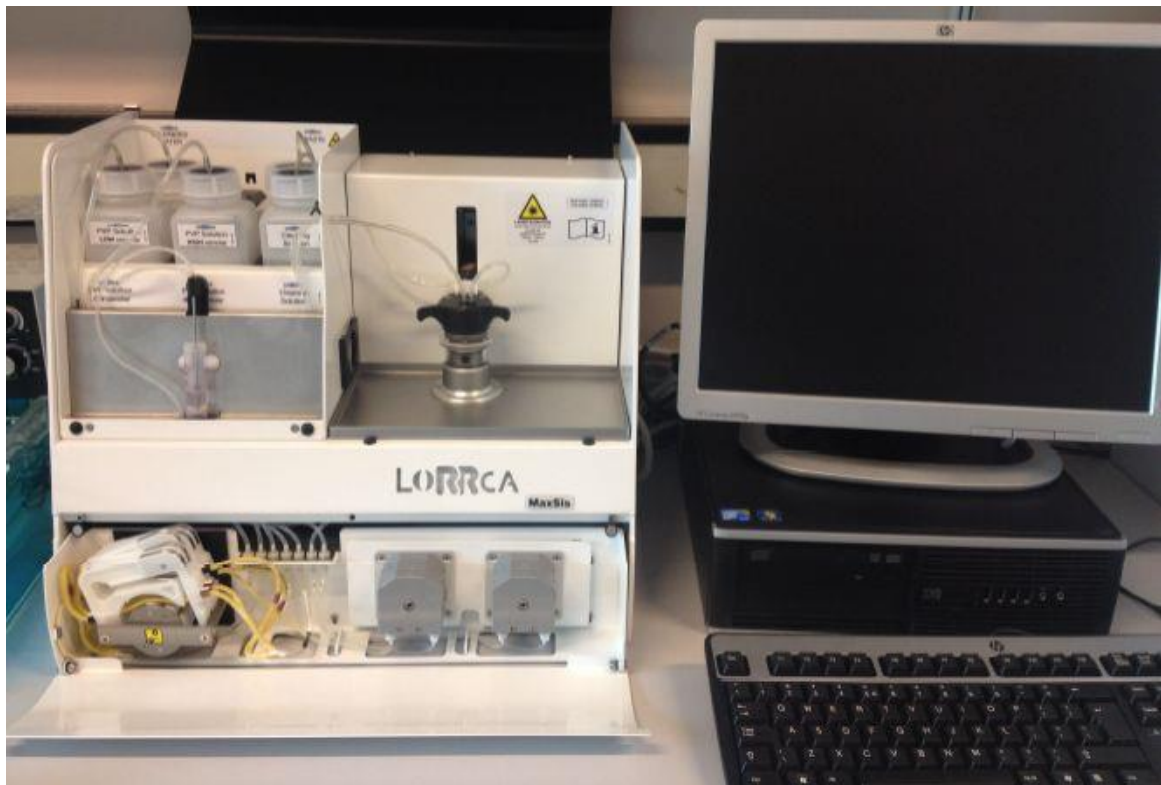
Figure 20 : The LORRCA MAXSIS Ektacytometer. From (Lazarova, www document)
