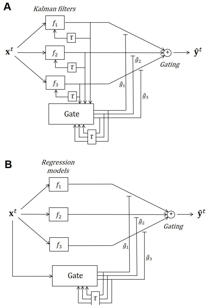
Figure 5.3: SKF ( A ) and MSLM ( B ) data flow. A . The weights used to combine the KF experts depend on the adequacy of each KF with the current and past observed neural signals. B . The weights used to combine the linear experts directly depend on the value of current and past observed neural signals.
