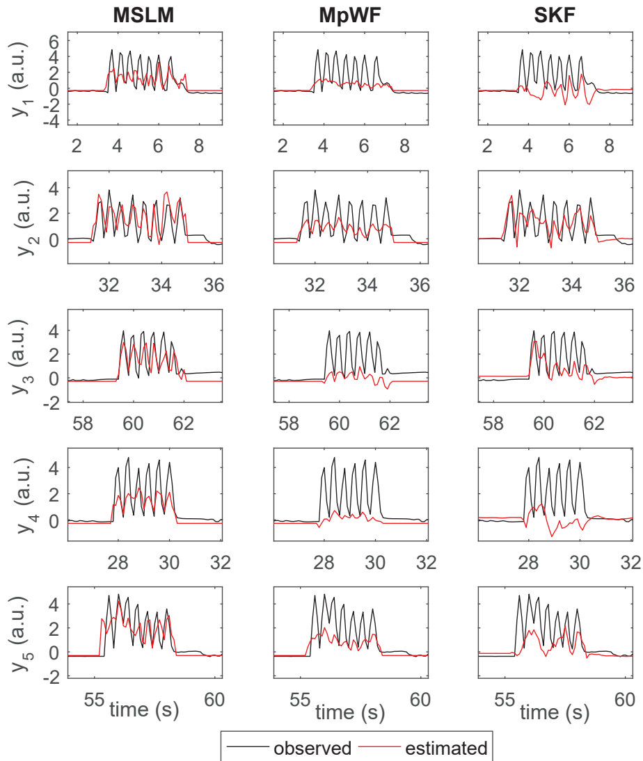
Figure 7.7: Clinical data set, known state sequence, focus on the IC states. Example of observed and estimated finger trajectories (subject zt). The tracked finger positions are indicated in solid black lines. Red trajectories represent the estimates yielded by the MSLM, MpWF and SKF decoders. "a.u." refers to "arbitrary unit".
