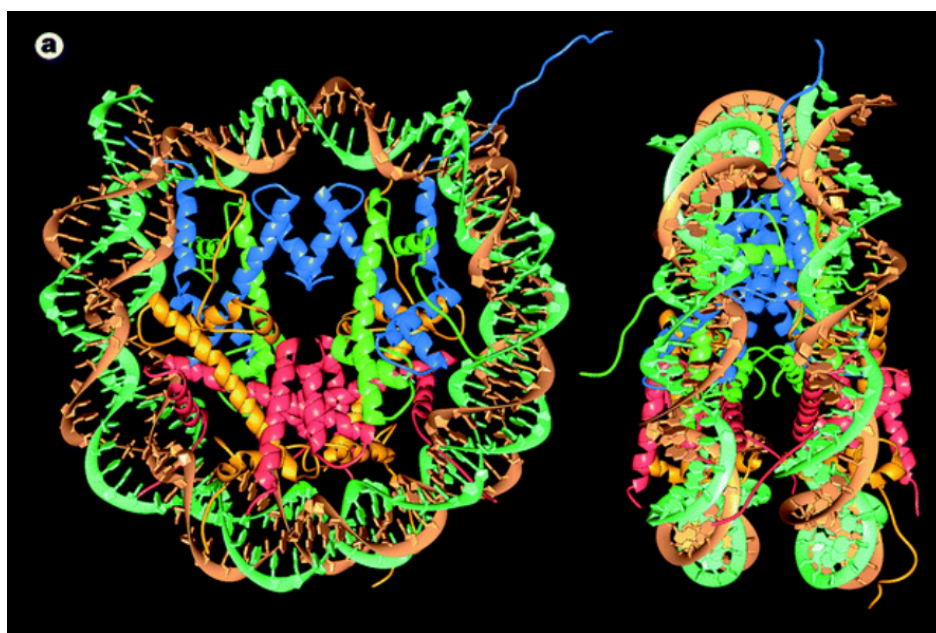
Figure 5: Nucleosome core particle (from Luger et al., 1997)
