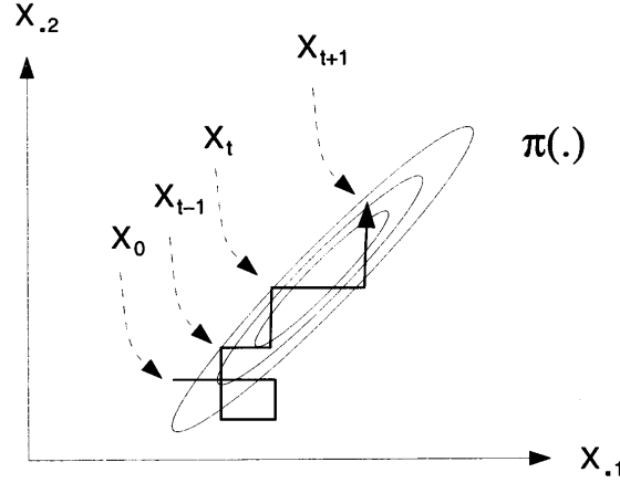
Figure 2.4: Illustration of the single-site updating Metropolis-Hastings MCMC (taken from [Gilks et al. , 1996]).
