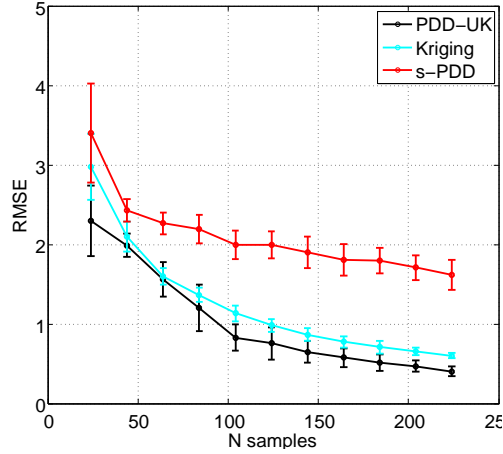
Figure 3.4: TEST 2: Mean RMSE convergence comparison between Ordinary Kriging, sparse PDD and coupled PDD-UK metamodelling, m = 5 , \varepsilon_{Q^2} = 10^{-8}
