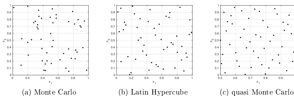
Figure 2.3: Plots of 50 samples drawn from a uniformly-distributed two-dimensional stochastic vector with Monte Carlo and Latin Hypercubes and quasi Monte Carlo sampling methods.
