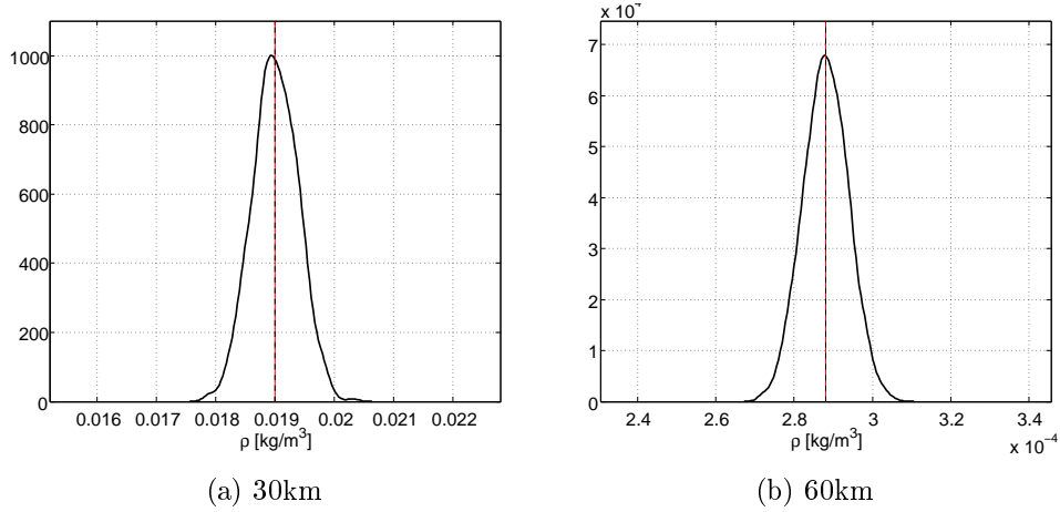
Figure 6.7: PDFs of the density rebuilt from stagnation pressure measurements (solid black line). The dashed line represents the posterior mean value and the red line the reference value. The x axis width shows the uniform prior interval.
