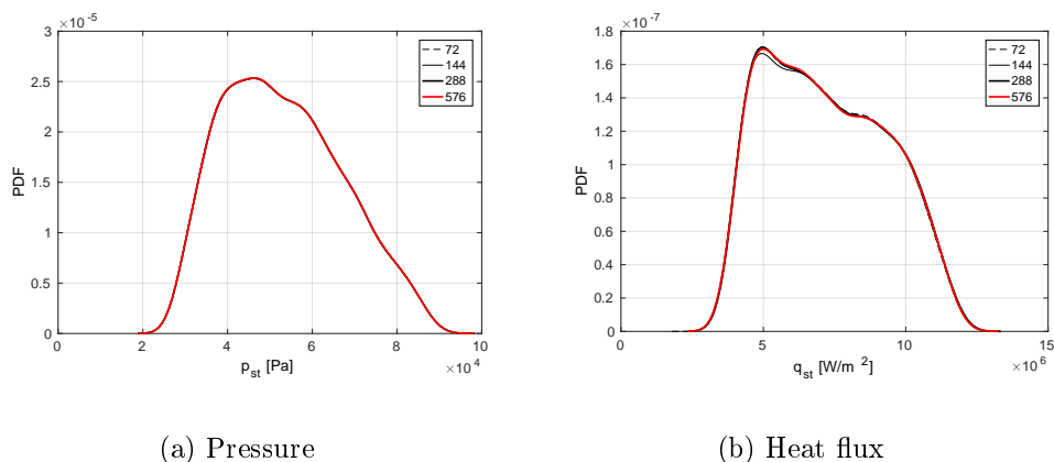
Figure 3.8: Kernel density estimates of the probability density functions of stagnation pressure and heat flux computed on the MC sample propagated through PDD-UK metamodels. Comparisons are proposed for results obtained with different surrogates trained on experimental design of increasing size.
