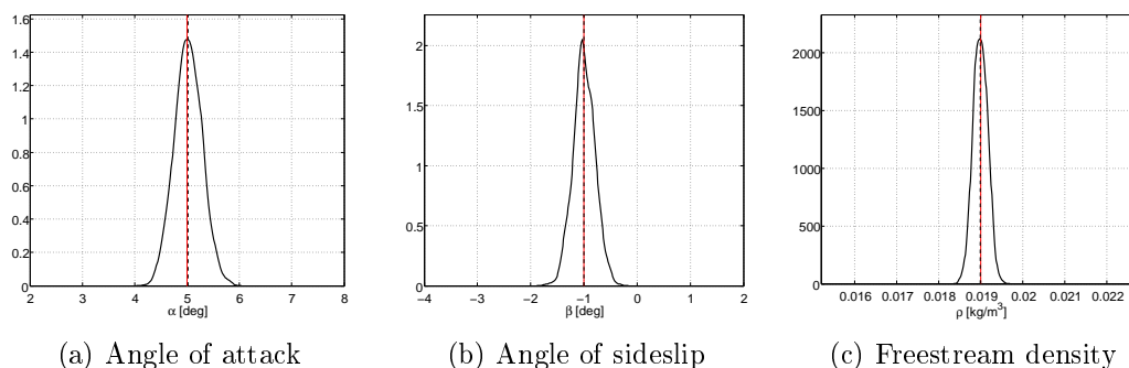
Figure 6.10: PDFs of the freestream density and flow angles rebuilt from wall pressure measurements (solid black line) for the 30km trajectory points. The dashed line represents the posterior mean value and the red line the reference value. The x axis width shows the uniform prior interval.
