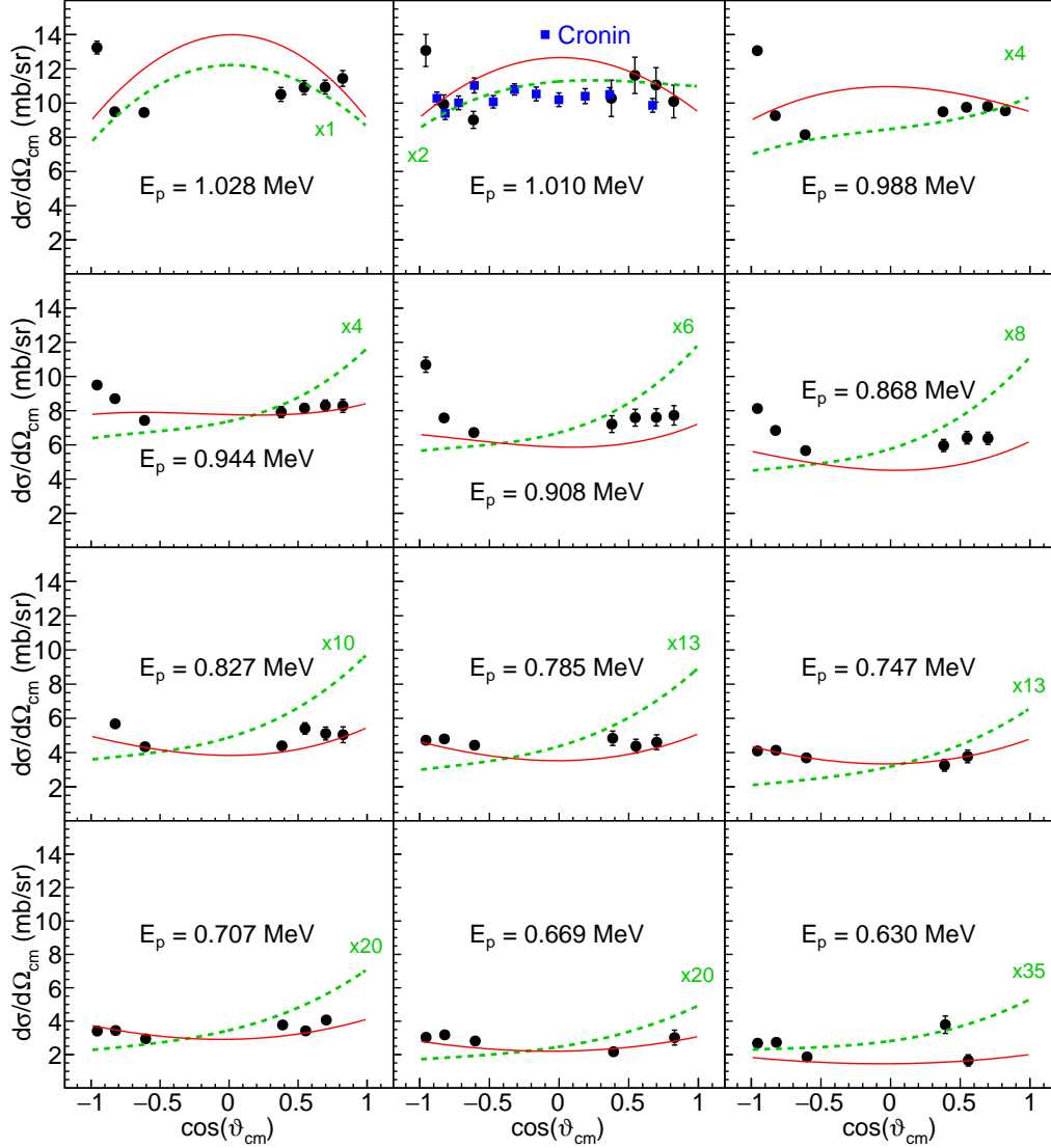
Figure 2.11: Angular distributions of the ^{10}\text{B}(p, \alpha_0)^7\text{Be} reaction, as a function of the proton energy. Vertical bars represents statistical errors. Blue squares report angular distribution data obtained by Cronin [218] at 1 MeV. Green dashed lines: R -matrix calculations of angular distributions obtained by using the resonance parameters reported in the literature [202, 212, 213, 215, 232]. The absolute cross section scales have been multiplied by the scaling factors indicated in the figure for ease of display. Red solid lines: R -matrix calculations of angular distributions (mb/sr) obtained by using parameters reported in Table 2.2, columns 3-10, that have been derived from the data fit procedure described in paragraph 2.2.3.
