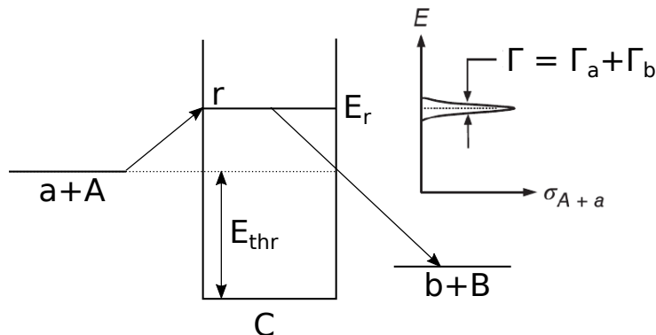
Figure 1.32: Level scheme of a compound nucleus reaction of the type a + A \longrightarrow C^* \longrightarrow b + B . The resonance r is populated at an excitation energy E_r . The behaviour of the cross section for the isolated resonance is qualitatively shown in the right part. The width \Gamma of the level is the Full Width at Half Maximum (FWHM) of the resonance in the cross section as a function of the energy and it corresponds to the sum of all the partial widths which contribute to the decay of the state \Gamma = \Gamma_a + \Gamma_b .
