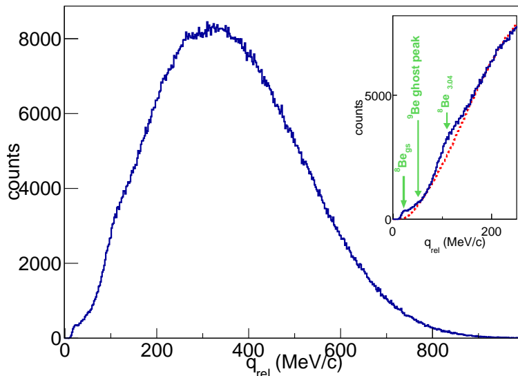
Figure 3.9: Experimental two- \alpha coincidence yield, as a function of the relative momentum, for ^{36}\text{Ar} + ^{58}\text{Ni} collisions at 74 AMeV obtained for central events with the INDRA 4\pi multi-detector. The insert shows a zoom of the low relative momentum part of the spectrum. Here the red line is the evaluated non-correlated background estimated via our event-mixing procedure. Arrows and labels indicate the position of expected peaks.
