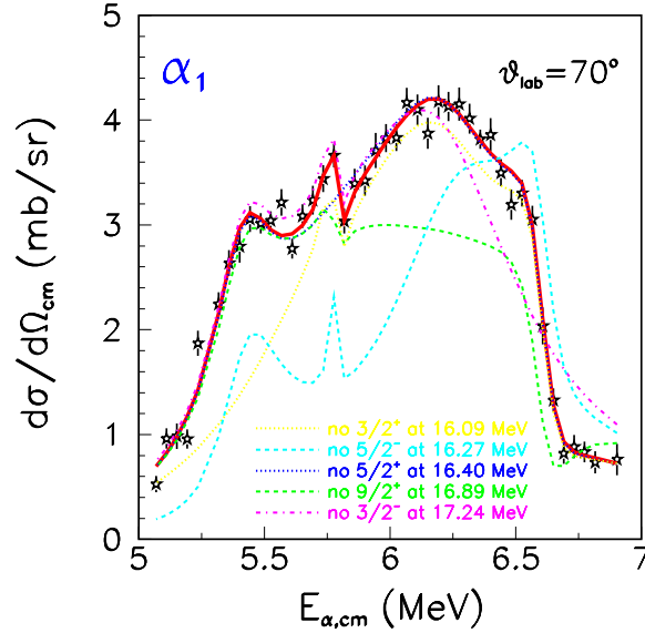
Figure 2.25: ^9\text{Be}(\alpha, \alpha_1)^9\text{Be}_{1.68} DCS data at \theta_{lab} = 70^\circ . The red line represents the R -matrix best-fit on the whole data set here investigated. The dotted yellow line is the R -matrix best-fit without the inclusion of the 3/2^+ state at 16.09 MeV. The dashed azure line is the R -matrix best-fit without the inclusion of the 5/2^- state at 16.27 MeV. The dotted blue line is the R -matrix best-fit without the inclusion of the 5/2^+ state at 16.40 MeV, responsible of the wing at E_{cm} \simeq 5.8 MeV. The dashed green line is the R -matrix best-fit without the inclusion of the 9/2^+ state at 16.89 MeV. Finally, the dash-dotted magenta line is the R -matrix best-fit without the inclusion of the 3/2^- state at 17.24 MeV.
