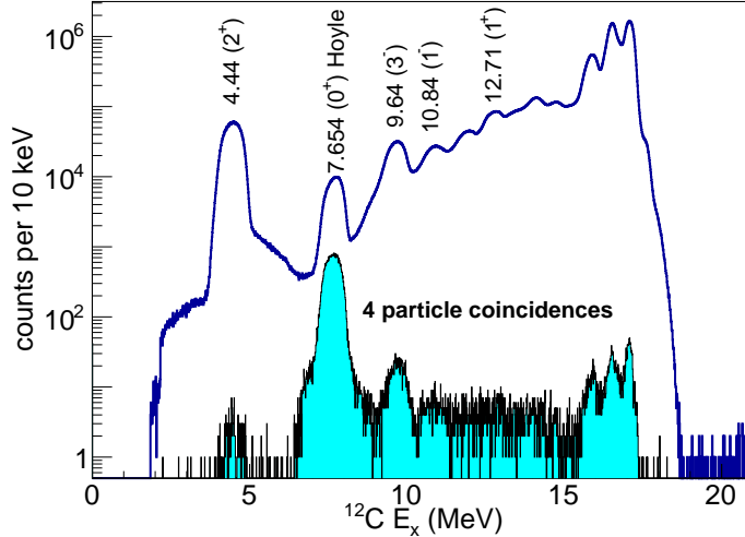
Figure 2.15: ^{12}\text{C} excitation energy spectrum reconstructed from the measured momentum of particles detected by the \Delta E - E anti-coincidence telescope (blue line). Labels are used to indicate the energy and spins of well-known states of ^{12}\text{C} . (filled histogram) Same spectrum obtained by selecting 4-particles coincidences.
