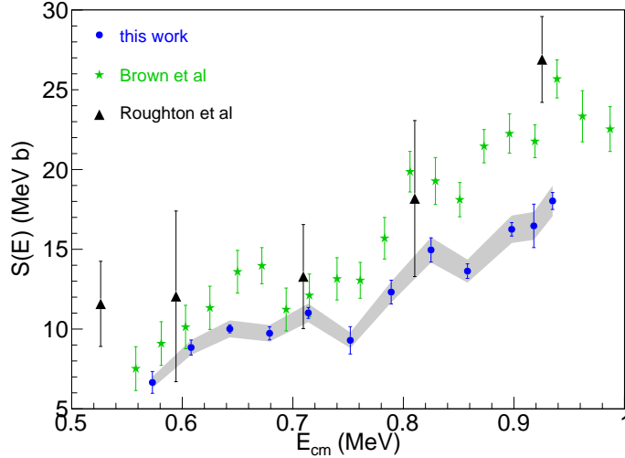
Figure 2.12: ^{10}\text{B}(p,\alpha_0)^7\text{Be} astrophysical S -factor. Blue dots: present data (vertical bars: statistical errors; grey band: non-statistical errors). Green stars: data by Brown et al [225] as reported in [109, 224]. Black triangles: data by Roughton et al [223] as reported in NACRE [109] and NACRE2 [224].
