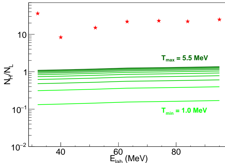
Figure 3.14: Experimental \alpha - \alpha yield ratios ( N_H/N_L ) as a function of the incident energy compared with the results of the pure thermal model. The experimental points are represented by red stars while in different tonality of green we show the present theoretical predictions for medium-temperatures in the range 1.0 \text{ MeV} \leq T \leq 5.5 \text{ MeV} .
