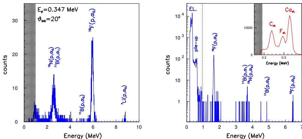
Figure 2.29: (Left panel) Experimental spectrum at \theta_{lab} = 20^\circ and E_p = 0.347 MeV with the Al absorber. Kinematics and energy loss considerations allow to identify the peaks due to the various reactions. (Right Panel) Experimental spectrum obtained at \theta_{lab} = 160^\circ and E_p = 0.347 MeV by using a tightly collimated unshielded silicon detector. For clarity, the elastic peak and the pile-up region is scaled by a \approx 500 factor. A magnified view of elastic scattering peaks is reported in the insert. The shadow region indicates electronic threshold.
