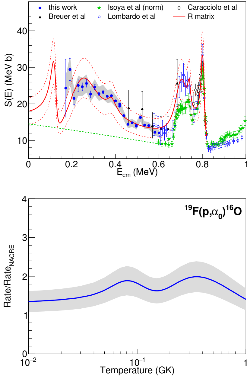
Figure 2.32: (Upper panel) S -factor of the ^{19}\text{F}(p,\alpha_0)^{16}\text{O} reaction at low energies ( \lesssim 1 MeV). Blue solid dots: experimental data obtained in this work (error bars: statistical errors; grey band: non-statistical errors). Black triangles: direct data by [299]. Blue empty circles: data by [228]. Green stars: data by Isoya et al [298] as normalized by NACRE [109]. Black empty diamonds: data by [300]. Green dashed line: non-resonant extrapolation reported in NACRE [109]. Red line: result of R -matrix best-fit of present data and data by Ref. [228]. White band within the red lines: confidence band of the fit. (Lower panel) Reaction rate calculation (expressed as ratio to NACRE) obtained from the R -matrix fit of the S -factor.
