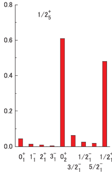
Figure 1.29: Spectroscopic factors of the ^{12}\text{C}(J_C^\pi) + n ( J_C^\pi = 0_1^+, 1_1^-, 2_1^+, 3_1^-, 0_2^+ ) and ^9\text{Be}(J_9^\pi) + \alpha ( J_9^\pi = 3/2_1^-, 1/2_2^-, 5/2_1^-, 1/2_1^+ ) channels for the 1/2_5^+ state in ^{13}\text{C} , E_x = 14.9 MeV. The strong ( \approx 0.6 ) 0_2^+ configuration indicates that this state is a candidate to be the ^{13}\text{C} Hoyle analog state. From [131].
