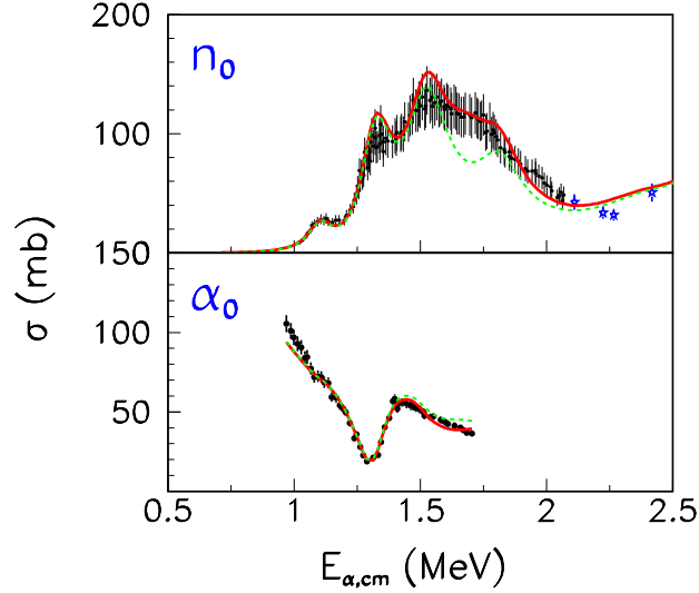
Figure 2.23: (upper panel) Zoom of ^9\text{Be}(\alpha, n_0)^{12}\text{C} integrated cross section data (see Figure 2.22). Green dashed line: R -matrix best-fit without the inclusion of the 1/2^+ state at 12.33 MeV. Red solid line: R -matrix best-fit with all the parameters of Table 2.3. (lower panel) The same of upper panel, but for the ^9\text{Be}(\alpha, \alpha_0)^9\text{Be} DCS at \theta_{cm} = 160^\circ .
