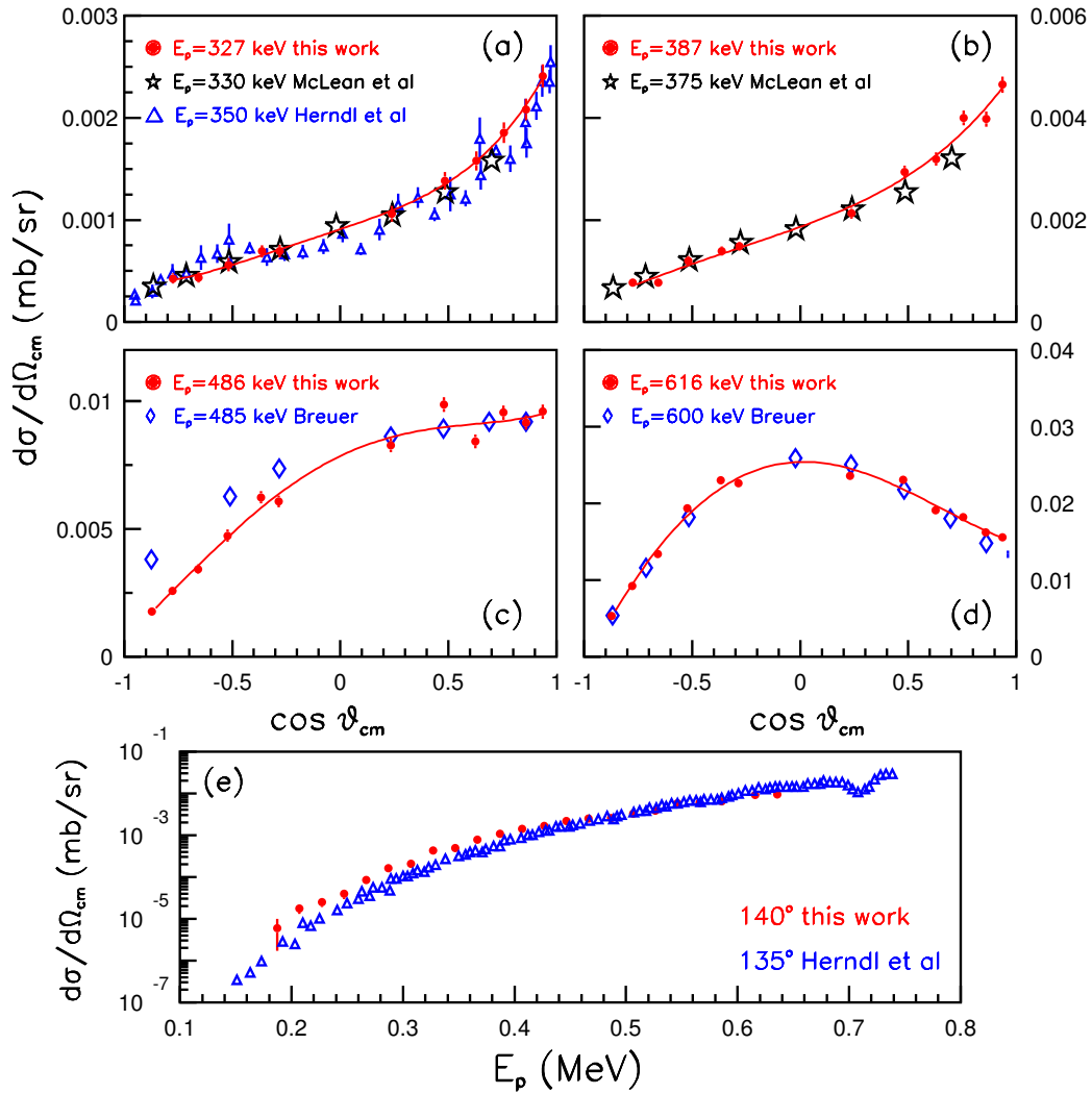
Figure 2.30: (Panels a-d) Angular distributions of the ^{19}\text{F}(p, \alpha_0)^{16}\text{O} reaction at E_p = 0.327, 0.387, 0.486 and 0.616 MeV. Red dots: Present data. Red lines: Legendre polynomial fits. Black stars: data from Ref. [304]. Blue diamonds: data from Ref. [299]. Blue triangles: data from Ref. [302]. Data from Refs. [299, 302, 304] have been normalized to our cross section scale as discussed in the text. (e) Excitation function obtained in this experiment at 140^\circ (red dots) compared with data reported at 135^\circ in Ref. [148] (blue triangles).
