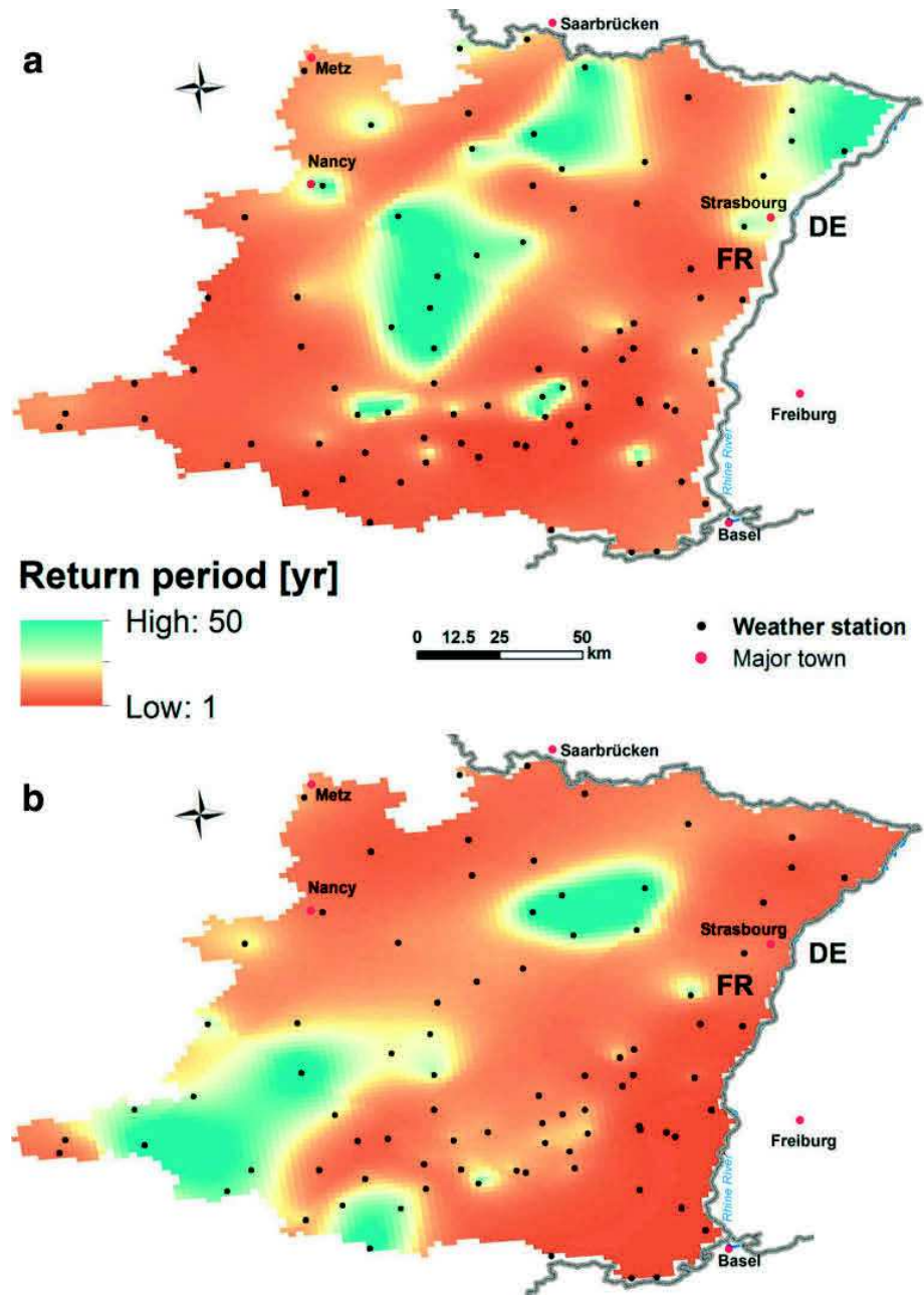
Fig. 8 Superimposed and averaged return period estimates during EPEs in a SHY and b WHY in VG
