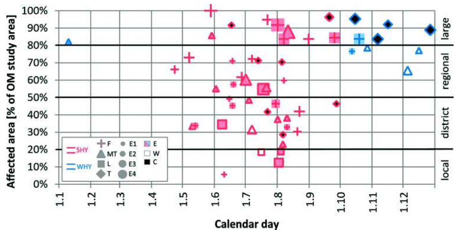
Fig. 3 Annual course of EPEs and dependent spatial characteristics of EPEs in OM (abbreviations described in Section 2.6)
