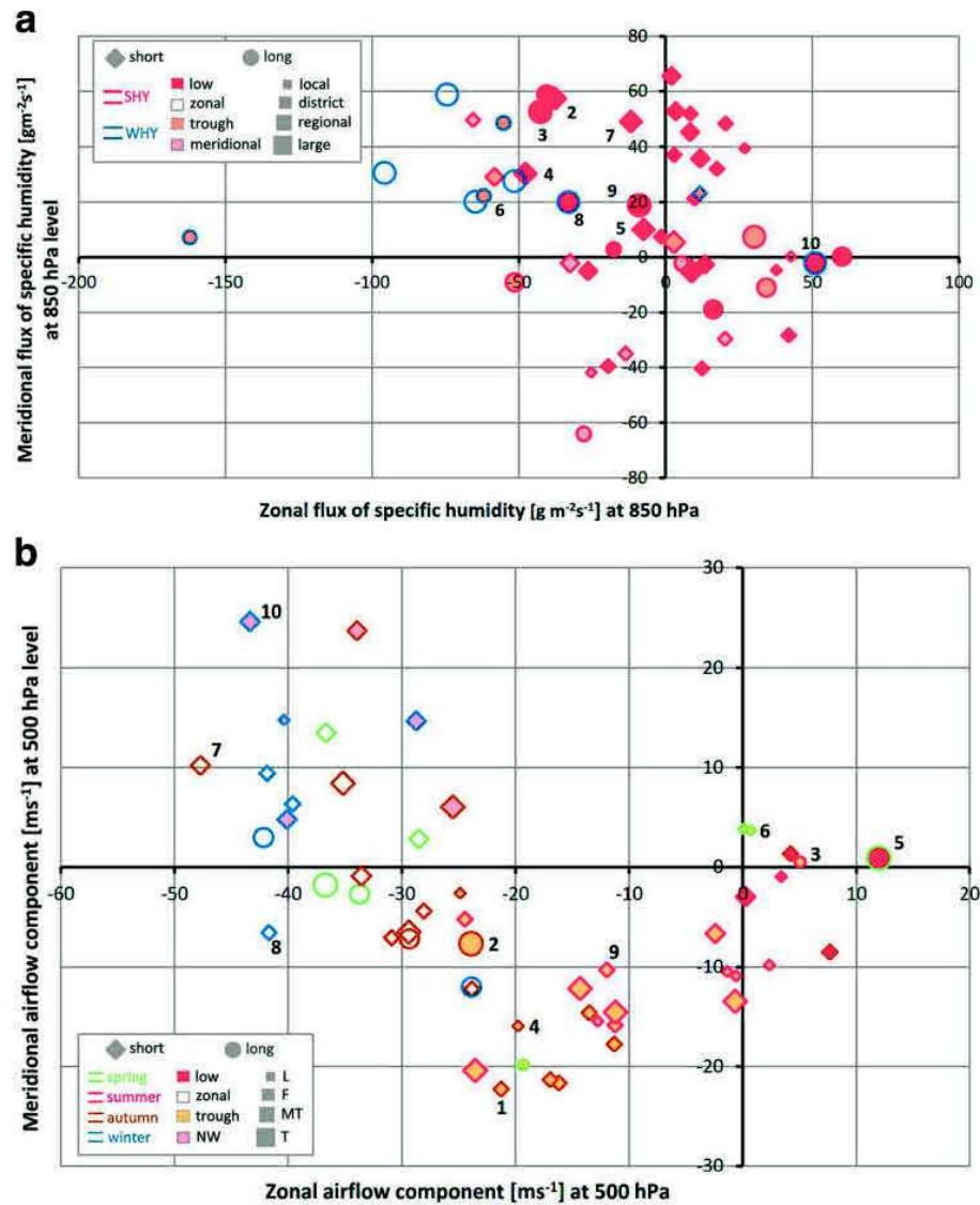
Fig. 2 Significantly dependent characteristics of EPEs in a OM and b VG. Ten strongest EPEs from OM (Table 1) and VG (Table 2) are numbered starting from the strongest (Nr. 1), except one in OM where it was beyond the available synoptic dataset. Note that the reversed values of the components of flux of specific humidity are displayed in a to match the cardinal points
