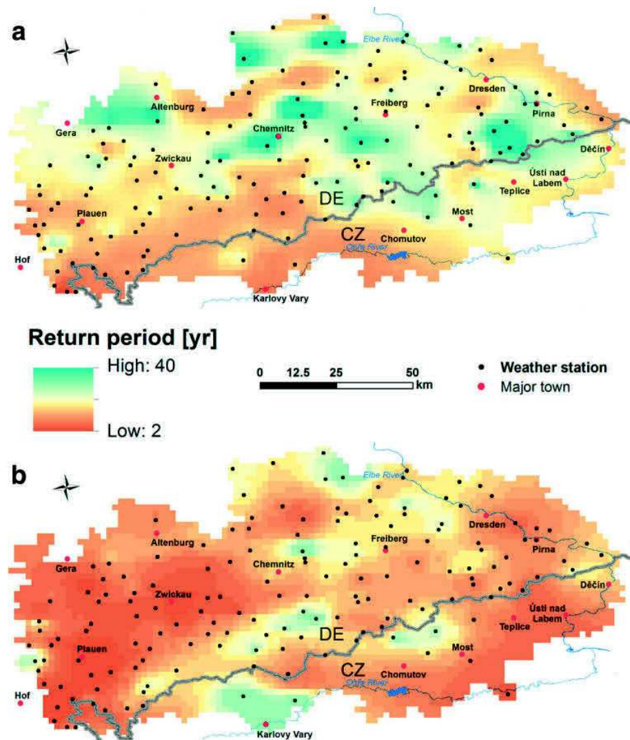
Fig. 7 Superimposed and averaged return period estimates during EPEs in a SHY and b WHY in OM
