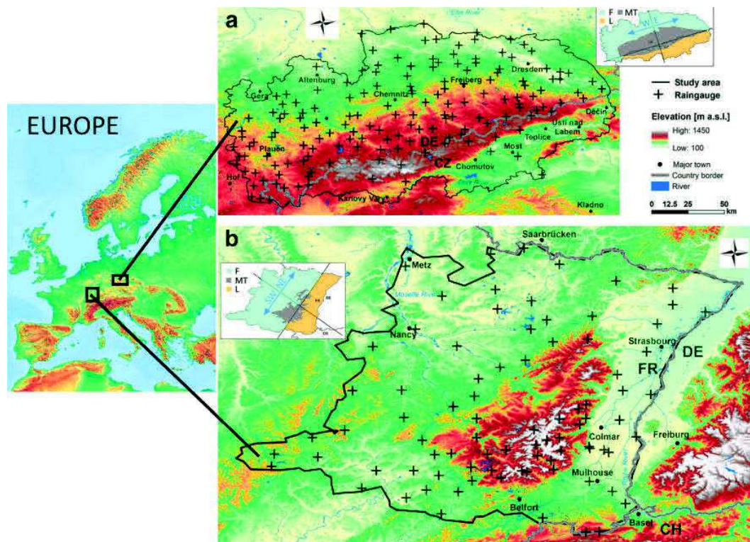
Fig. 1 Study area of (a) the Ore Mountains and (b) the Vosges Mountains, and the spatial distribution of the (a) 167 and (b) 84 analysed rain gauges. The relief is represented in colour scale, i.e. the highest
