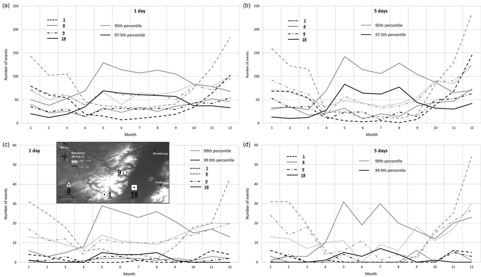
Figure 4. Monthly distribution of 1-day (a and c) and 5-day (b and d) heavy precipitation events for four stations exceeding four different thresholds – 95th, 97.5th (a and b), 99th, 99.9th (c and d) percentiles respectively. The thresholds are distinguished by a diverse grayscale. Each station is one of the representatives of the four categories of stations displayed in Figure 2 and Table 1 in bold. As in Figure 2, the categories of stations are indicated by a different type of line – MT stations by the dashed lines (no. 1); LSp stations by the broken lines (no. 9); URP stations by the solid lines (no. 18); WSd stations by the dotted lines (no. 8).
