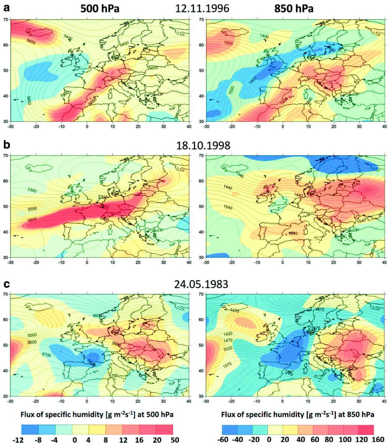
Fig. 5 Meridional (a, c) and zonal (b) component of flux of specific humidity in colour scale and geopotential height in contour at (left) 500 hPa level and (right) 850 hPa level for the three frequent synoptic patterns during EPEs (the day with highest E_{10} ) in VG: a trough and
