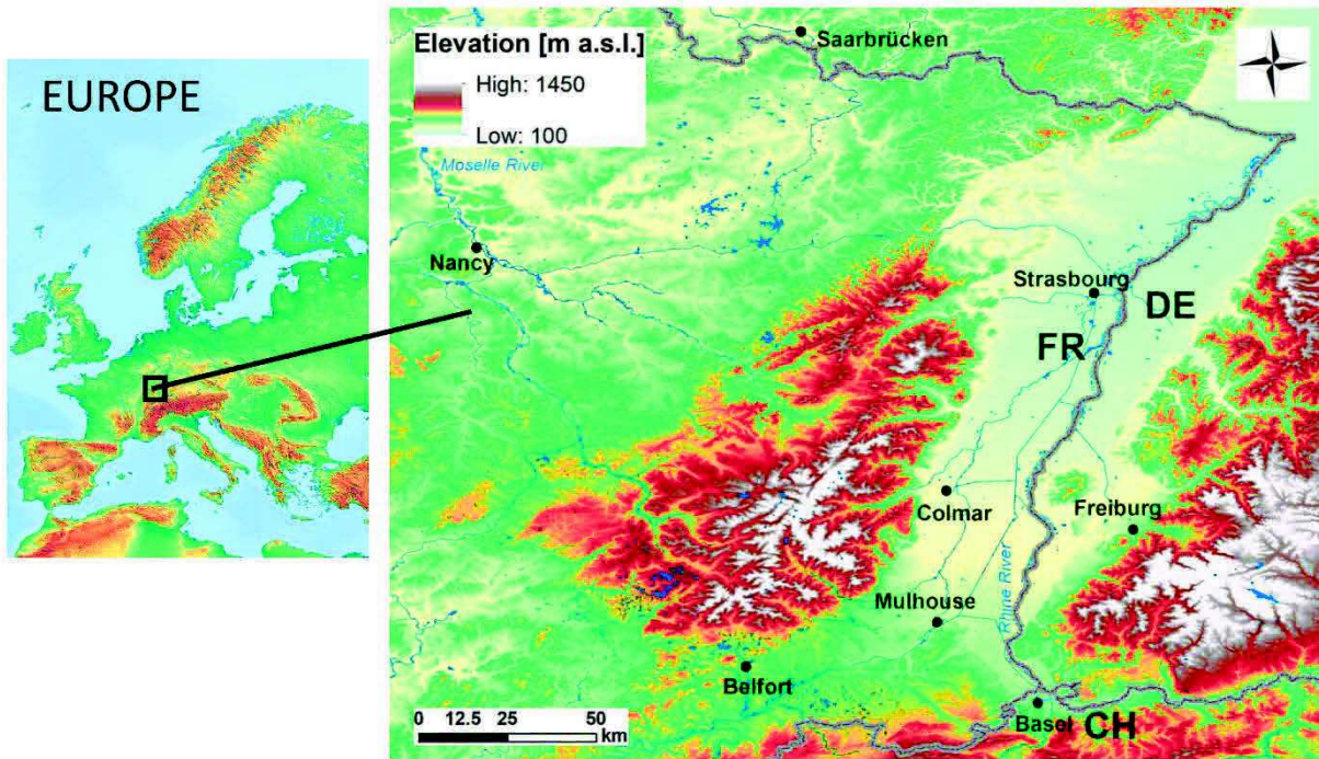
Figure 2 Topographical map of the Vosges Mountains (right side) and its location in Europe (left side)
