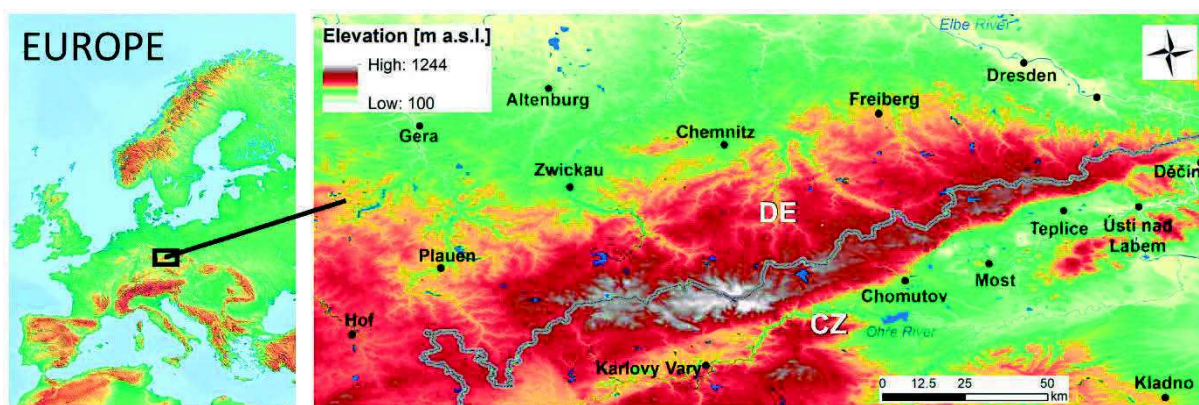
Figure 1 Topographical map of the Ore Mountains (right side) and its location in Europe (left side)
