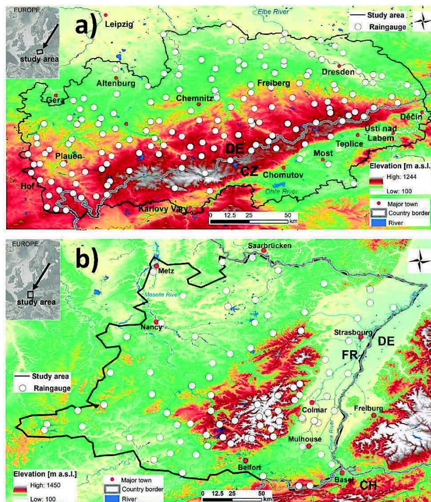
Figure 3 Study area and the distribution of rain gauges in (a) Ore Mountains and (b) Vosges Mountains
