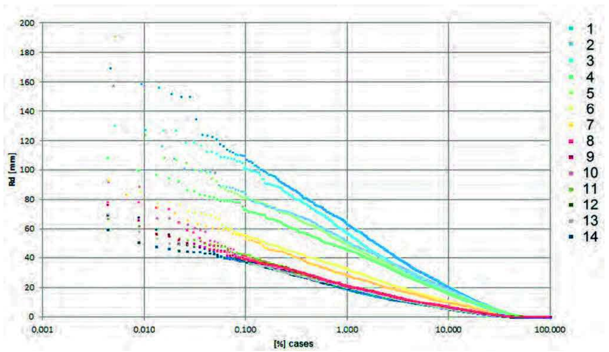
Fig. XXIII The variability of daily precipitation totals ( Rd ). Stations are listed in the order of descending annual rainfall, station numbers are identified in Table 1. The x-axis is expressed in logarithmic scale.
