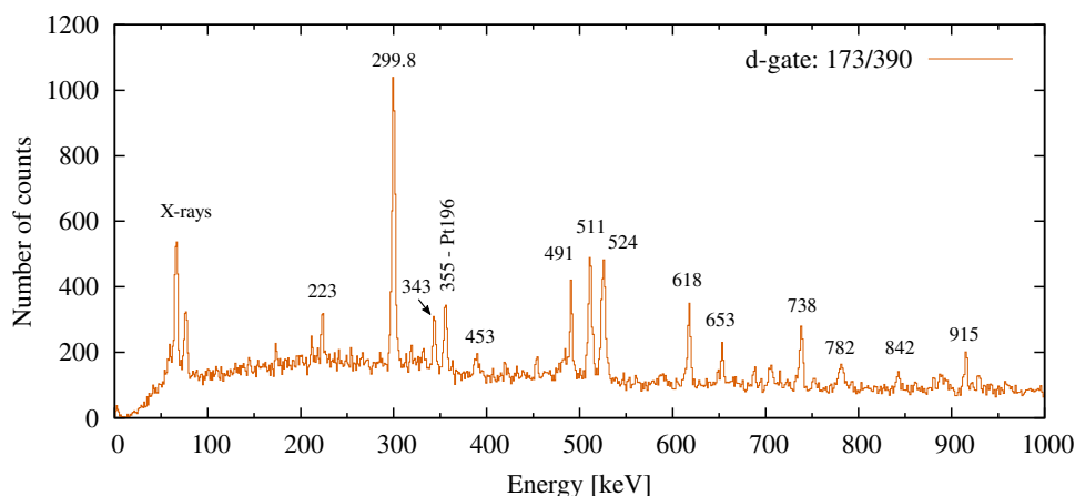
Figure 11.6: Double coincidence spectrum of the the 173 keV and the 390 keV transition as the lower two transitions of the Warner cascade.
