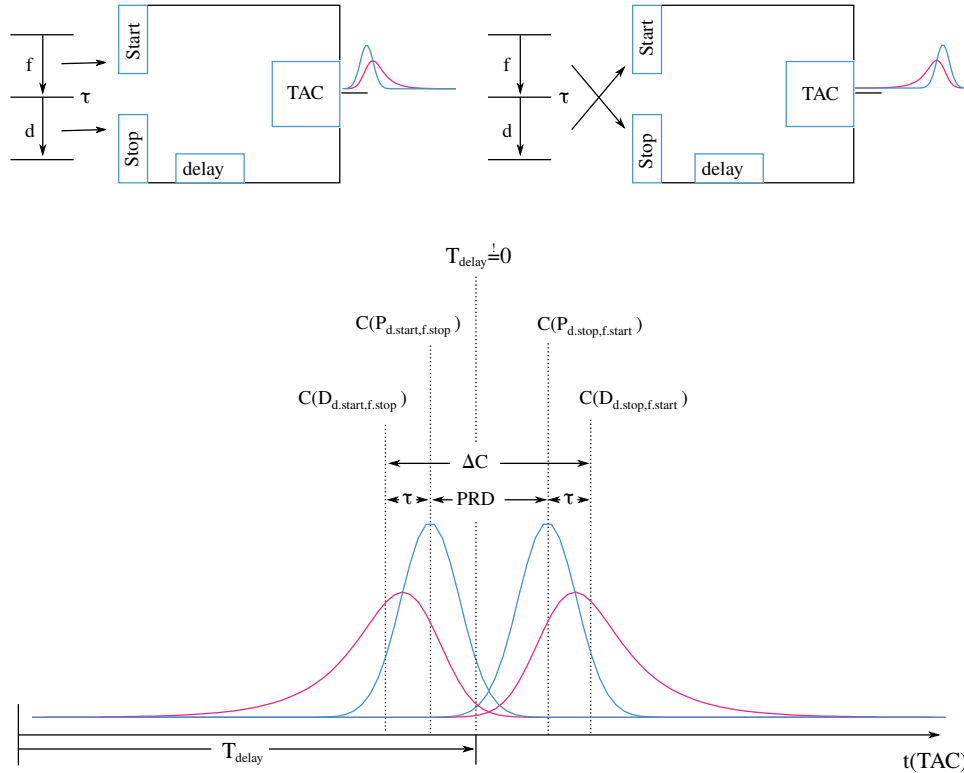
Figure 2.15: Schematic illustration of the GCDM for a two detector fast-timing circuit: Upper part: The feeding transition triggers the start detector and the decaying transition stops (left). The decaying transition triggers the start detector and the feeding transition stops (right). Lower part: The resulting spectra for both options illustrated in the upper part for a prompt transition (in blue) and for a delayed transition corresponding to the lifetime \tau of the the state. The delay is shifted to t=0 . The centroid differences \Delta C and PRD are indicated. Note the asymmetry of the centroids C(P) and C(D) with respect to t=0 coming from the different time responses of the two branches. The difference is however not affected by this.
