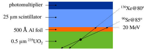
Figure 8.1: Simplified fission event tagger based on a solid plastic scintillator illustrating the limitations of fission fragment discrimination efficiency. Fission fragments being emitted under small angles lose too much energy in the target and the aluminum layer respectively. The calculation was done with LISE++ .
