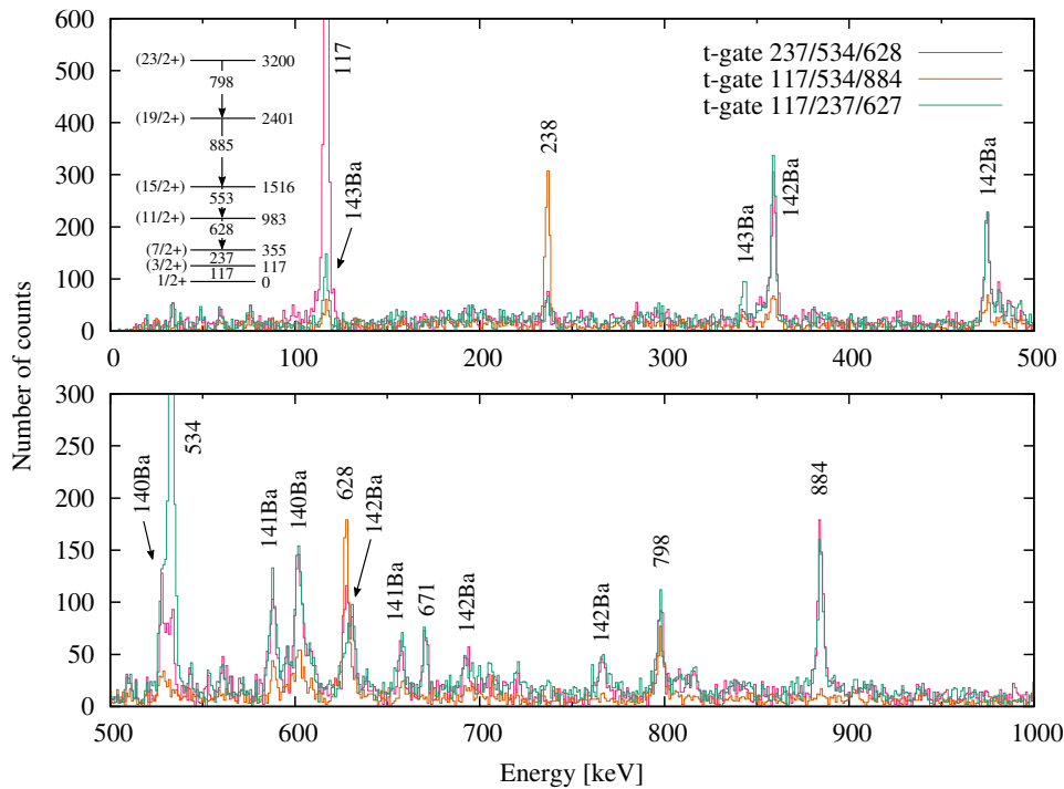
Figure 3.5: Triple coincidence spectra for various combinations of the positive parity band in ^{93}\text{Kr} . The inlay shows the level scheme of this band. See text for further explanations.
