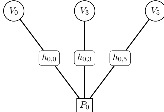
FIGURE 2.2 – Tanner Graph of a NB-LDPC code.
