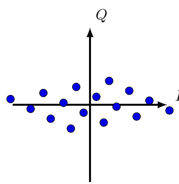
FIGURE 4.5 – Rotated 16-QAM modulation with severe fading on Q axis
