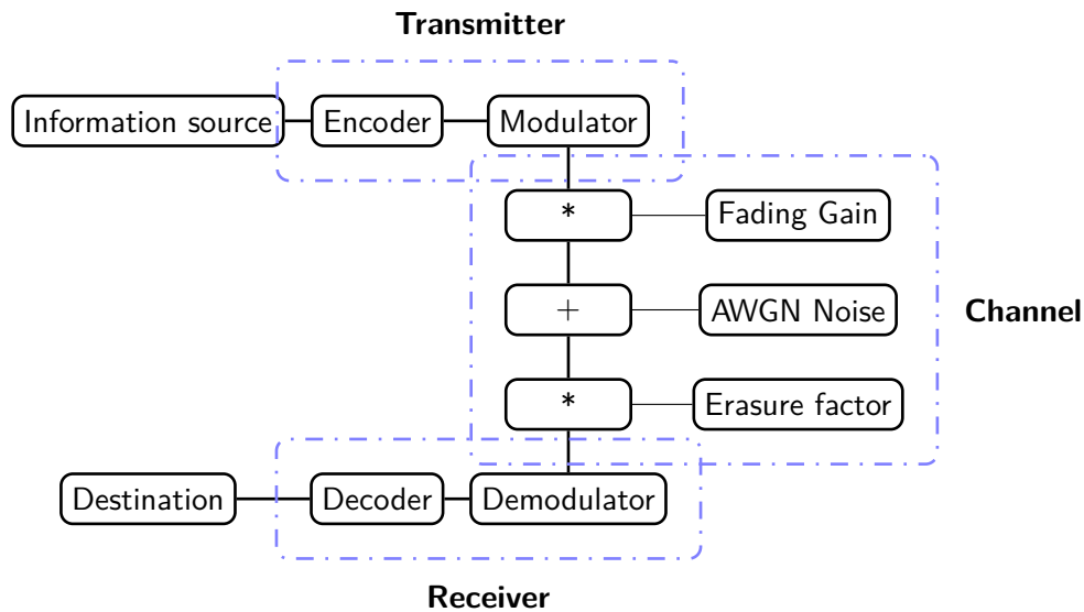
FIGURE 3.2 – Coded Modulation transmission scheme over Rayleigh channel with erasure.
