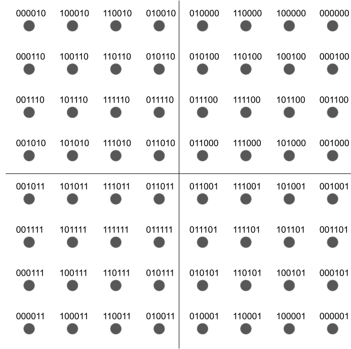
FIGURE 5.3 – Mapping \pi_2
