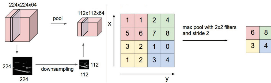
Figure 1.8: Max-pooling. Source: [122].
