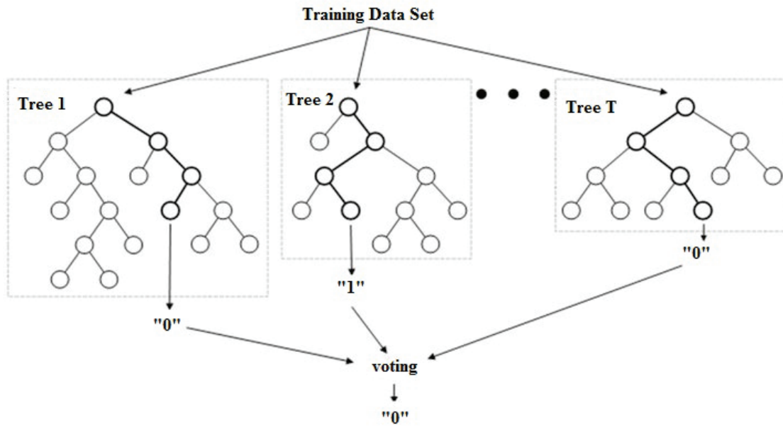
Figure 1.2: Random forests: majority voting. Figure adapted from [163].
