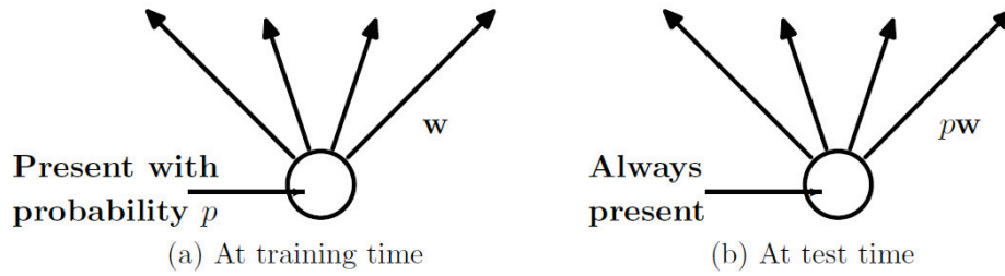
Figure 1.10: Dropout during training. Source: [213].
