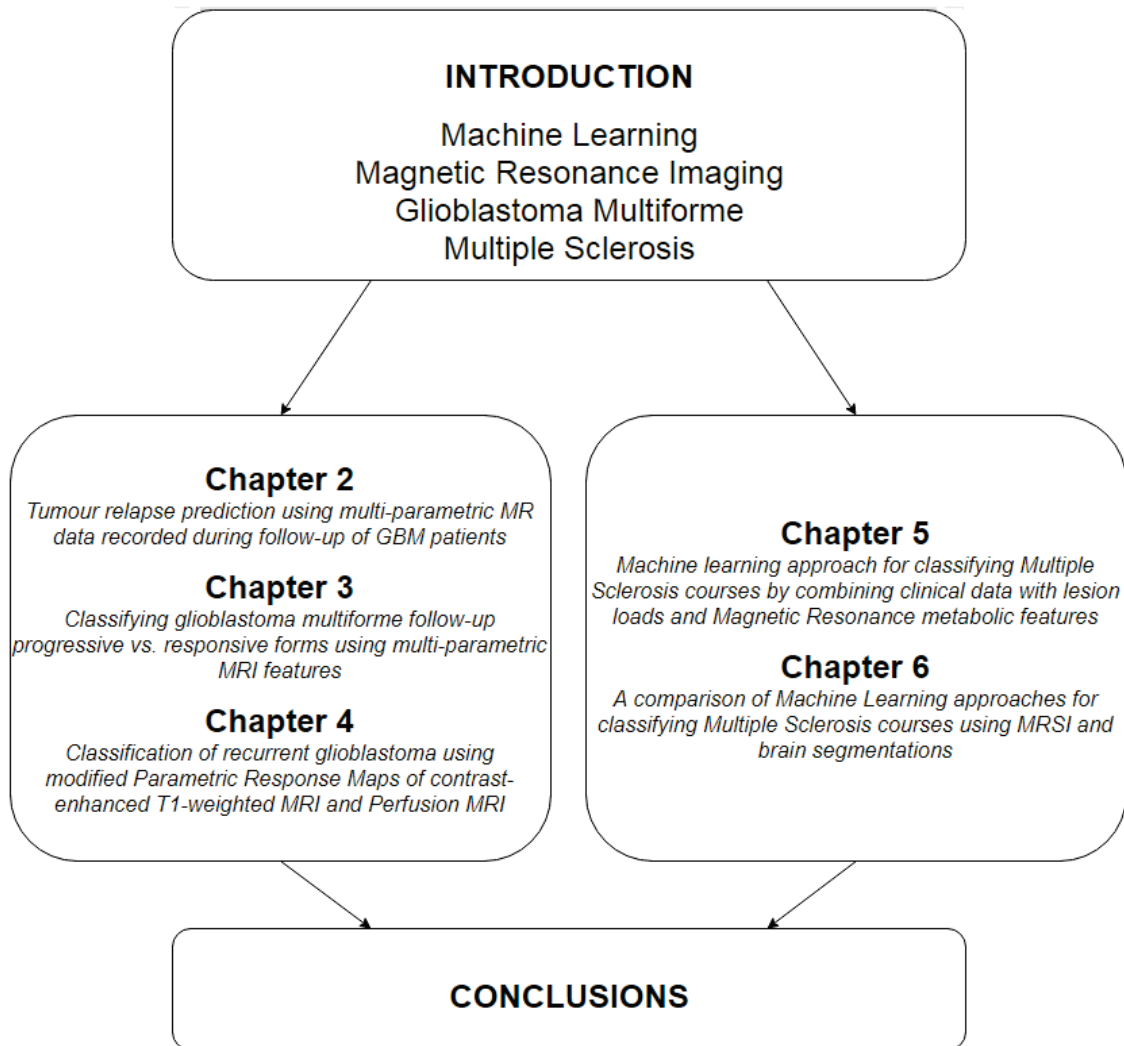
Figure 1.29: Thesis outline.
