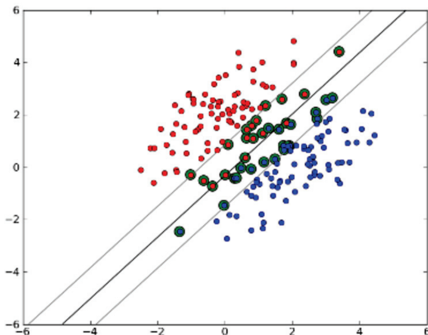
Figure 1.1: SVM: finding the best separation plane
