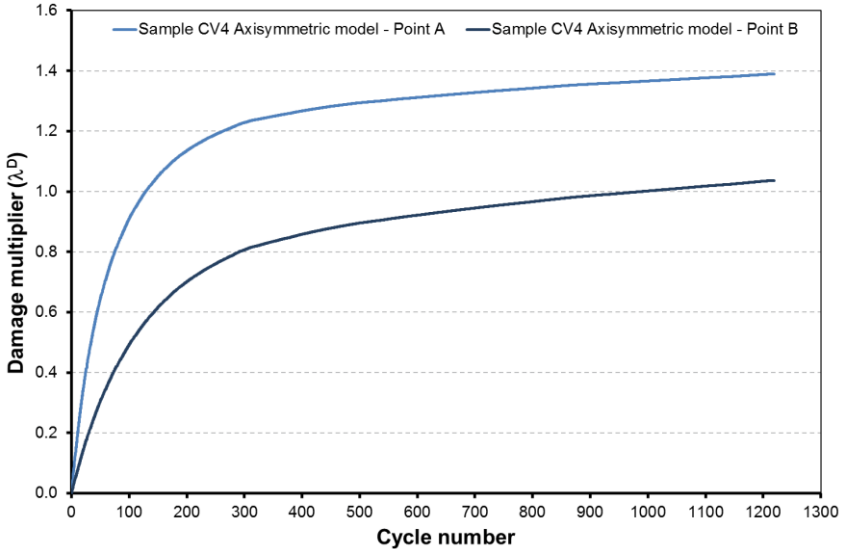
Figure 4-62 Sample CV4: Damage multiplier evolution
