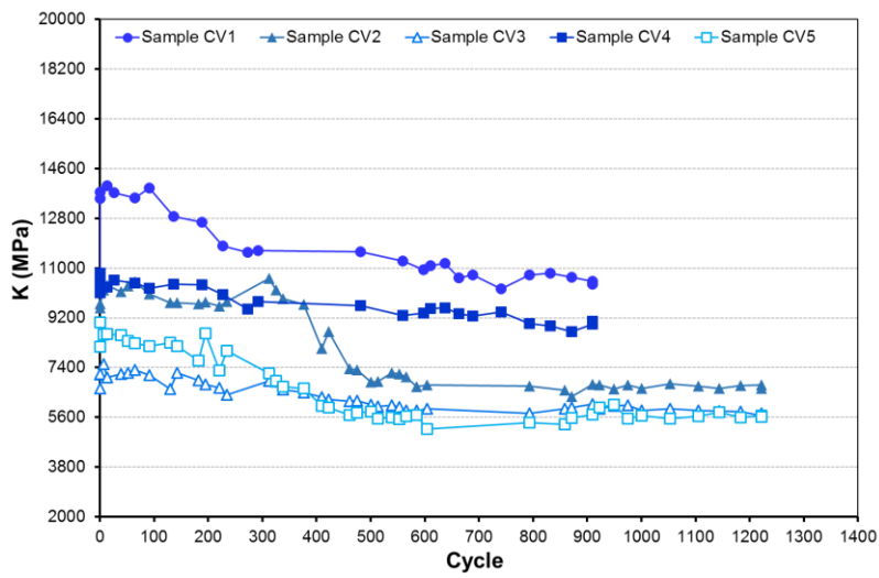
Figure 3-59 Bulk modulus evolution – samples group 1
