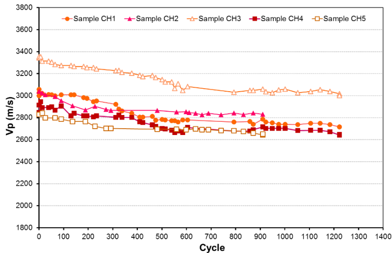
Figure 3-55 Compression elastic wave propagation velocity evolution- samples group 2: a) samples drilled in vertical direction b) samples drilled in horizontal direction
