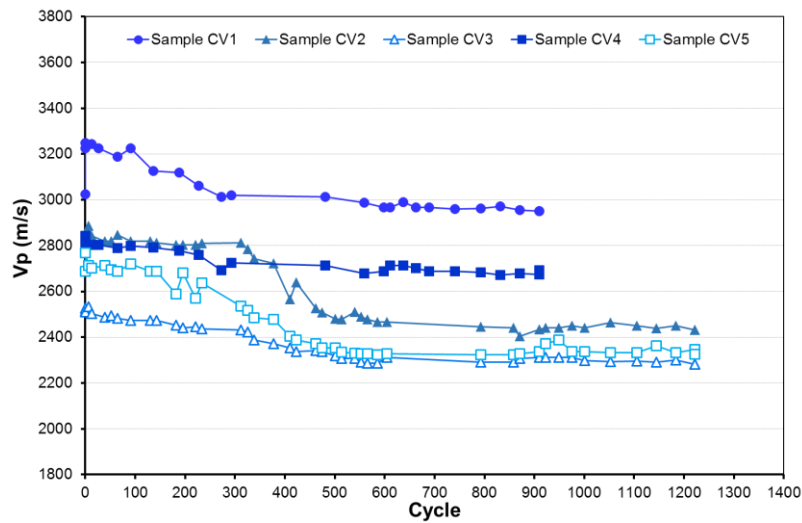
Figure 3-54 Compressive elastic wave velocity evolution samples group 1
