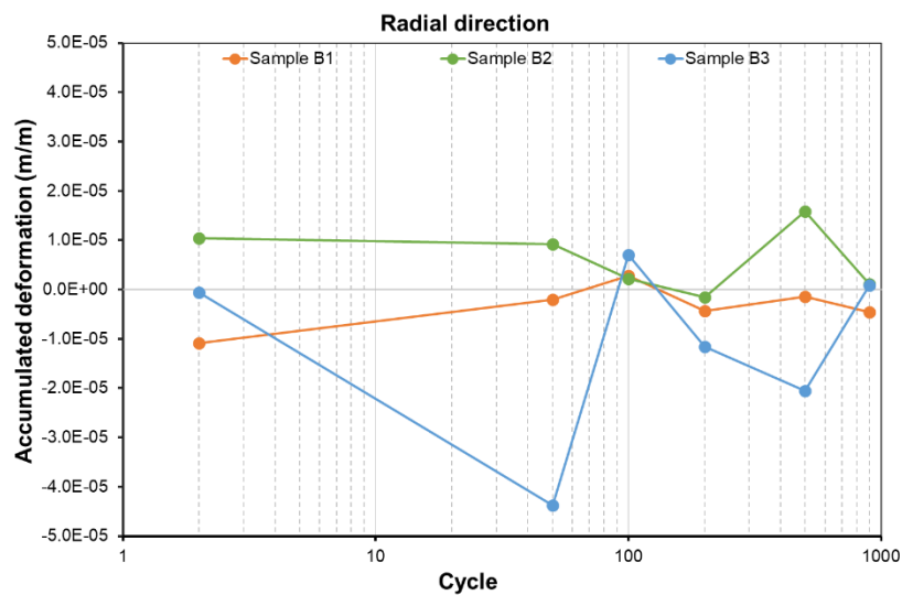
Figure 3-51 Radial direction accumulated deformation – samples group 1
