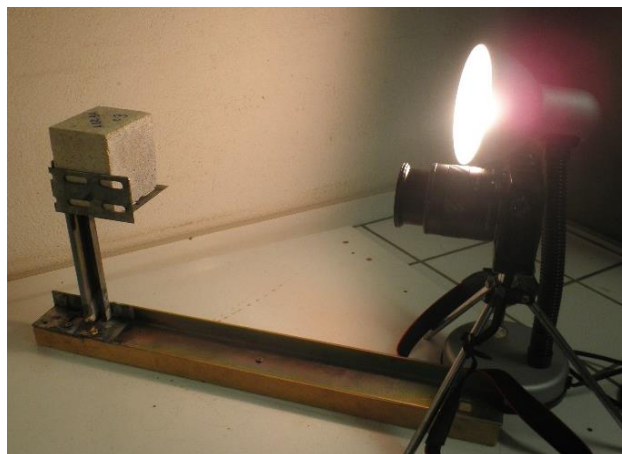
Figure 3-29 Fixing device
