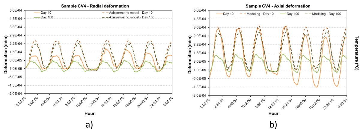
Figure 4-66 Sample CV4: Strains amplitude a) radial strains b) axial strains
