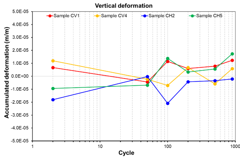
Figure 3-52 Vertical direction accumulated deformation – samples group 2
