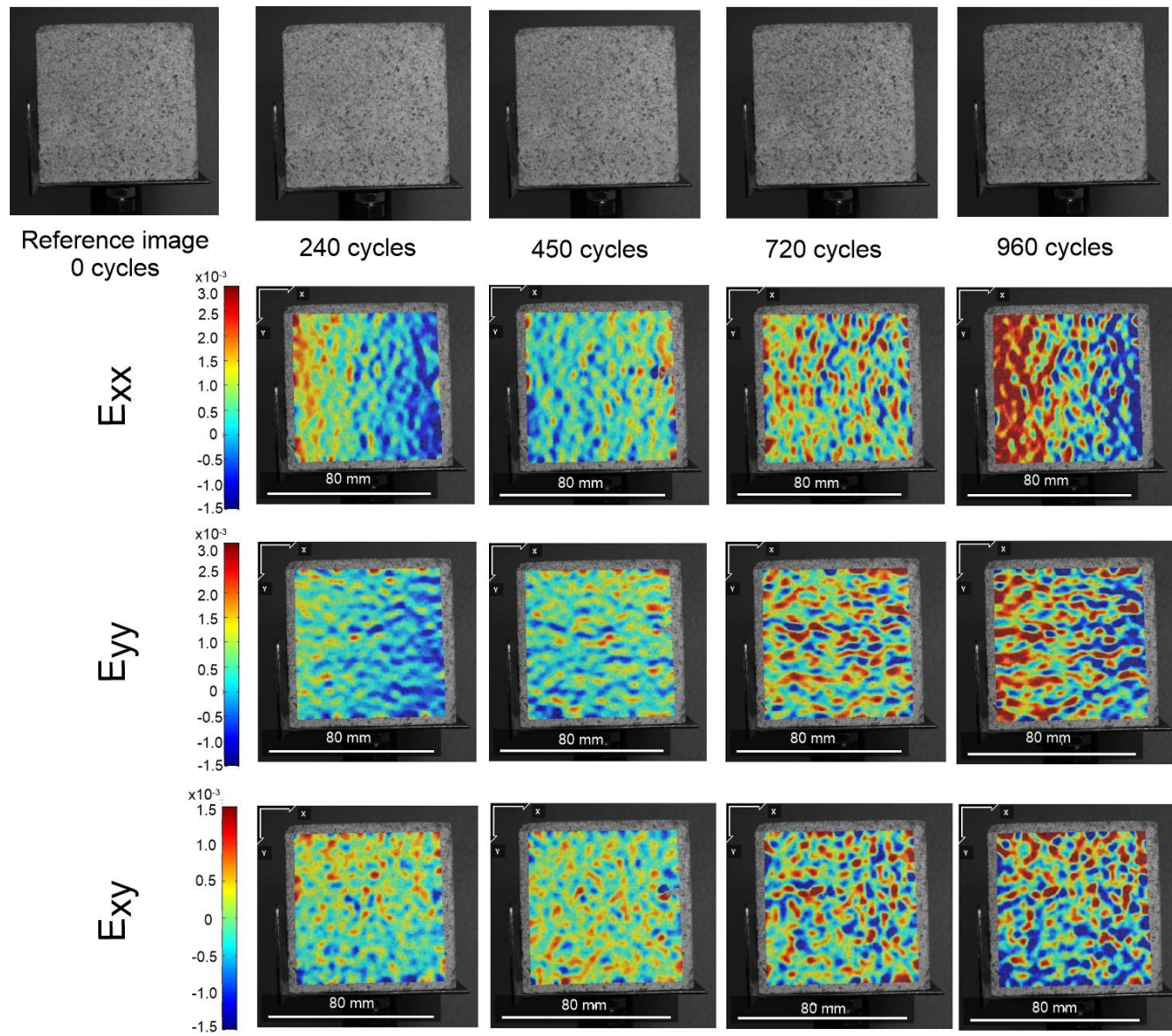
Figure A-3 DIC analysis for sample C1 – face without speckle pattern
