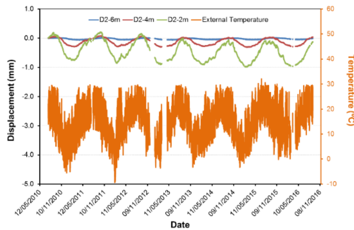
Figure 2-17 Extensometers measures: a) D1 b) D2
