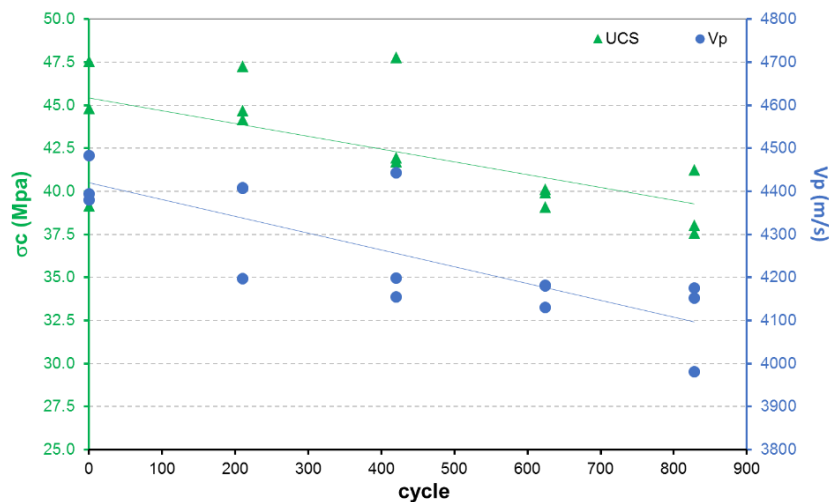
Figure 3-62 UCS and VP evolution
