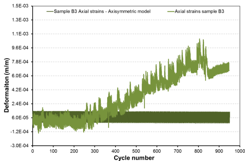
Figure 4-52 Sample B3: Axial strains
