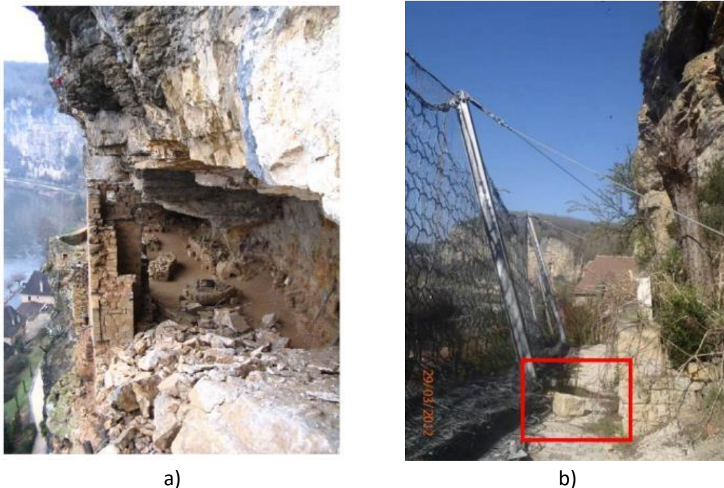
Figure 2-8 First level of risk a) Remaining blocks inside the cavern b) Wire mesh installed
