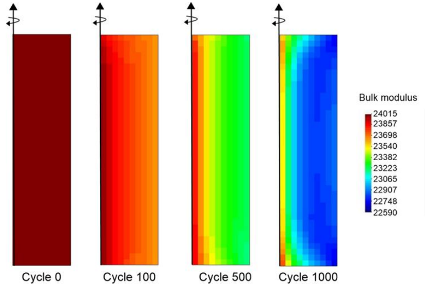
Figure 4-49 Sample B3: Bulk modulus evolution in the sample
