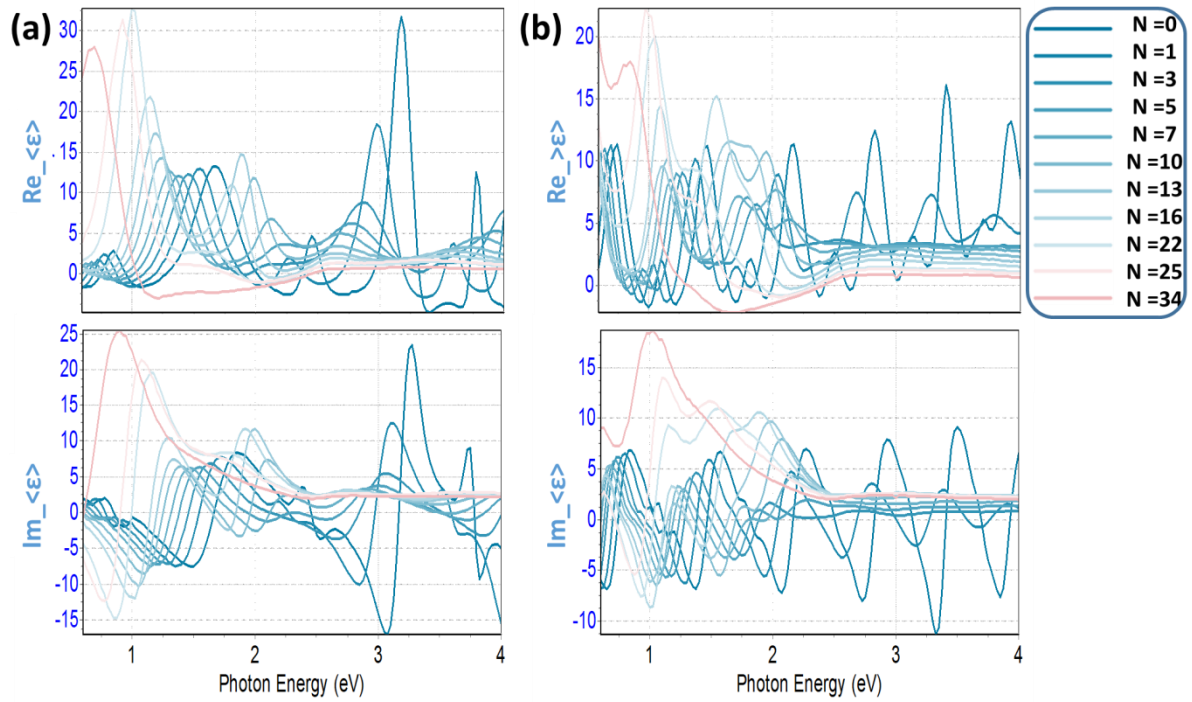
Figure IV. 18 Real (upper plots) and imaginary (lower plots) parts of \langle\epsilon\rangle measured at the angle of incidence 65^\circ , as a function of the photon energy for gradually increasing values of the number N of gold loading cycles (from N=0 to 34). (a) shows the thin films, with thickness ca. 300 nm while (b) shows the thick films, with thickness ca.700nm.
