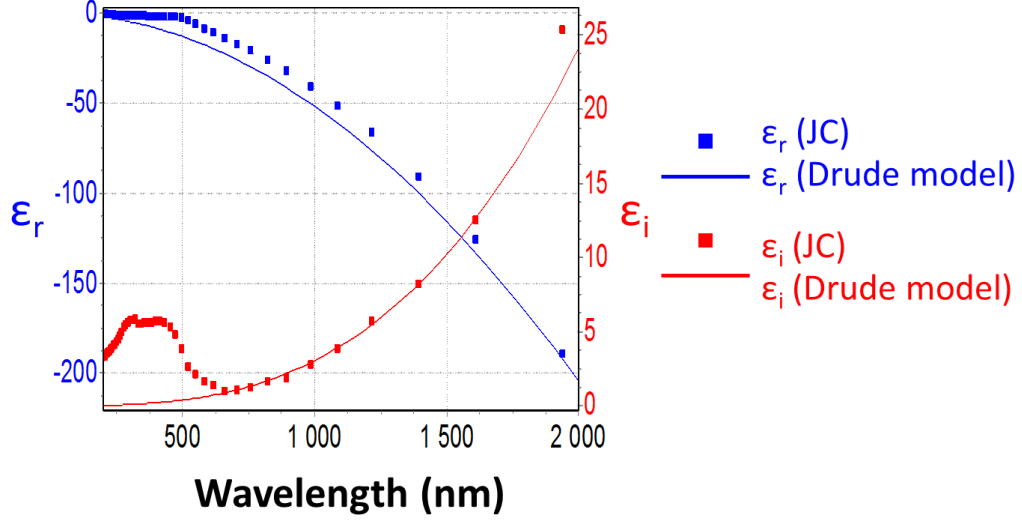
Figure I. 25 Permittivity of gold taken from JC (dots) and compared with the Drude model approximation (continuous curves)
