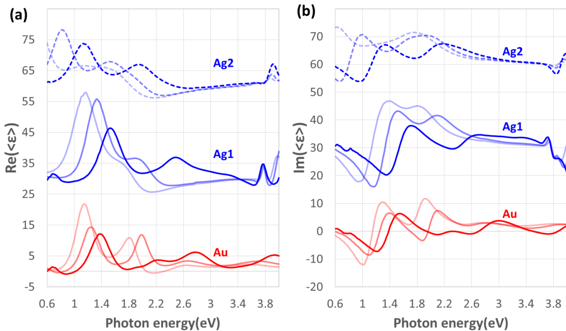
Figure VI. 19 Real (a) and imaginary (b) parts of the pseudo permittivity \langle \epsilon \rangle from the ellipsometry data. The ellipsometry data are measured at AOI 65°. The different impregnation cycles for loading metal N=5 , N=10 and N=15 are shown in the figure with gradually lighter colors. Au stands for the sample with gold NPs (Figure VI. 17(a)), Ag1 stands for sample with silver NPs in the top 4 layers (Figure VI. 17(b)), and Ag2 stands for the sample with silver NPs in the whole film (Figure VI. 17(c)). The curves are vertically shifted for clarity.
