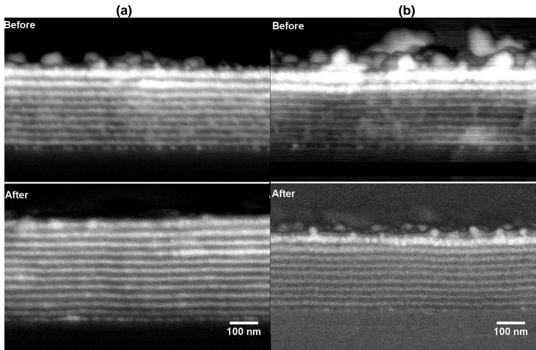
Figure V. 12 SEM images of (a) N=20 (b) N=30 . Before means gold loading follow the Normal Process. After means gold loading follow the Annealing Process.
