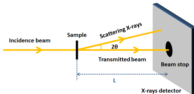
Figure II. 8 Schematic of Small Angle X-ray Scattering (SAXS) geometry
