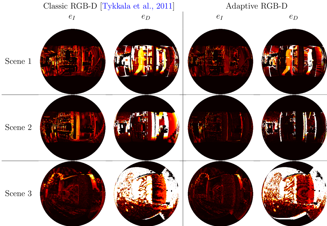
Figure 5.8 – Intensity ( e_I ) and geometric ( e_D ) errors between spherical RGB-D frames with large displacements for three distinct indoor and outdoor sequences. The colors encode the error absolute value (hot colors indicate bigger errors than cold colors). The left column is the classic RGB-D cost and the last column the adaptive one. Scene 1 corresponds to the registration between the two left frames shown in fig. 5.1 from the sequence whose trajectory is displayed in fig. 5.10. Scene 2 corresponds to a registration from the trajectory depicted in fig. 5.11. Finally, Scene 3 is an outdoor sequence which frames are depicted at right of fig. 5.1.
