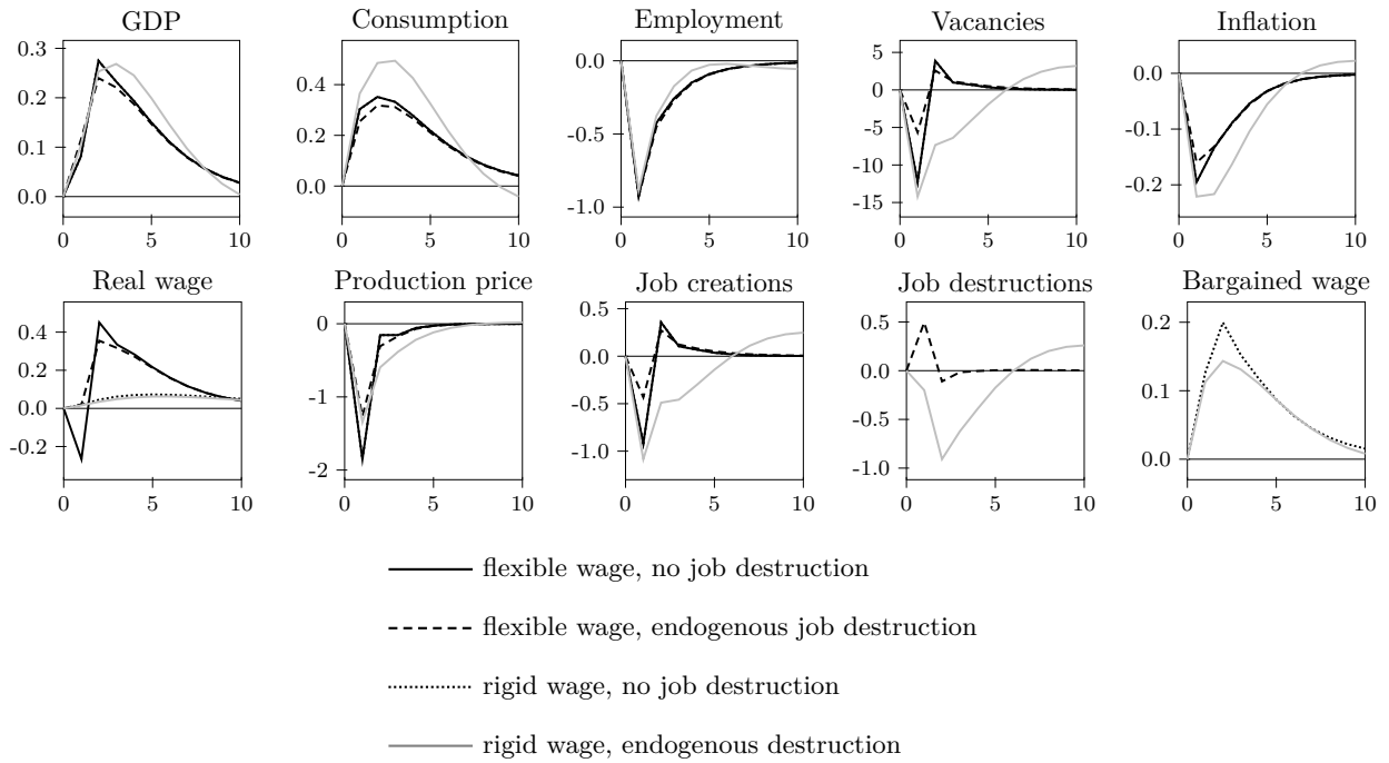
Figure 2.14: Technology shock
