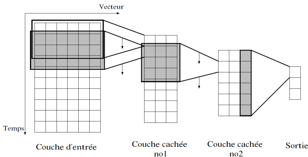
FIGURE 2.5 – Architecture du TDNN. Image issue de Durand [1995]
