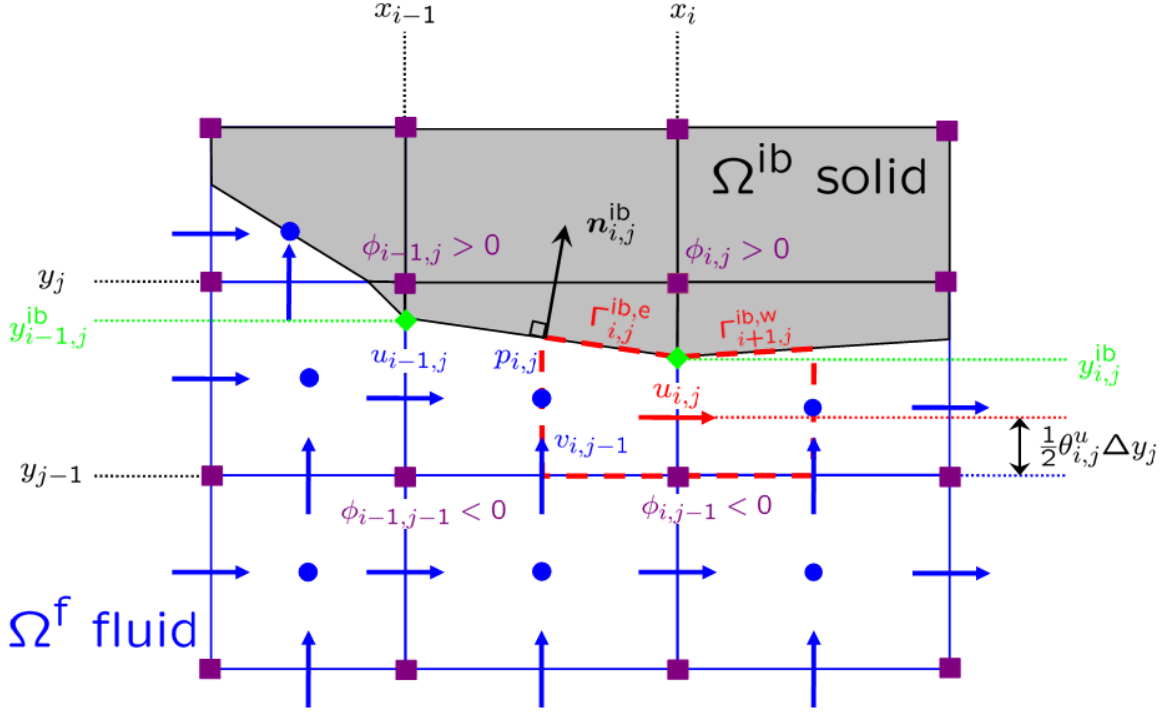
Figure 2.6: Staggered arrangement of the variables near the trapezoidal cut-cell \Omega_{i,j} on the LS-STAG mesh reprinted from [22].
