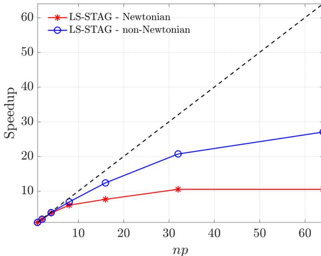
Figure 4.5: The speedup of LS-STAG solver versus the number of processors ( np ) in the strong scaling measurement. The dashed line (--) shows the ideal speedup.
