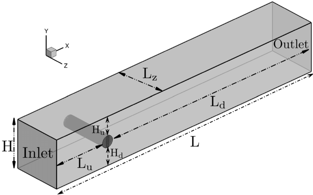
Figure 4.11: Computational domain for the cylinder flows of Section 4.3.
