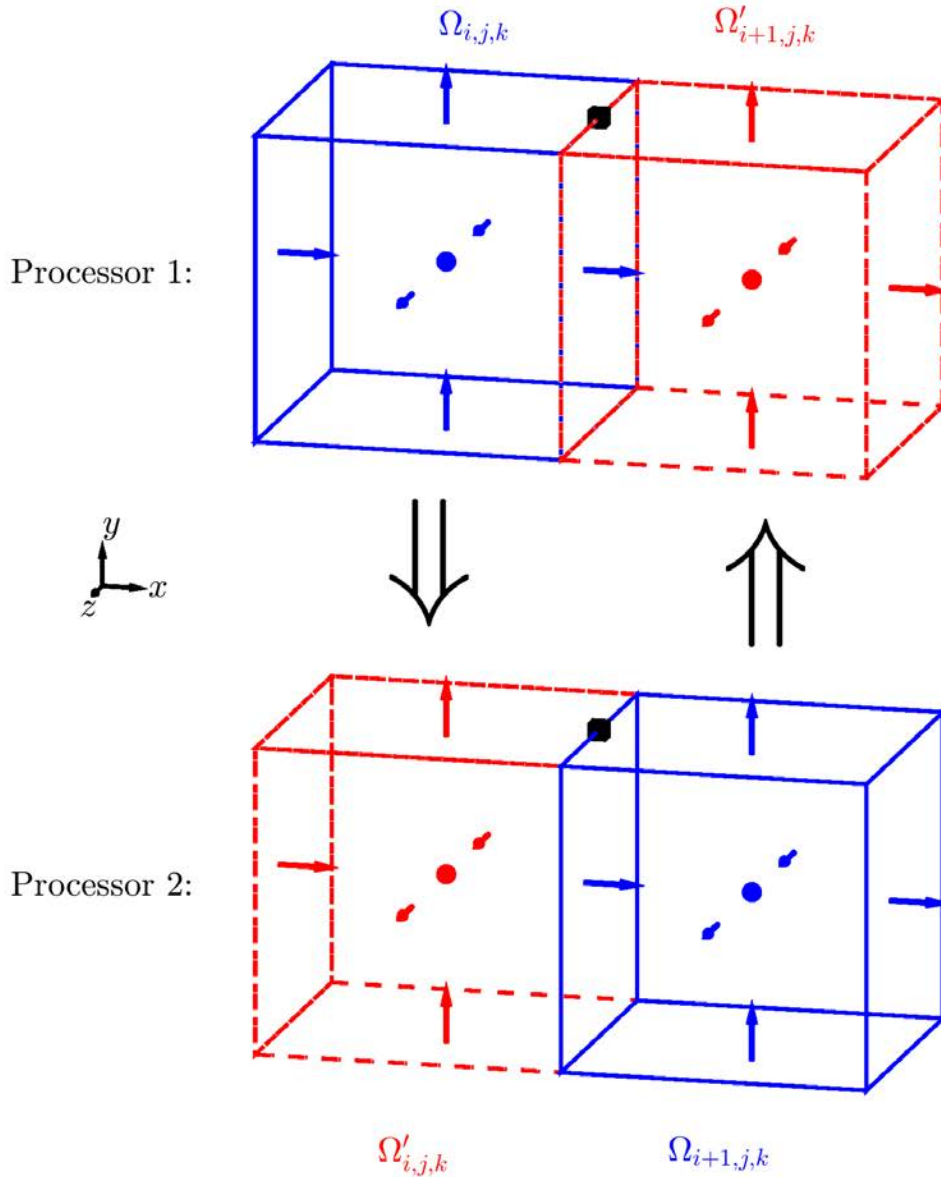
Figure 4.2: The communication between two successive processors. The velocity components in cells \Omega_{i,j,k} and \Omega_{i+1,j,k} related to two different processors (1 and 2), are respectively stored in overlapping cells \Omega'_{i,j,k} and \Omega'_{i+1,j,k} via MPI “point-to-point” communication routines. The data in blue cells are computed on current processor while those in red (overlapping) cells are retrieved from the neighbor processors.
