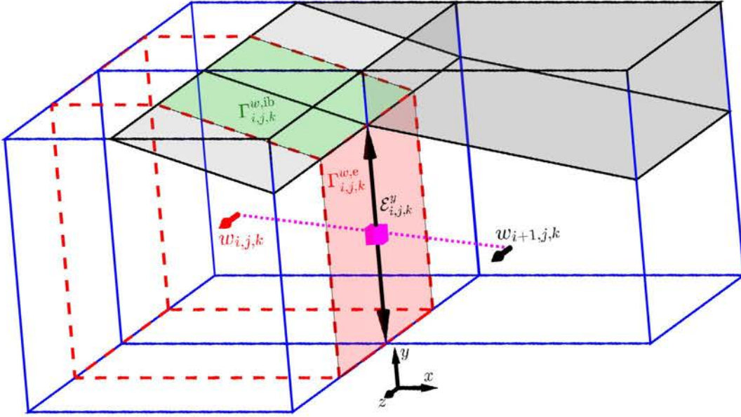
Figure 3.18: Illustration of an arbitrary staggered control volume \Omega_{i,j,k}^w \in \Omega_{i,j,k} \cup \Omega_{i,j,k+1} (red dashed line (---)) whose eastern face \Gamma_{i,j,k}^{w,e} is shaded in red and its solid face \Gamma_{i,j,k}^{w,ib} is highlighted in green. Velocity gradient \partial w/\partial x|_{i,j,k} (■) is located at the center of edge \mathcal{E}_{i,j,k}^y . The adjacent velocity vectors, w_{i,j,k} and w_{i+1,j,k} , are connected by a dotted line (··) which is not perpendicular to the face \Gamma_{i,j,k}^{w,e} .
