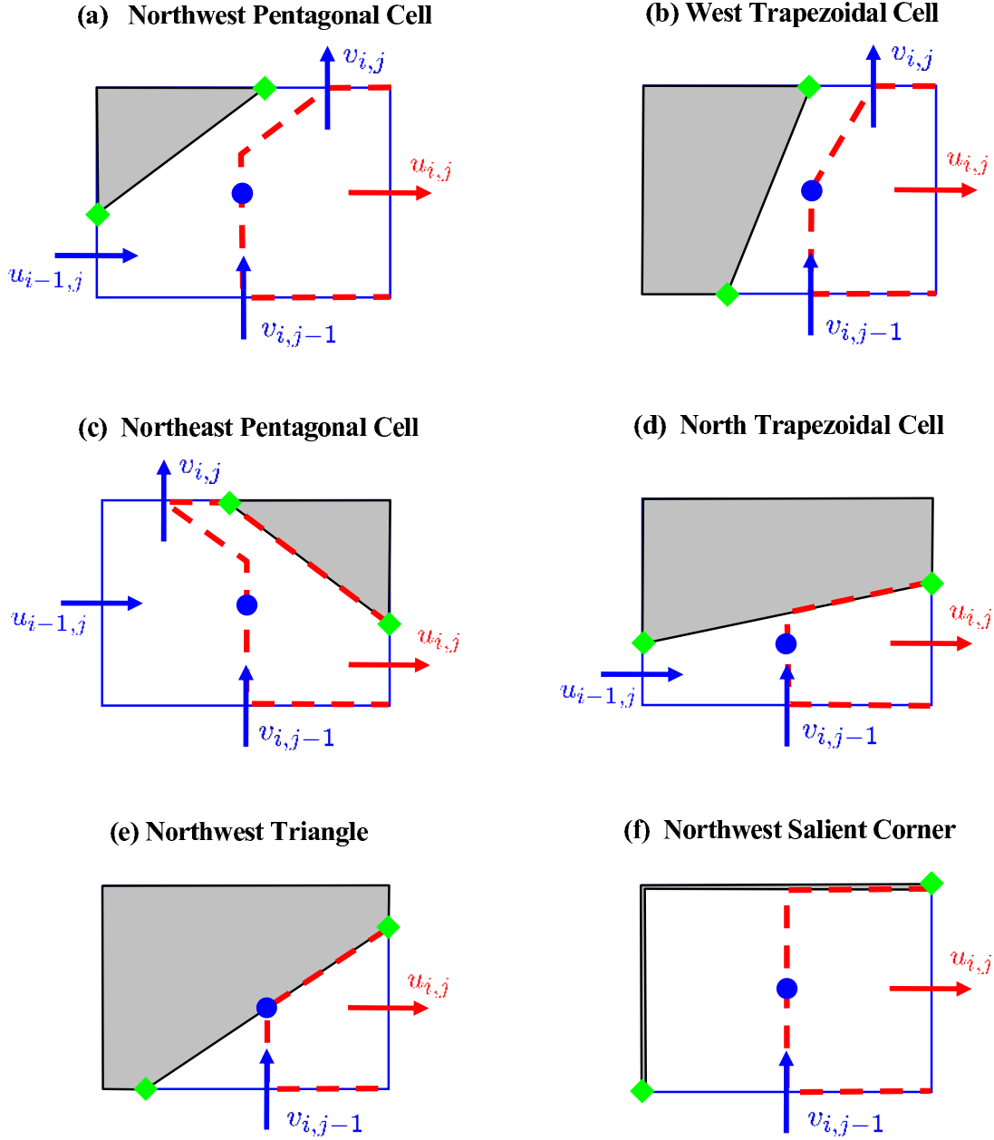
Figure 2.8: Basic types of half u_{i,j} control volumes, \Omega_{i,j}^u , inside the cut-cell \Omega_{i,j} reprinted from [22]. The green diamonds (◆) denote the locations of the discretization of the velocity boundary conditions. Note that the re-entrant corner of a Cartesian mesh is a particular case of pentagonal cell (c) when \phi_{i,j} = 0 , and the particular case of a salient corner (f) in which \phi_{i-1,j-1} = \phi_{i-1,j} = \phi_{i,j} = 0 and \phi_{i,j-1} < 0 only differs in definition of the cell volume with the limiting case of triangle (e) where \phi_{i-1,j-1} = \phi_{i,j} = 0 , \phi_{i-1,j} > 0 and \phi_{i,j-1} < 0 .
