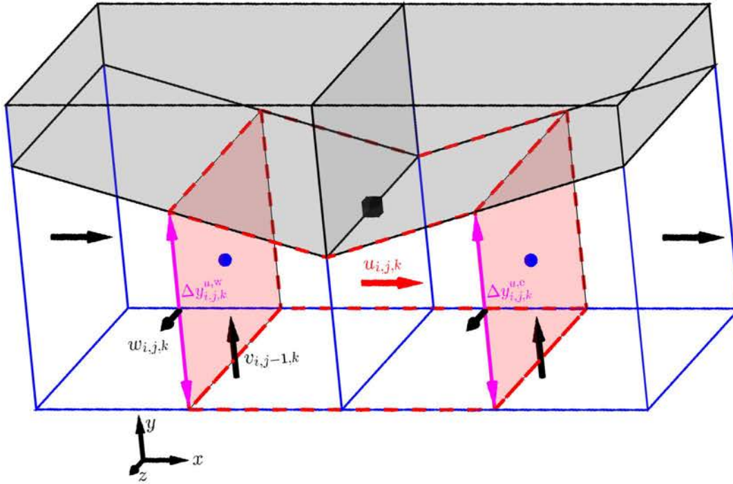
Figure 3.20: Illustration of the control volume \Omega_{i,j,k}^u in the vicinity of two trapezoidal cells (red dashed line (—)). The western and \Gamma_{i,j,k}^{u,w} ( \Delta y_{i,j,k} \times \Delta z_k ) and eastern \Gamma_{i,j,k}^{u,e} ( \Delta y_{i,j,k} \times \Delta z_k ) faces are shaded in red. The shear stress \dot{\gamma}_{xy}|_{i,j,k} is located at the midpoint of solid edge (■).
