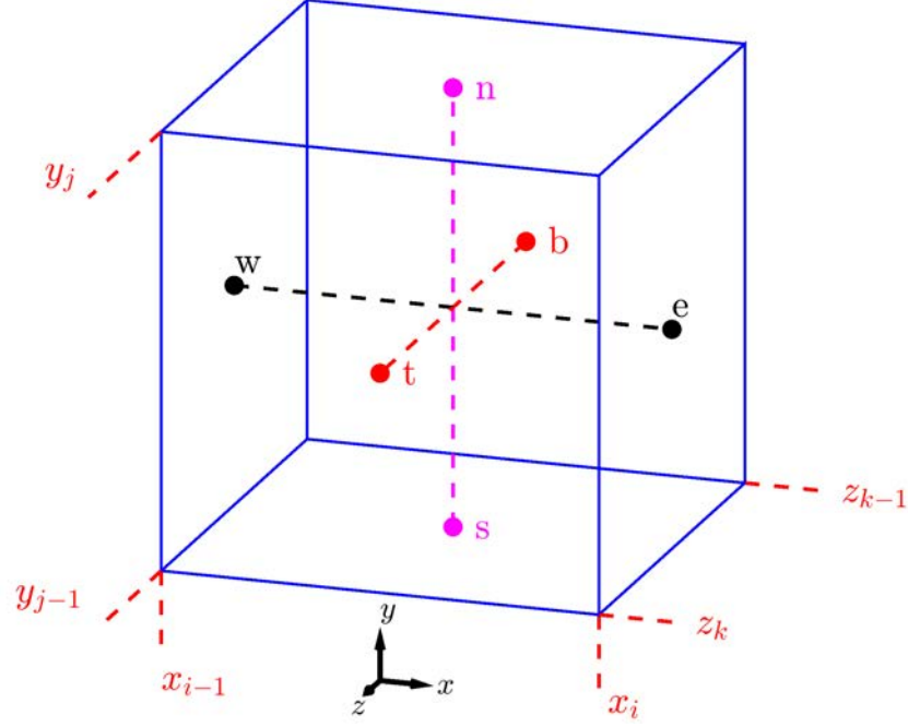
Figure 3.5: The elementary faces of a Cartesian cell denoted with the usual compass notations (w: West, e: East, s: South, n: North, b: Bottom and t: Top).
