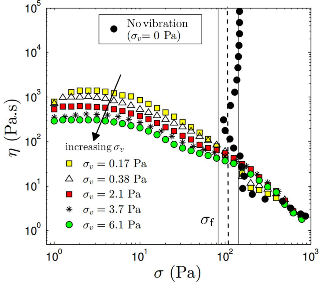
Figure 1.4: Viscosity \eta as a function of the shear stress \sigma for different values of vibration stress \sigma_v for the glass beads of 100\mu m immersed in a Newtonian fluid with the viscosity of \eta_f = 67.8 mPa.s reprinted from Hanotin [46]. The rectangular zone display the estimation of frictional stress \sigma_f .
