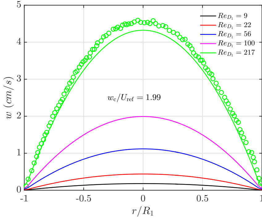
Figure 5.9: Axial velocity profiles of water at z = -9 \text{ mm} for different Reynolds numbers: circles ( \circ ) for experimental data [86] and solid lines (—) for LS-STAG computation. For all Reynolds number the ratio of w/U_{\text{ref}} is equal to 1.99.
