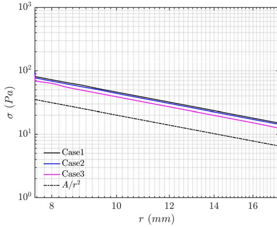
Figure 5.39: The shear stress profile along the annular gap ( r \in [7.5 \text{ } 17.5] \text{ mm} ) for different cases.
