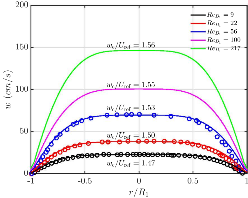
Figure 5.11: Axial velocity profiles of Xanthan 0.3% at z = -9 \text{ mm} for different Reynolds numbers: circles ( \circ ) for experimental data [86] and solid lines (—) for LS-STAG computation.
