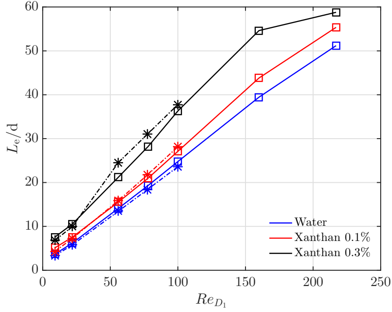
Figure 5.7: Evolution of establishment length with the Reynolds number: LS-STAG (-□-) versus FLUENT ® (-*-*) [86] for three different fluids.
