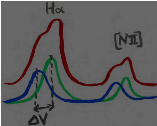
Figure 1.15: Scheme of the blue-shifted component for \text{H}\alpha and [\text{N II}] produced by galactic outflows. The green Gaussian correspond to the systemic (narrow) component and the broad component is shown in blue. The velocity difference (corresponding to the outflow velocity) between the two components is shown by the label \Delta V .
