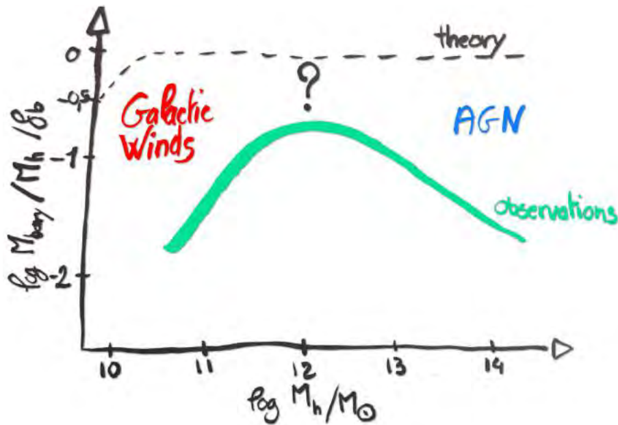
Figure 1: Scheme of the fraction of baryons versus galaxy halo mass. The predicted amount is represented by the dashed black curve whereas the observations are represented by the green one. We can see the two major problems : the global shift between observations and theory as well as the two cutoffs at low and high mass regimes. The two phenomena invoked to explain these cutoffs are Active Galactic Nuclei (AGN in blue) for the high mass regime and galactic winds (in red) for low mass galaxies.
