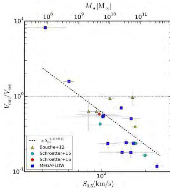
Figure 5.8: V_{\text{out}}/V_{\text{esc}} as a function of S_{0.5} (bottom x-axis) and M_* (top x-axis). Yellow triangles are from Bouché et al. (2012), cyan and red circles are from Schroetter et al. (2015) and Schroetter et al. (2016) respectively. The horizontal line corresponds to V_{\text{out}} = V_{\text{esc}} . The dashed black line corresponds to a fit with coefficients shown in the legend.
