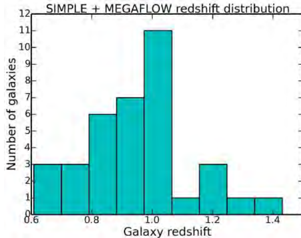
Figure 5.1: Redshift distribution of the 36 galaxies from SIMPLE and MEGAFLOW.
