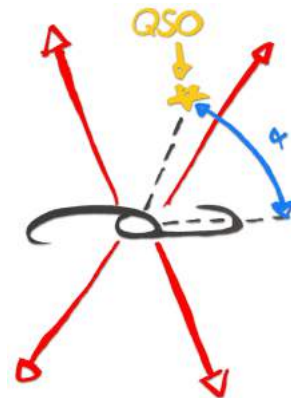
FIG. 1.— Scheme representing the azimuthal angle: The galaxy is represented at the center in black, the red arrows represent the outflowing gas expelled from both side of the galaxy minor axis. The azimuthal angle \alpha is represented by the blue angle between the galaxy major axis and the quasar LOS (in yellow).
