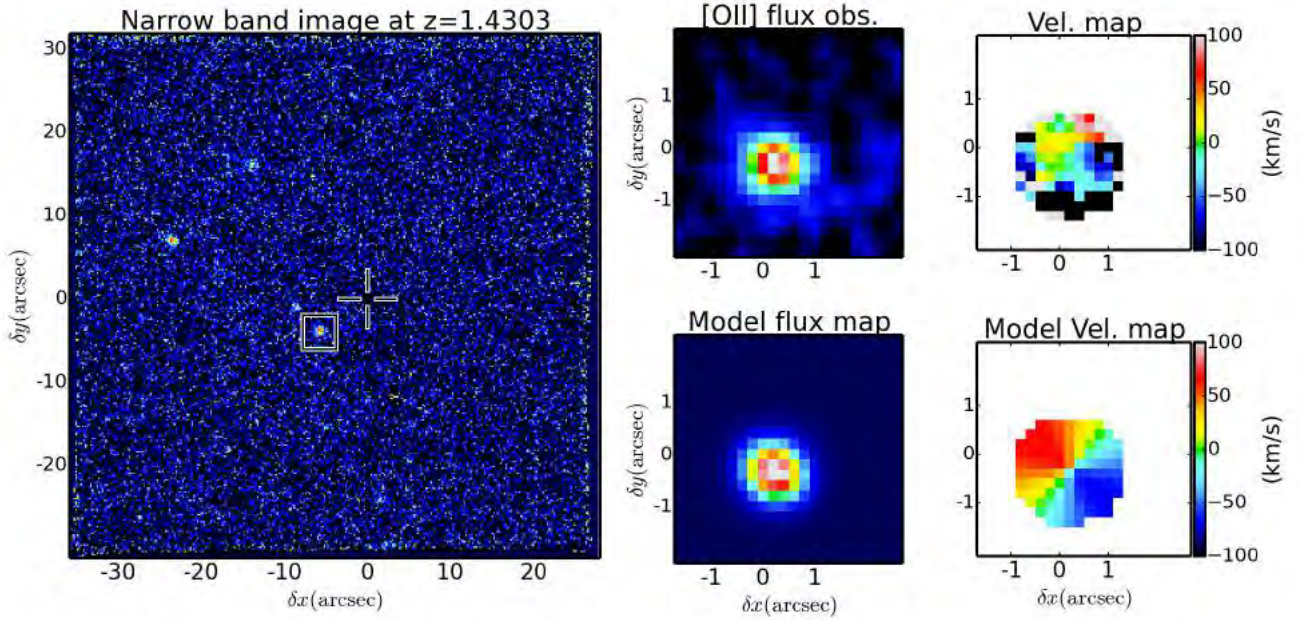
FIG. 7.— Same as Figure 2 but for J215200+0625G3 at redshift z = 1.4303 . Note that the emissions around the galaxy in the observed [O II] flux panel is noise and not tidal tails. This galaxy has a maximum SNR/pixel of 10.5. Again, as in Figures 4 and 5, residual spots are galaxies further away from the quasar LOS and are thus less likely to be the host of the absorbing materials (78, 184 and 211 kpc). The 78 kpc away galaxy is close enough to be considered as an host galaxy but we choose to ignore it based on impact parameter argument.
