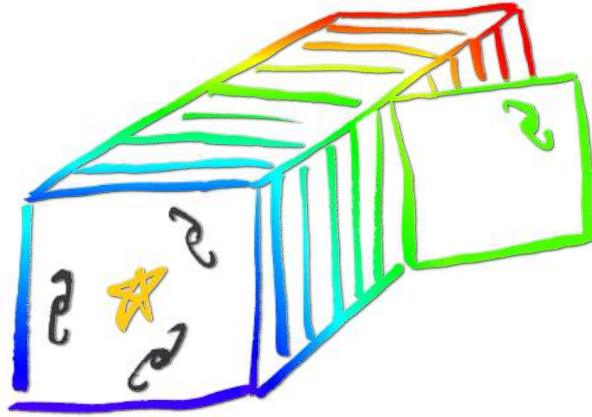
Figure 2.1: Scheme of an 3D IFU cube: the foreground image represents a white-light image of the cube and the extracted image represents a slide of the cube at a given wavelength. On this extracted image one can see only one galaxy which is emitting at the extracted wavelength.
