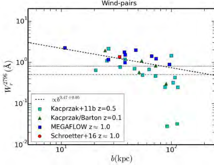
Figure 5.6: Mg II ( \lambda 2796 ) rest equivalent width as a function of impact parameter b for galaxy-quasar pairs classified as wind-pairs. Horizontal dashed black lines show the W_r^{\lambda 2796} > 0.5 \text{ \AA} and W_r^{\lambda 2796} > 0.8 \text{ \AA} selection criteria. The thick black dashed line represents a fit to the data. Fitting coefficients are shown in the legend. Errors on W_r^{\lambda 2796} are typically \sim 10^{-3} \text{ \AA} and \sim 0.5 \text{ kpc} for b .
