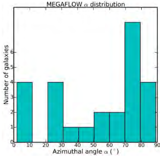
Figure 4.13: Azimuthal angle \alpha distribution for 26 galaxies with reliable morphokinematic parameters detected in the MUSE fields. We note that 11 galaxies are classified as wind-pairs and that there is a bimodal distribution of \alpha . There are more galaxy-quasar pairs in a configuration favorable for wind study.. This is probably due to the fact that we select only strong Mg II REW in the quasar spectra and the largest W_r^{\lambda 2796} tend to be associated with outflows (e.g. Kacprzak et al., 2011; Lan et al., 2014a).
