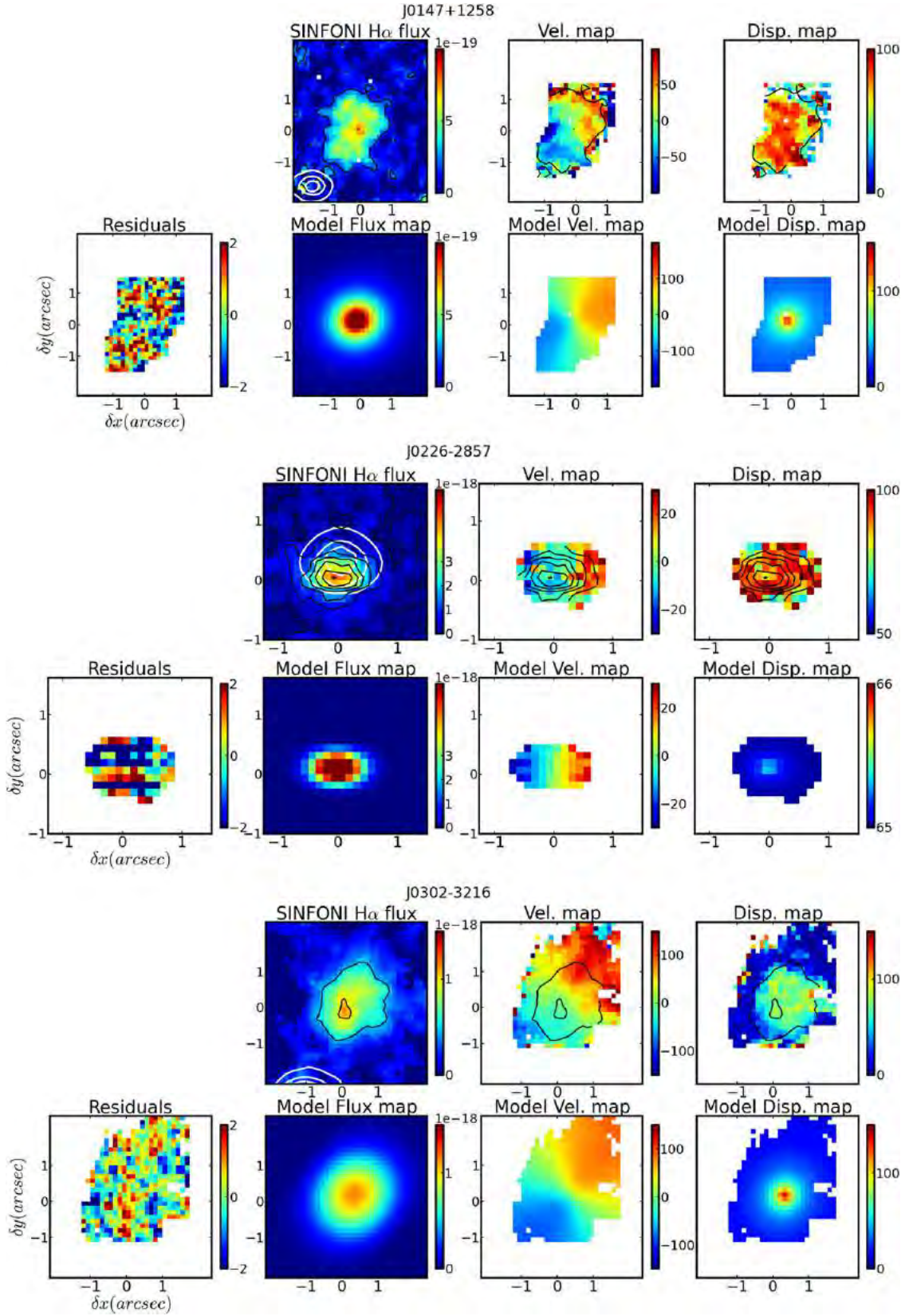
Figure 1. From left to right: top: the HST /WFPC2 image (when available), the H \alpha J -band SINFONI flux ( \text{erg s}^{-1} \text{cm}^{-2} ), the velocity map (in \text{km s}^{-1} ) derived from the SINFONI data, and the dispersion map (in \text{km s}^{-1} ). Bottom: the residuals cube represented in 2D (in \sigma ), the intrinsic reconstructed galaxy with GalPaK 3D (deconvolved from the PSF given by the quasar), its velocity map, and the dispersion map. The quasar position is represented by the white contours on the observed flux maps when present in the map. In each panel, north is up and east is to the left.
