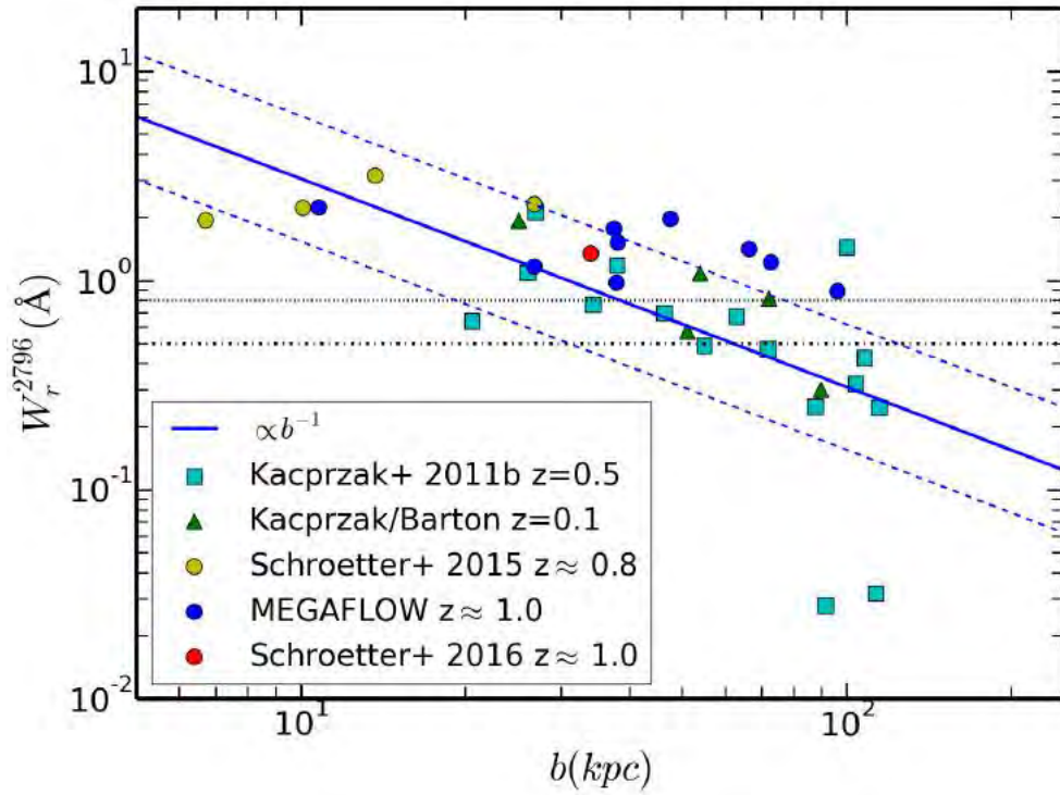
Figure 2.5: W_r^{\lambda^{2796}} as a function of impact parameter b for galaxy-quasar pairs classified as wind-pairs. Horizontal dashed black lines shows the W_r^{\lambda^{2796}} > 0.5\text{\AA} and W_r^{\lambda^{2796}} > 0.8\text{\AA} selection criteria.
