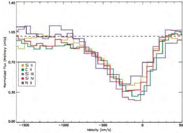
Figure 1.16: Outflow absorption lines seen in a galaxy spectrum from Heckman et al. (2015). This absorption is blue-shifted with respect to the galaxy systemic velocity. We can also see that the different absorption lines have the same absorption behavior like their asymmetry.
