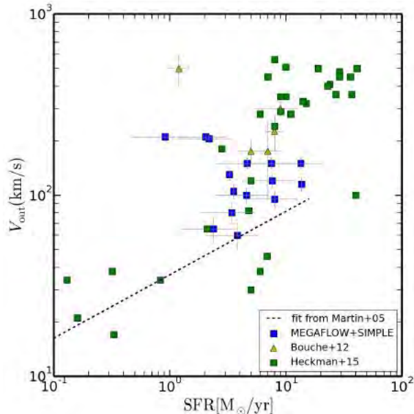
Figure 5.10: V_{\text{out}} as a function of SFR for both surveys (MEGAFLOW and SIMPLE) as well as observations from Bouché et al. (2012) and Heckman et al. (2015). The dashed black line shows a fit ( \log V = (0.35 \pm 0.06) \log(\text{SFR}) + (1.56 \pm 0.13) ) from Martin (2005). Errors on Heckman et al. (2015) observations are 0.2 dex for SFR and 0.05 dex for V_{\text{out}} .
