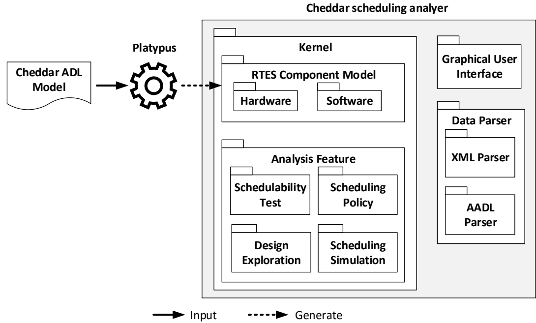
Figure 31: Cheddar Framework
