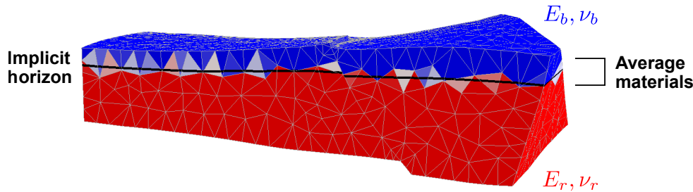
Figure 1.2: Equivalent mechanical properties. Faulted model with an implicit horizon (black thick line). This horizon is the boundary of two layers (red and blue). Average Young's modulus and Poisson's ratio is defined for each tetrahedron crossed by the implicit horizon.
