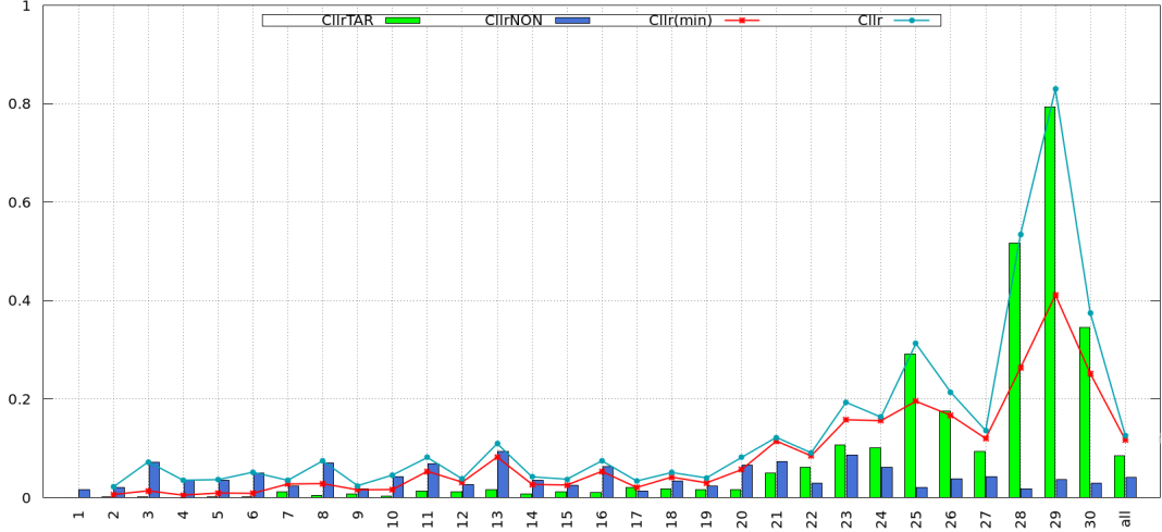
Figure 8.5: C_{llr} , C_{llr}^{min} , C_{llr}^{TAR} , C_{llr}^{NON} per speaker and for “all” (data from all the speakers are pooled together).
