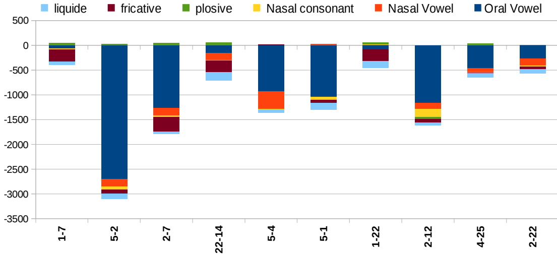
Figure 9.6: Stacked bar chart of relative C_{llr}^{NON} computed on the 10 “best” speaker pairs, spk^i-spj , in term of discrimination power (Averaged C_{llr}^{NON}=5.10^{-5} bits).
