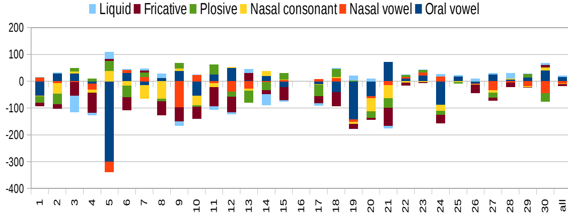
Figure 9.11: Stacked bar chart of C_{lr}^R computed on C_{lr}^{TAR} (target trials) per speaker and for "all". Experiments are performed taking advantage of the full bandwidth (0-8000 Hz).
