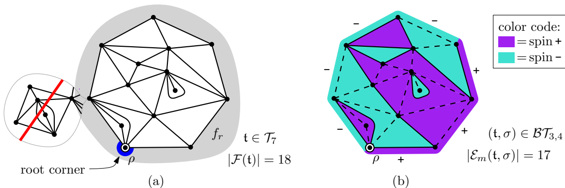
Figure V.1 – (a) a triangulation \mathbf{t} of the 7-gon with 18 internal faces. The boundary will no longer be simple if one attaches to \mathbf{t} the map inside the bubble to its left. (b) a bicolored triangulation of the (3,4)-gon with 17 monochromatic edges (in dashed lines).
