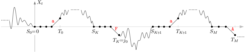
Figure IV.4 – The decomposition of N_0^+ into intervals [S_k, T_k] .
