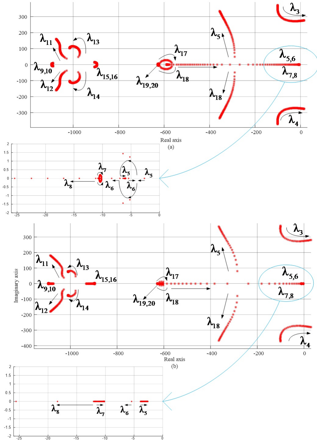
Figure 4.4: Root locus with the variation of parameters in the Droop control: ( K_e = 10\text{sec}^{-1} , K_a = 10\text{sec}^{-1} ). (a) Variation of m_i : 5 \times 10^{-5} \leq m_1 \leq 5 \times 10^{-3} (rad/W.sec), 1 \times 10^{-4} \leq m_2 \leq 1 \times 10^{-2} (rad/W.sec); (b) Variation of n_i : 1.33 \times 10^{-2} \leq n_1 \leq 0.53 (V/Var.sec), 2.67 \times 10^{-2} \leq n_2 \leq 1.06 (V/Var.sec).
