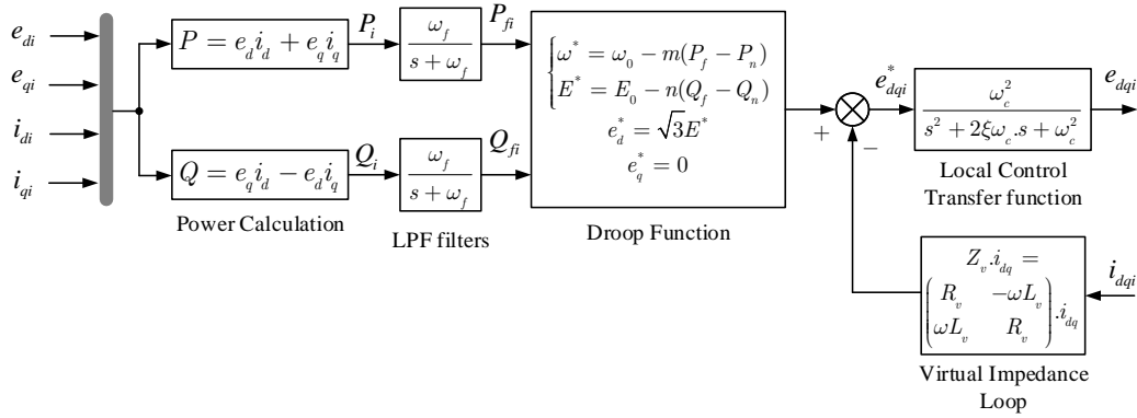
Figure 5.2: Equivalent Block diagram describing the Droop Control in DG_i .
