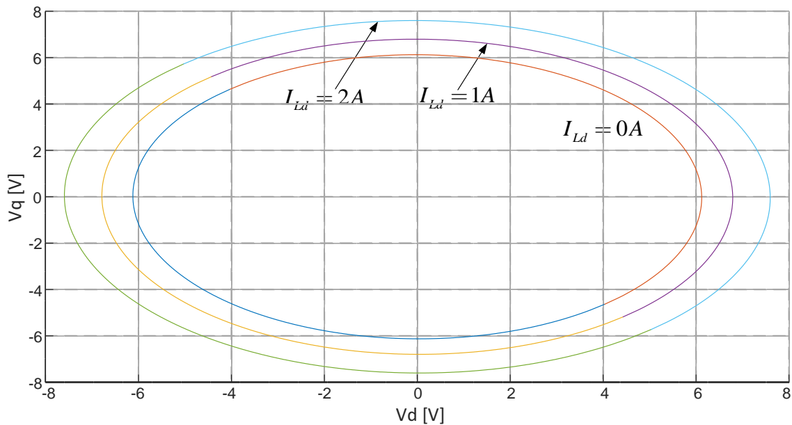
Figure 5.13: Estimated Domain of attraction for the system under the effect of constant current load ( P_c(\text{CPL}) = 600\text{W} , R_{ch} = 100\Omega ).
