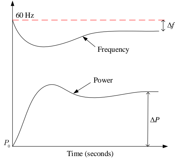
Figure 1.3: Synchronous Generator transient response.
