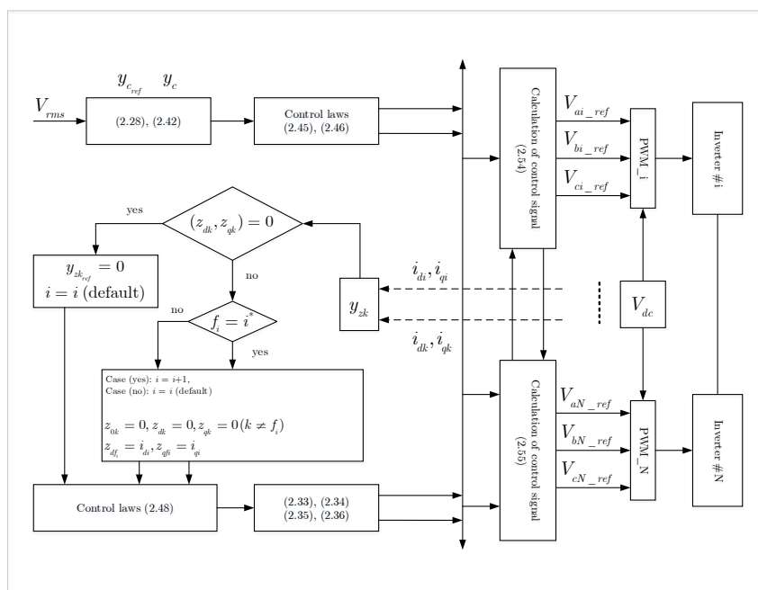
Figure 2.8: Operational block diagram of the proposed control method for N-parallel inverters with the circulating current and balancing method.
