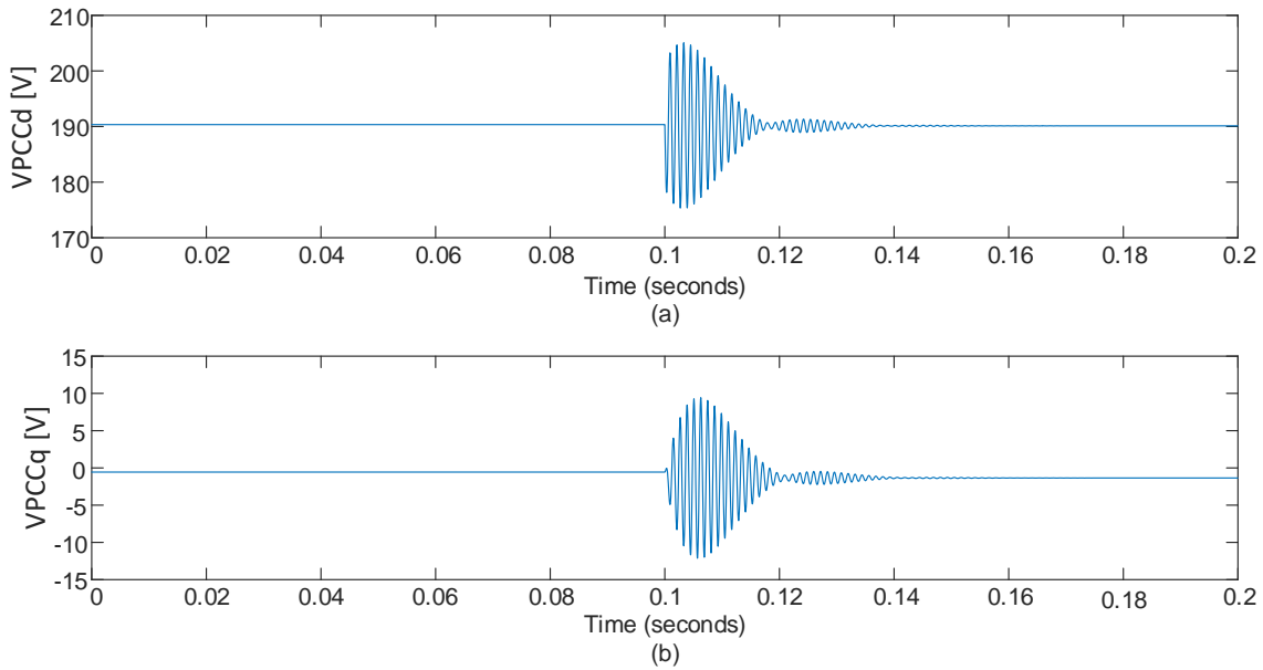
Figure 5.16: PCC dq voltage waveform evolution inside the predicted domain of attraction for CPL load change: P_{CPL} = 200 - 1000W .
