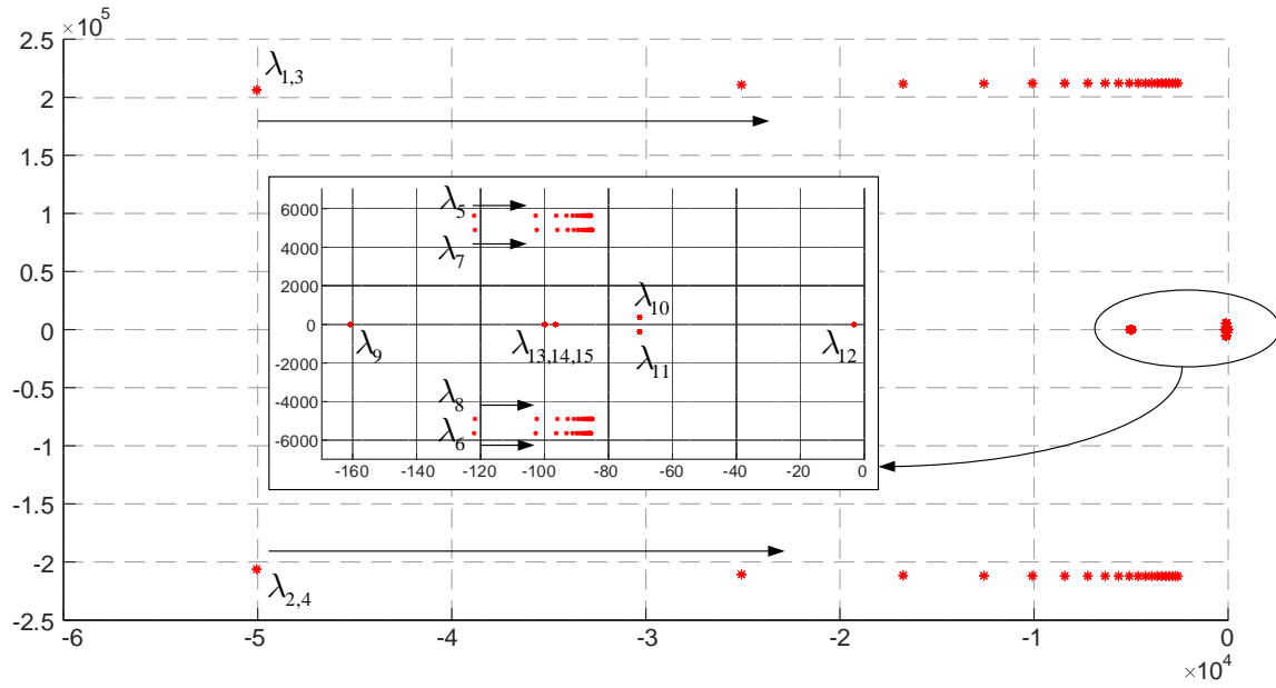
Figure 5.8: Low-frequency eigenvalues as function of R_{ch} load change (increasing): 100 \leq R_{ch} \leq 2000 ( \Omega ).
