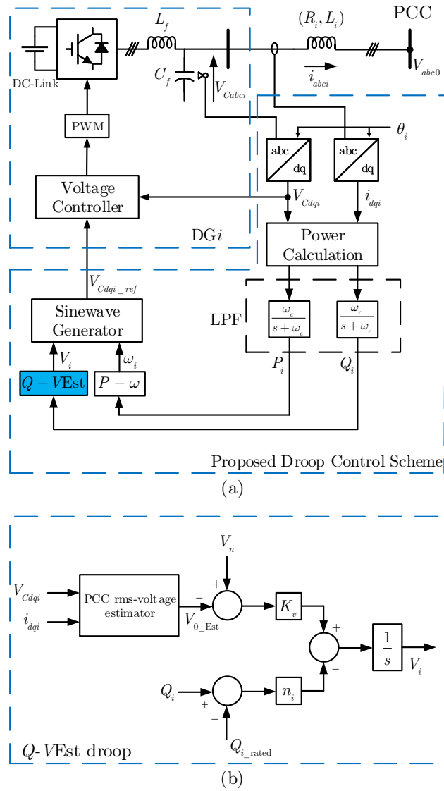
Figure 2.18: Proposed Droop Control scheme with modified Q - V_{Est} Droop.
