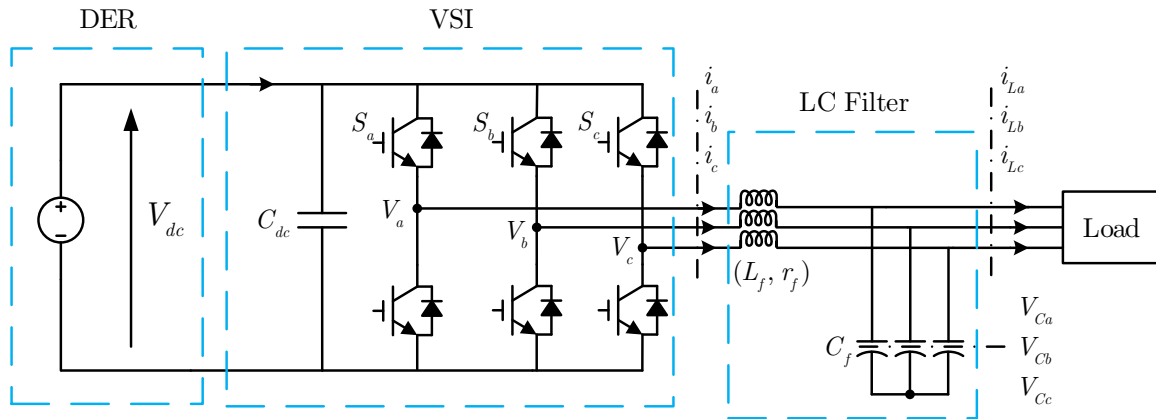
Figure 2.1: Distributed Generator with DER modeled as a DC source.
