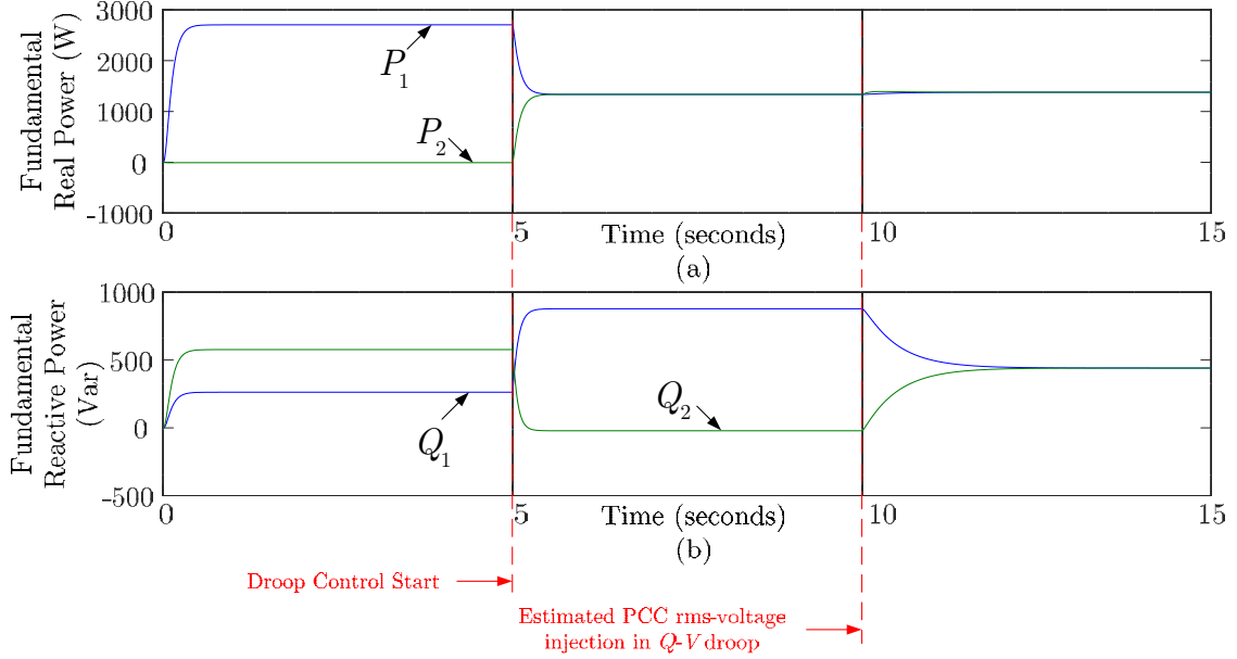
Figure 2.20: Simulation results: (a) Fundamental Real power: P_1 , P_2 ; (b) Fundamental Reactive power: Q_1 , Q_2 before and after the intervention of the estimated PCC rms-voltage.
