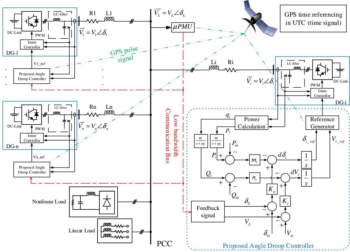
Figure 4.2: Microgrid with Proposed Angle droop control overall block diagram
