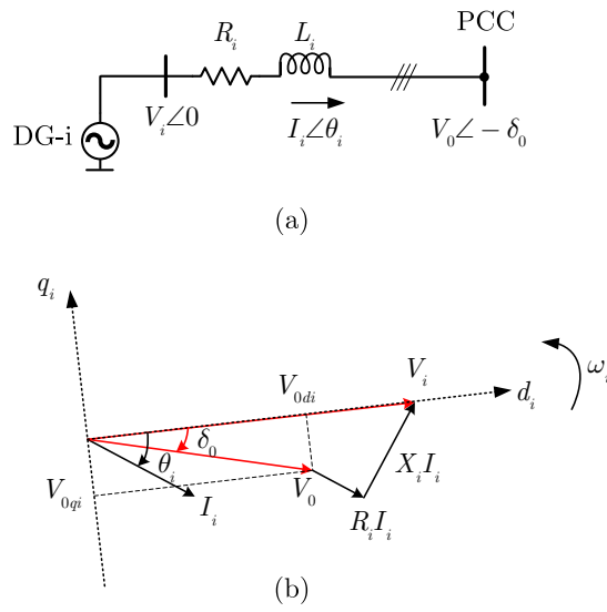
Figure 2.17: Single Line circuit with vector diagram
