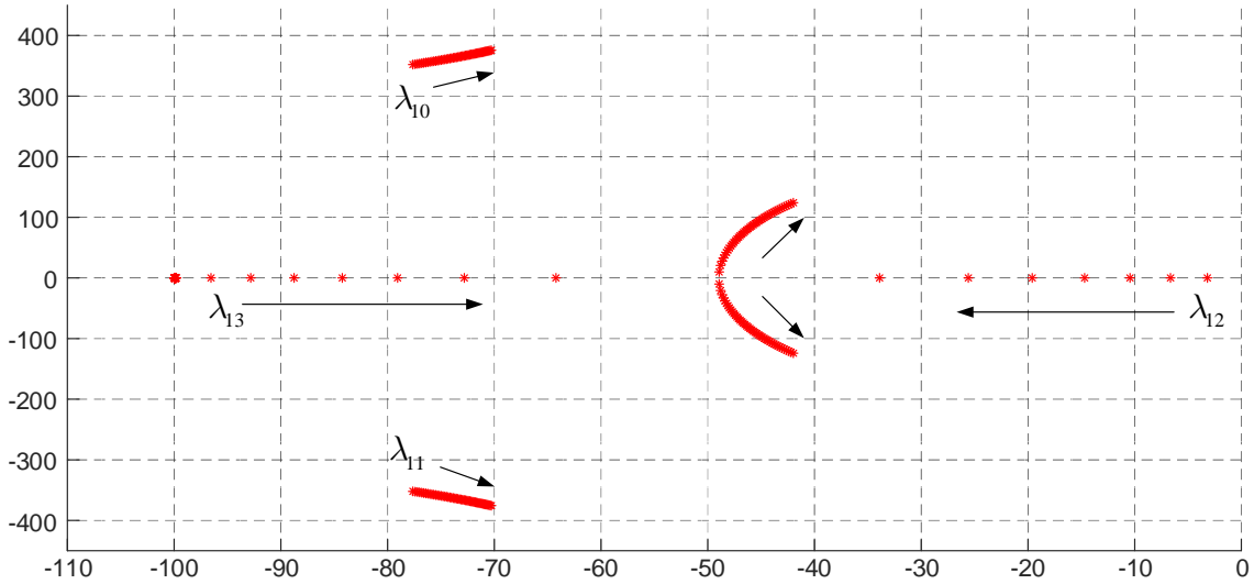
Figure 5.5: Low-frequency eigenvalues as function of frequency drop (increasing variation): 0.1 \leq \Delta\omega \leq 5 (rad/sec).
