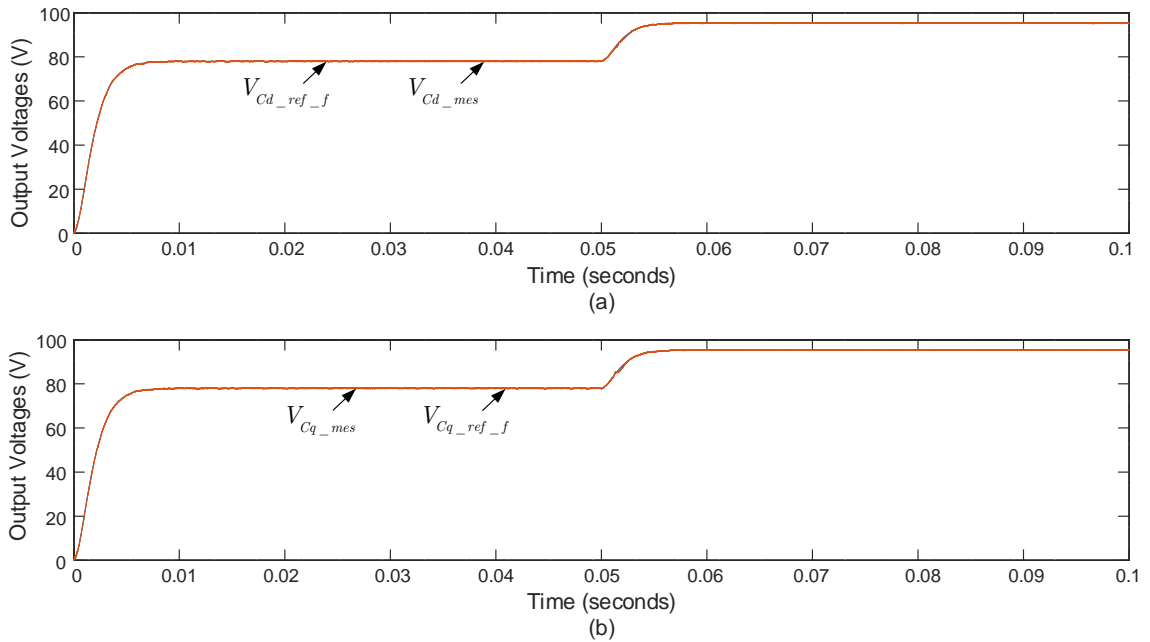
Figure 2.6: dq output voltages of parallel system under the proposed control method. (a) Voltage V_{cd} , (b) Voltage V_{cq} from the startup to a step in V_{rms} voltage at t = 50\text{ms} from 90 to 110V.
