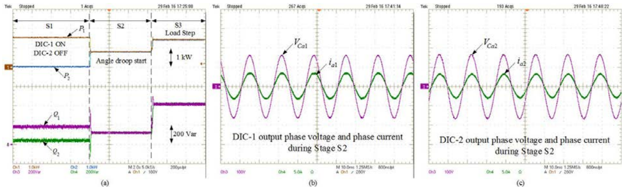
Figure 4.15: Experimental results of case 1: (a) real and reactive power sharing between two converters; (b) phase voltage and phase current for DIC-1; (c) phase voltage and phase current for DIC-2.
