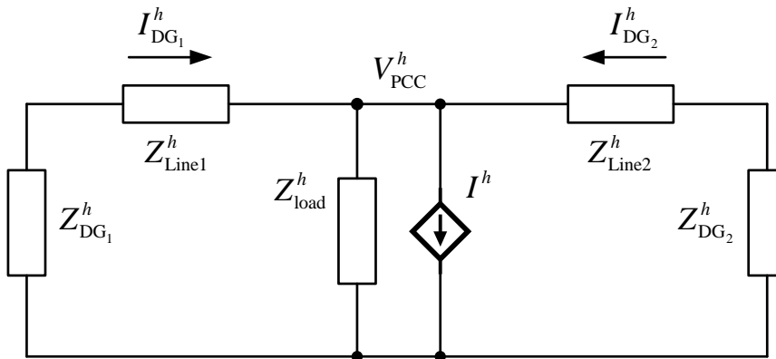
Figure 3.2: Equivalent circuit of two DGs at harmonic frequencies.
