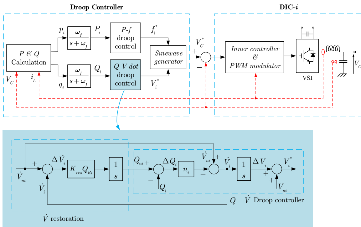
Figure 1.13: Q - \dot{V} droop Controller and the overall control block diagram of DIC- i .
