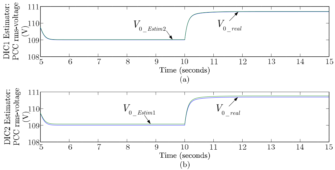
Figure 2.21: Simulation results: (a) DG1 state Estimator PCC rms-voltage compared to real value; (b) DG2 state Estimator PCC rms-voltage compared to real value.
