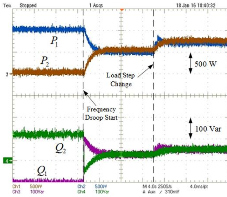
Figure 3.21: Experimental results for case 1: (a) Fundamental Real power: P_1 , P_2 and Fundamental Reactive power: Q_1 , Q_2 under different stages.
