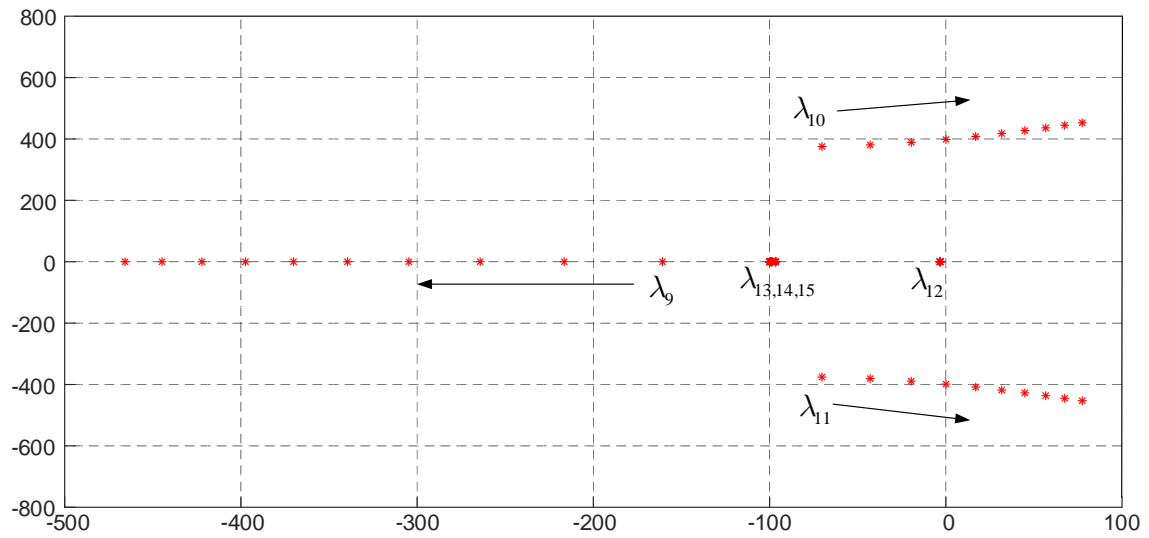
Figure 5.6: Low-frequency eigenvalues as function of voltage drop (increasing variation): 1 \leq \Delta V \leq 10 (V).
