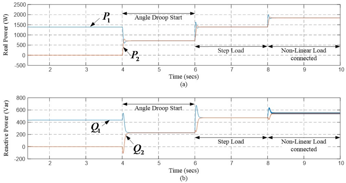
Figure 4.6: Simulation results for Microgrid with two DGs. (a) Real power: P_1 , P_2 ; (b) Reactive power: Q_1 , Q_2 .
