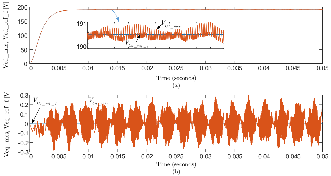
Figure 2.3: Behavior of the Flat outputs ( V_{cd}, V_{cq} ) at starting phase.
