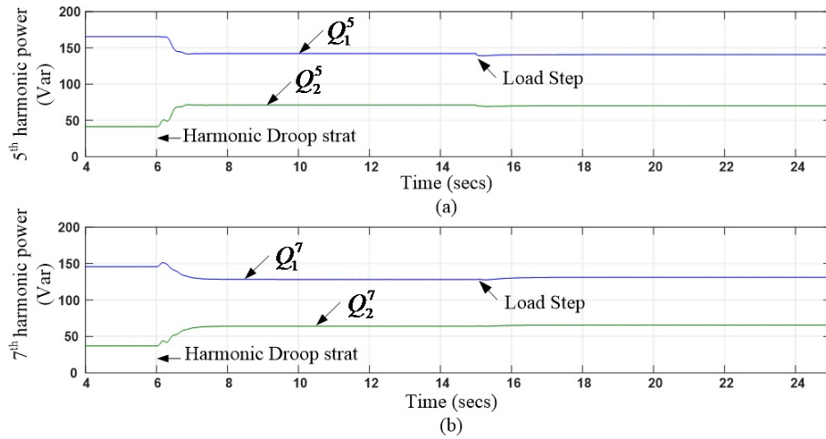
Figure 3.10: Simulation results for case 2. (a) 5th Harmonic power for two DGs: Q_1^5 , Q_2^5 ; (b) 7th Harmonic power for two DGs: Q_1^7 , Q_2^7 .
