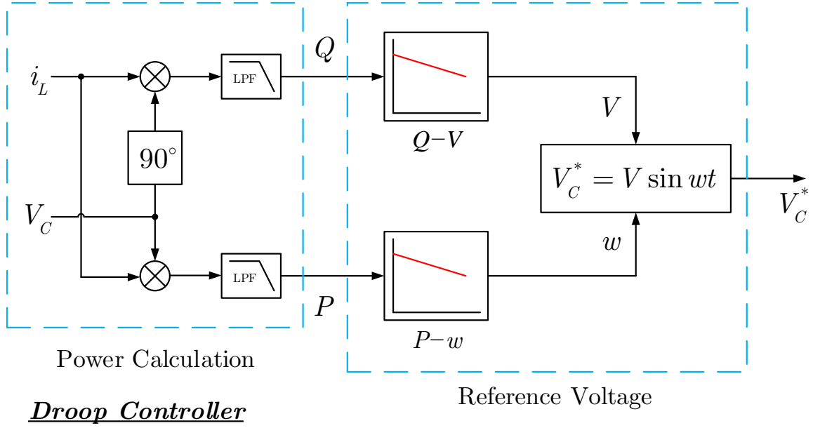
Figure 1.6: Droop Controller Block Diagram.
