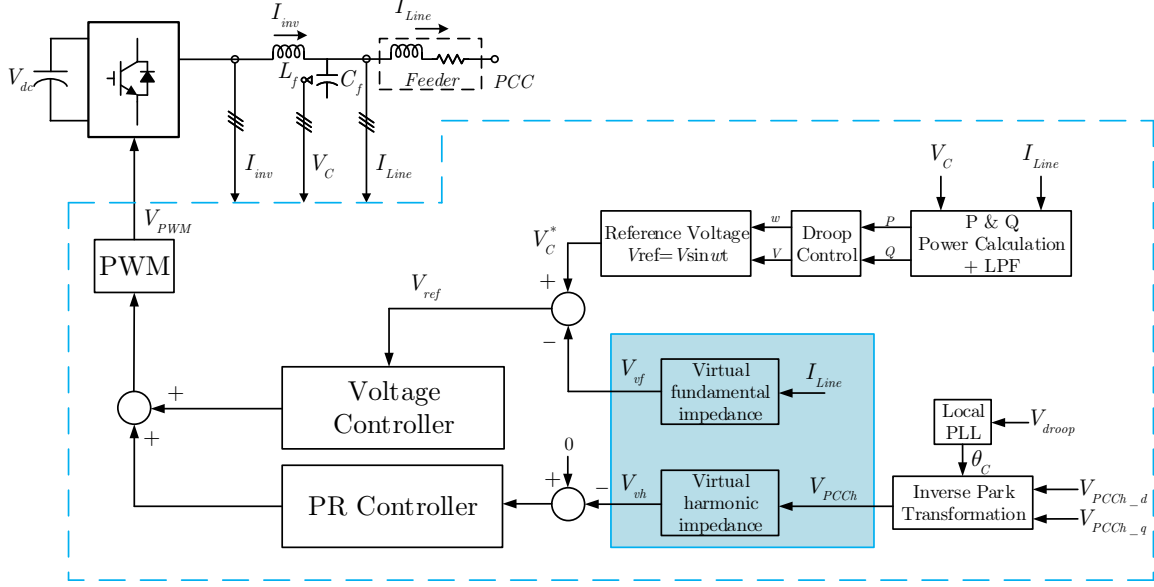
Figure 1.9: Droop Control with enhanced virtual impedance.
