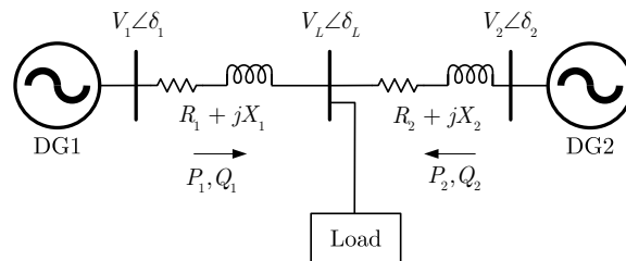
Figure 2.19: Simplified circuit of the system.
