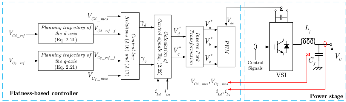
Figure 2.2: Functional diagram of the proposed Control.
