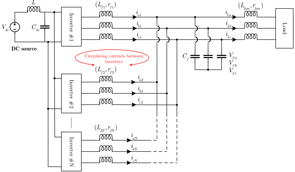
Figure 2.5: System with N -parallel inverters.
