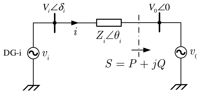
Figure 1.4: Distributed Generator Delivering power to infinite bus through impedance \bar{Z}_i .
