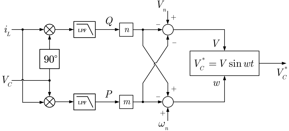
Figure 1.7: Droop Control for complex line impedance.
