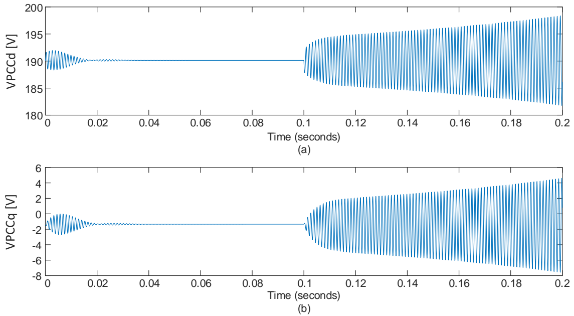
Figure 5.17: PCC dq voltage waveforms evolution outside the predicted domain of attraction for CPL load change: P_{CPL} = 1000 - 1150W .
