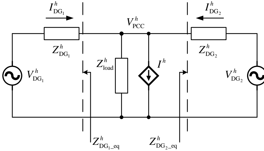
Figure 3.3: Simplified Equivalent circuit of two DGs based microgrid.
