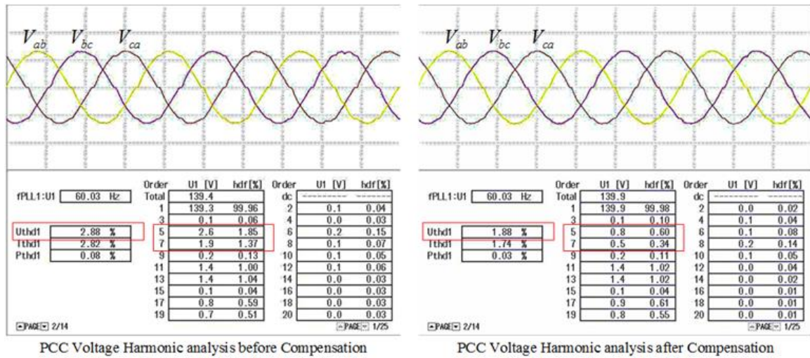
Figure 3.25: Experimental results: PCC phase-to-phase voltages with harmonic analysis before and after compensation.
