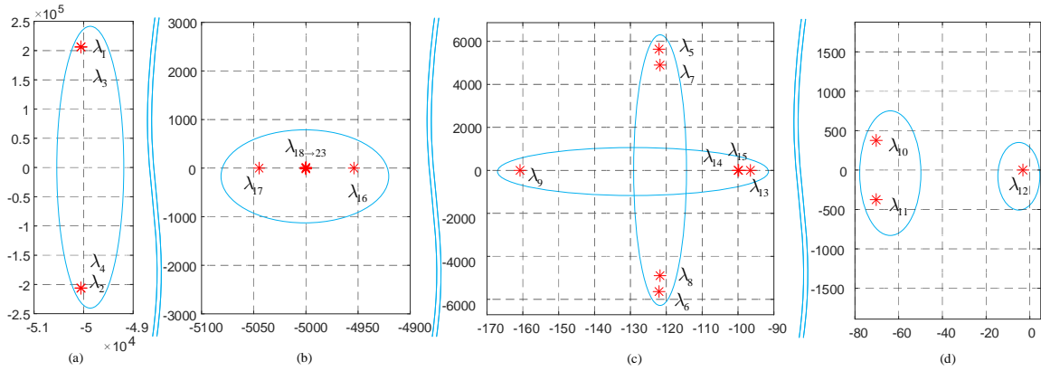
Figure 5.4: Eigenvalues spectrum of the system indicating different clusters.
