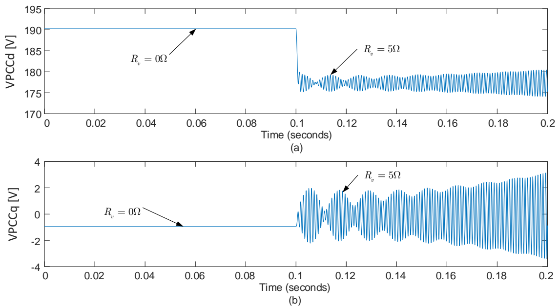
Figure 5.18: PCC dq voltage waveforms evolution inside/outside the predicted domain of attraction for virtual resistance: R_v = 0 - 5\Omega .
