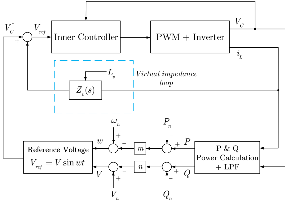
Figure 1.8: Droop Control overall scheme with virtual output impedance.
