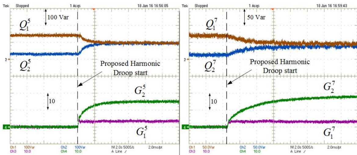
Figure 3.22: Experimental results for case 1: 5th and 7th Harmonic power distribution with gain time response for both DGs.
