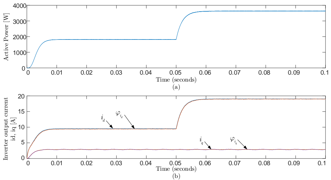
Figure 2.4: Current response during a load transient change from 800 to 3600W.
