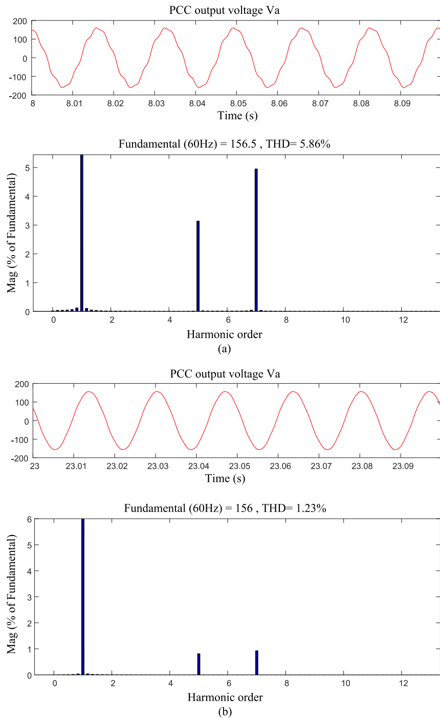
Figure 3.17: Simulation results for microgrid with three DGs: (a) Steady state PCC phase voltage and Harmonic analysis before starting the Harmonic droop: (b) PCC phase voltage and Harmonic analysis after starting the Harmonic droop.
