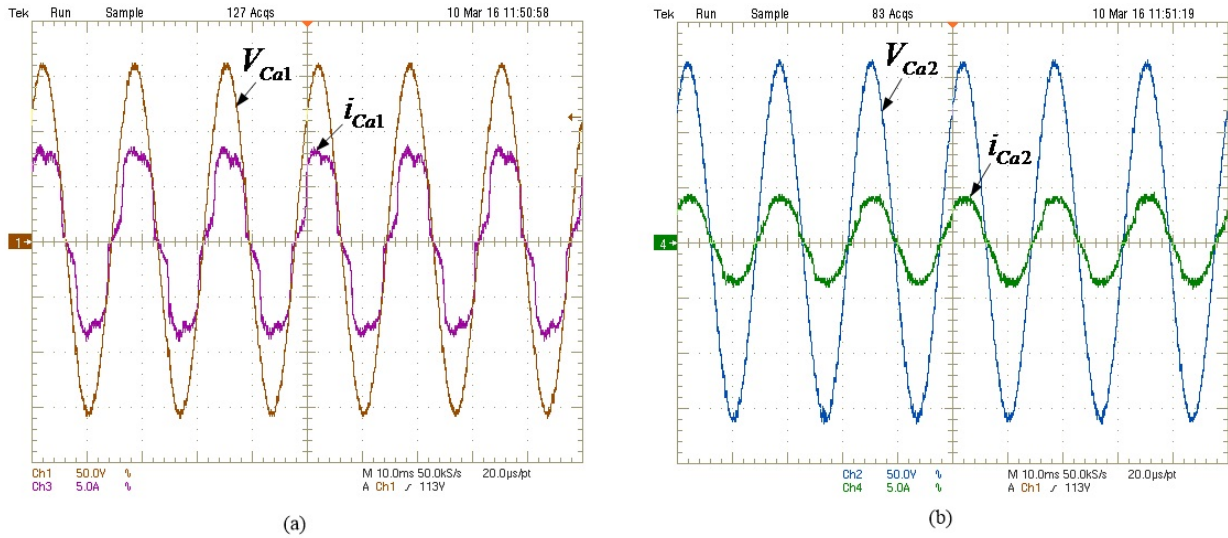
Figure 2.26: Experimental results for Case 2: (a) phase voltage and phase current for DG1; (b) phase voltage and phase current for DG2.
