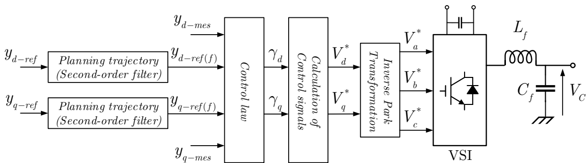
Figure 1.2: Flatness Control Functional Diagram.
