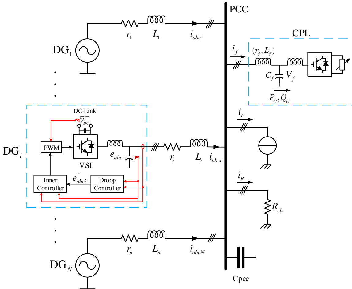
Figure 5.1: Simplified Diagram of the Microgrid system under study.
