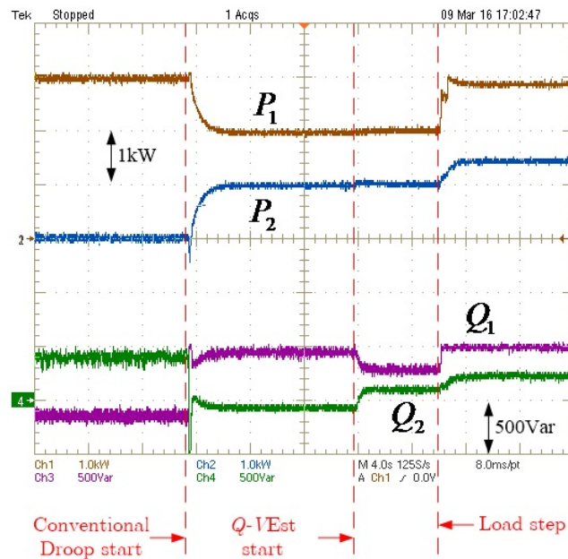
Figure 2.25: Experimental results for Case 2: Fundamental Real power: P_1 , P_2 ; Fundamental Reactive power: Q_1 , Q_2 before and after the intervention of the estimated PCC rms-voltage.
