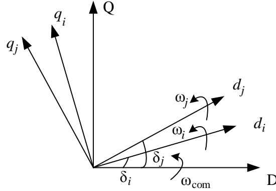
Figure 5.3: Reference Frame Transformation.
