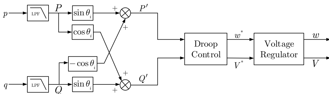
Figure 1.10: Virtual Power Droop Control Block diagram.
