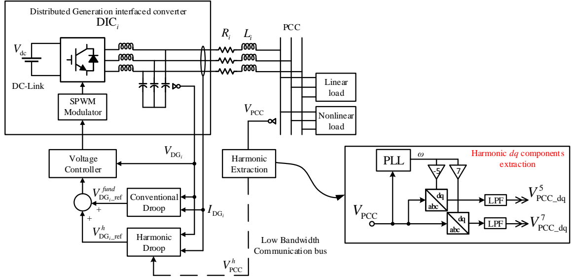
Figure 3.4: Proposed control strategy for DG interfaced converter.
