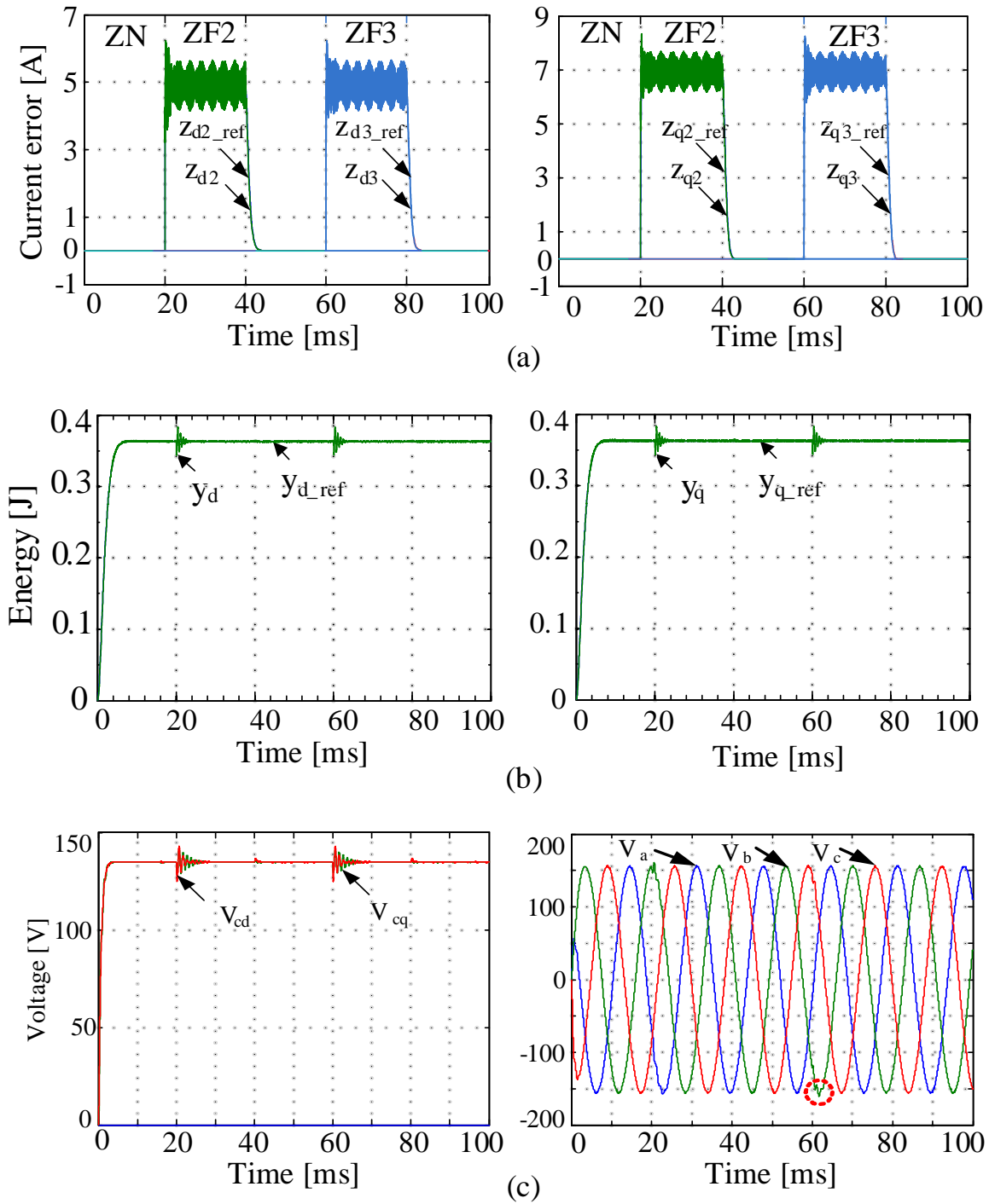
Figure 2.11: Behavior of the parallel inverters system under the proposed control method ( V_{dc} = 500V , V_{rms} = 110V , P_{load} = 3.2kW ). (a) Behavior of current error during healthy and faulty conditions. (b) Behavior of electrostatic energies y_d, y_q under the proposed current balancing method with minimal perturbation. (c) Behavior of V_{cd}, V_{cq} and the output three phase voltages in different zones.
