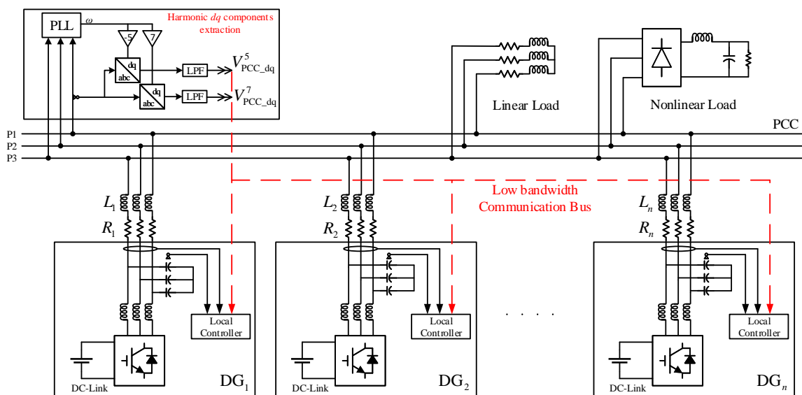
Figure 3.1: Three-phase microgrid with parallel DGs, Linear and nonlinear loads.
