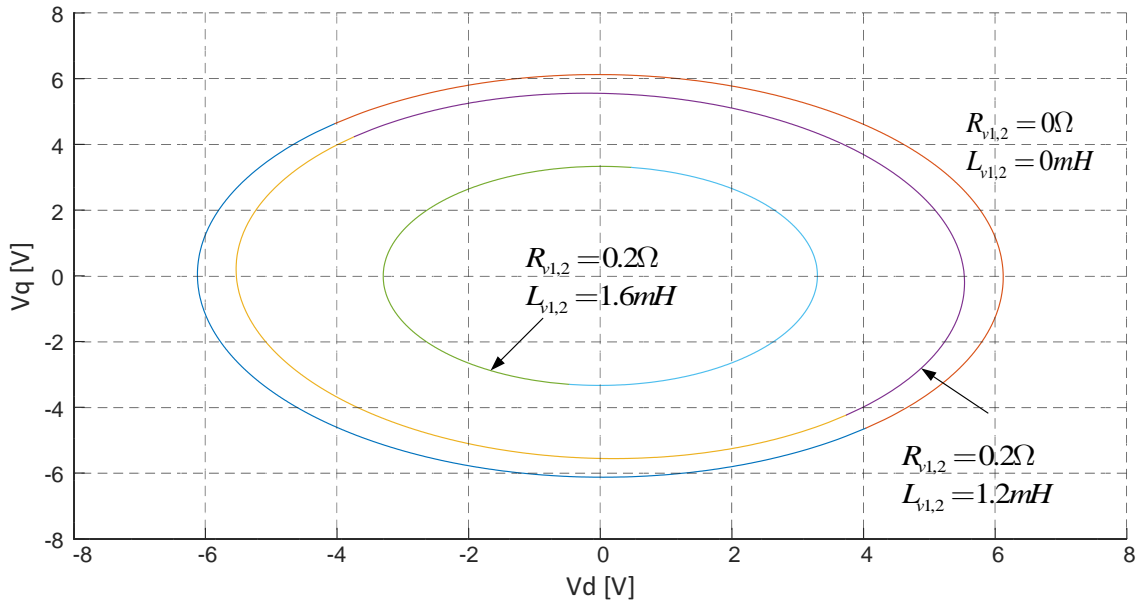
Figure 5.15: Effect of virtual inductance L_v on the estimated domain of asymptotic stability when the bandwidth of inverters controller ( \omega_c = 5000 rad/sec) is lower than the cutoff frequency of the CPL input filter ( \omega_f = 8000 rad/sec). Load condition: P_c(\text{CPL}) = 600\text{W} , I_{Ld} = 0 , I_{Lq} = -3\text{A} , R_{ch} = 100\Omega .
