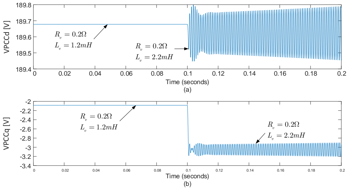
Figure 5.19: PCC dq voltage waveforms evolution inside/outside the predicted domain of attraction for virtual resistance: L_v = 1.2 - 2.2mH .
