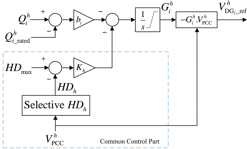
Figure 3.5: Proposed Harmonic Droop Controller.
