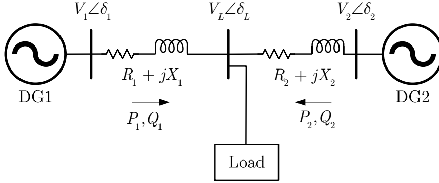
Figure 4.1: Simplified circuit of the system
