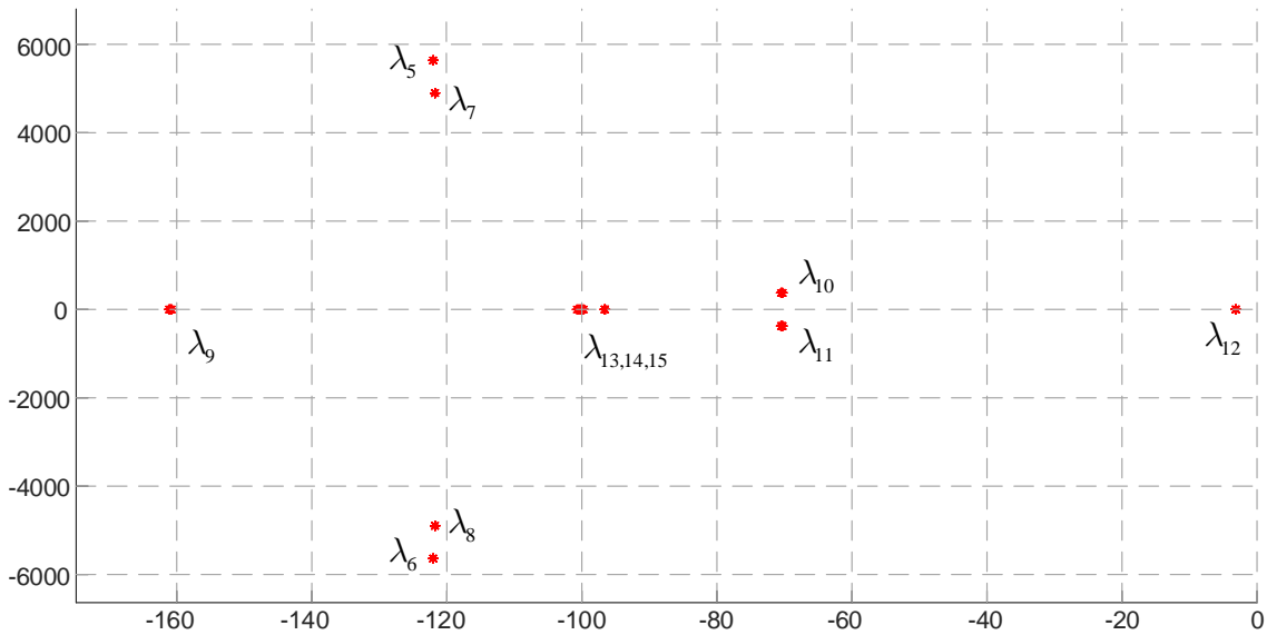
Figure 5.9: Low-frequency eigenvalues as function of I_{Lq} current source load change (increasing): 0 \leq I_{Lq} \leq 20 (A).
