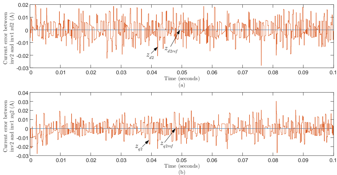
Figure 2.7: dq current error between inverter 1 and 2 under the proposed control method. (a) current error z_{d2} , (b) current error z_{q2} .
