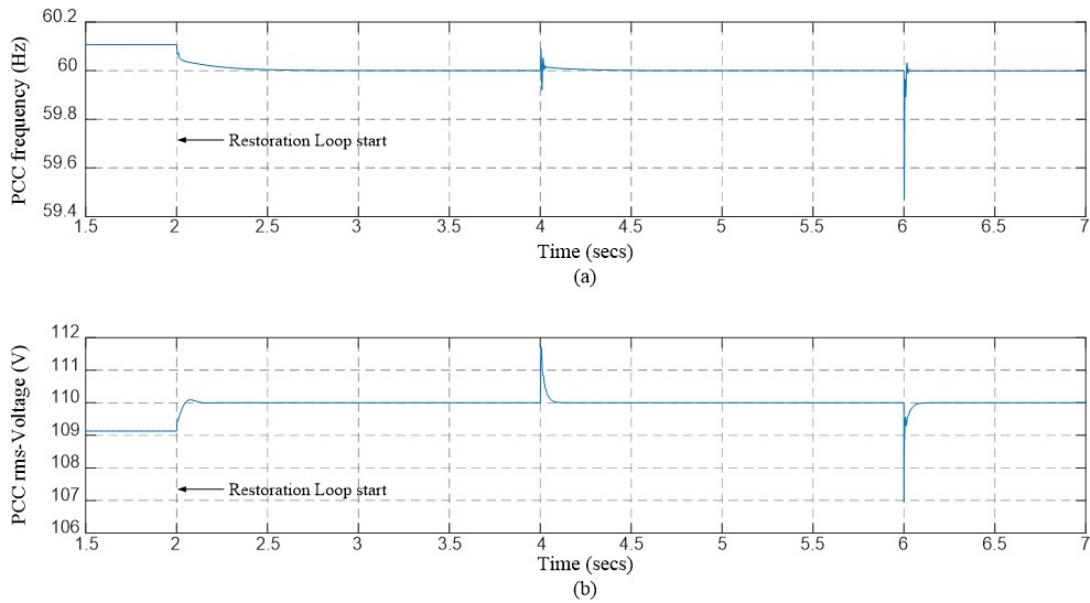
Figure 4.12: Simulation results for Microgrid with three DGs using Hierarchical Droop. (a) PCC frequency (Hz); (b) PCC rms-Voltage (V).
