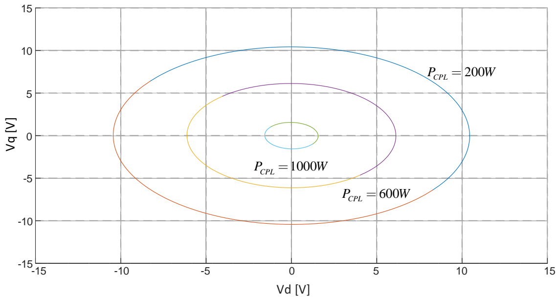
Figure 5.11: Estimated Domain of attraction for the system under the effect of CPL active power ( R_{ch} = 100\Omega , I_{Ld} = 0 , I_{Lq} = -3A ).
