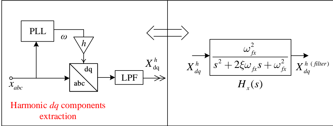
Figure 3.6: Synchronous individual harmonic “ dq frame” extraction block.
