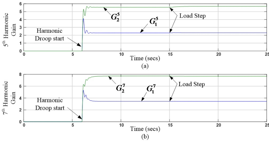
Figure 3.11: Simulation results for case 2. (a) 5th Harmonic Gains for two DGs: G_1^5 , G_2^5 ; (b) 7th Harmonic Gains for two DGs: G_1^7 , G_2^7 .
