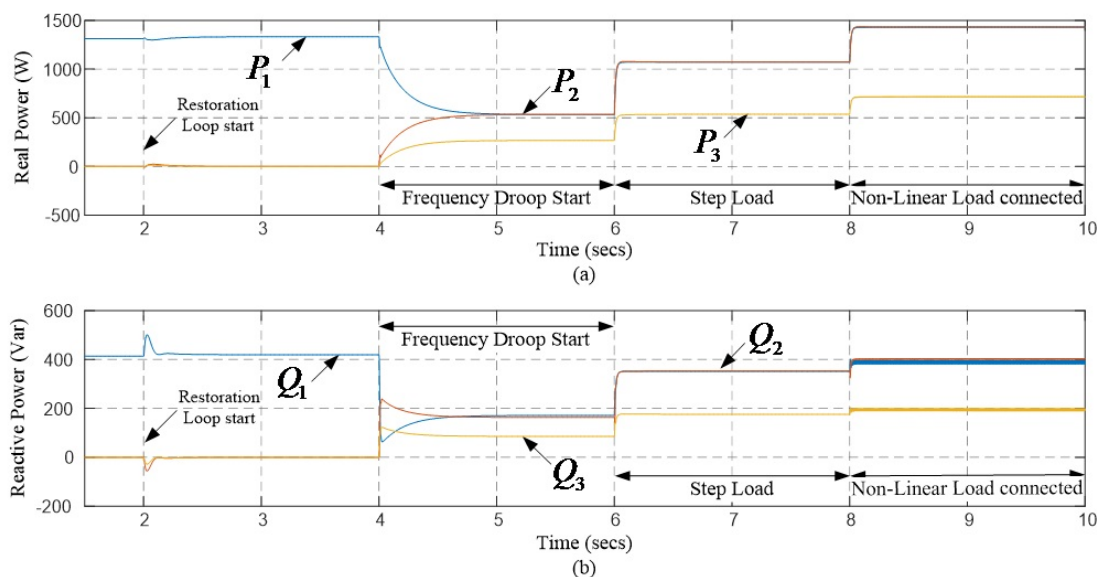
Figure 4.11: Simulation results for Microgrid with three DGs using Hierarchical Droop. (a) Real power: P_1 , P_2 and P_3 ; (b) Reactive power: Q_1 , Q_2 and Q_3 .
