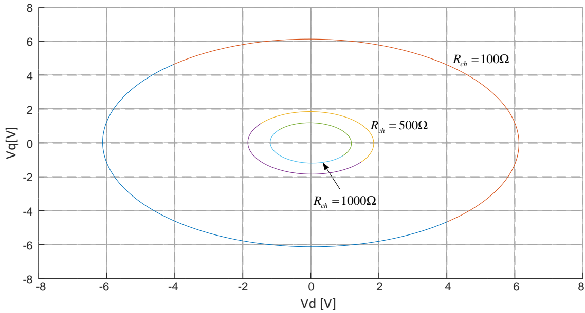
Figure 5.12: Estimated Domain of attraction for the system under the effect of Resistive Load, R_{ch} ( P_c(\text{CPL}) = 600\text{W} , I_{Ld} = 0 , I_{Lq} = -3\text{A} ).
