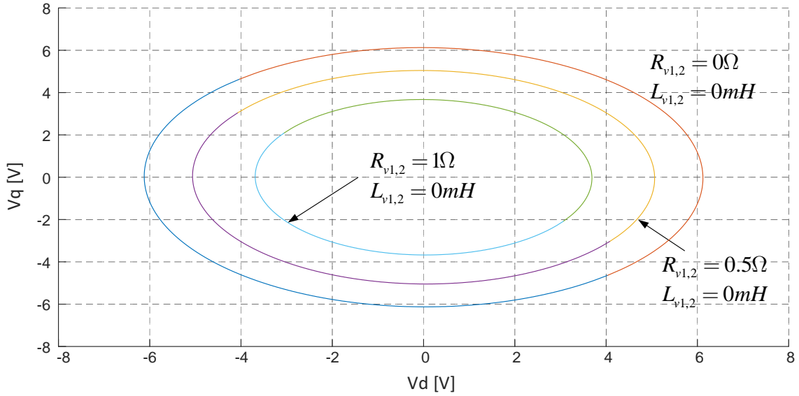
Figure 5.14: Effect of virtual resistance R_v on the estimated domain of asymptotic stability when the bandwidth of inverters controller ( \omega_c = 5000 rad/sec) is lower than the cutoff frequency of the CPL input filter ( \omega_f = 8000 rad/sec). Load condition: P_c(\text{CPL}) = 600\text{W} , I_{Ld} = 0 , I_{Lq} = -3\text{A} , R_{ch} = 100\Omega .
