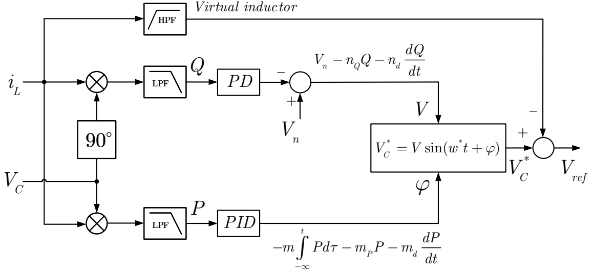
Figure 1.11: Additional control loop Droop Controller.
