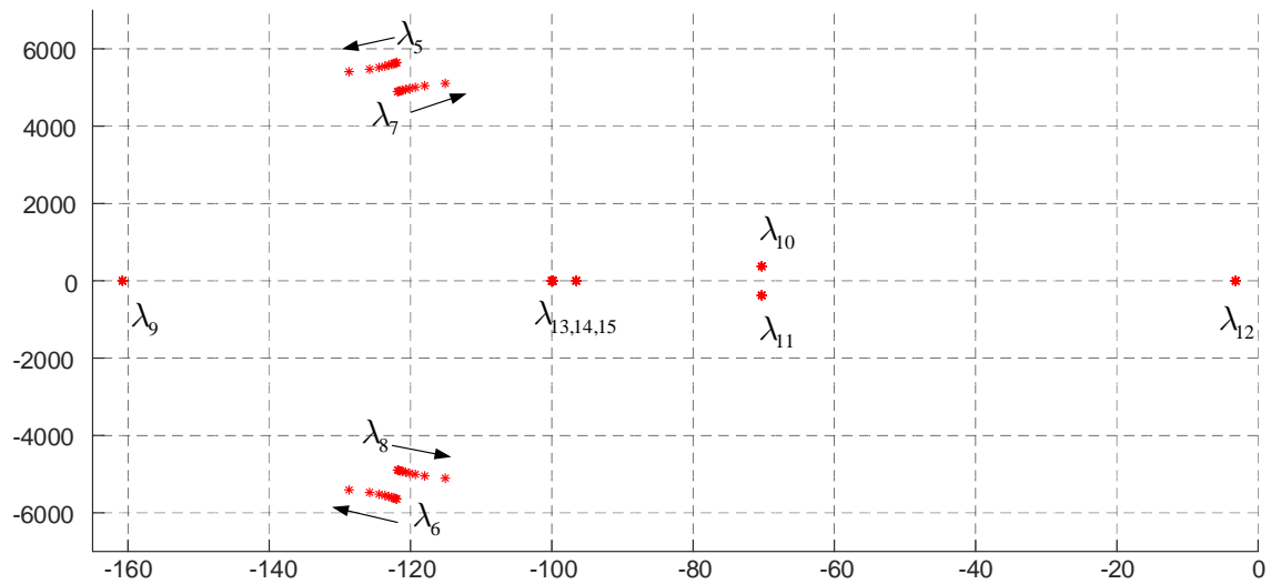
Figure 5.7: Low-frequency eigenvalues as function of CPL real power (increasing): 100 \leq P_c \leq 1000 (W).
