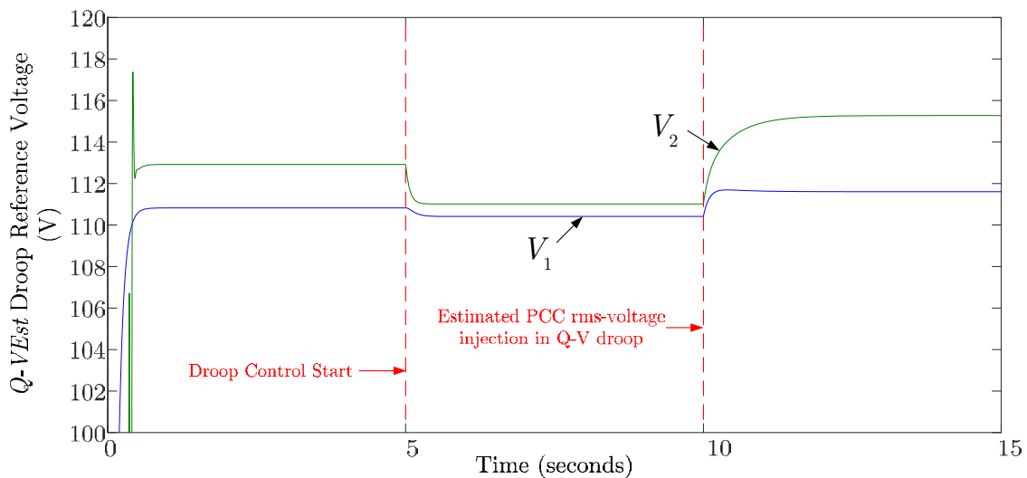
Figure 2.22: Q - V_{Est} Droop Reference voltage variation before and after the injection of the estimated PCC rms-voltage.
