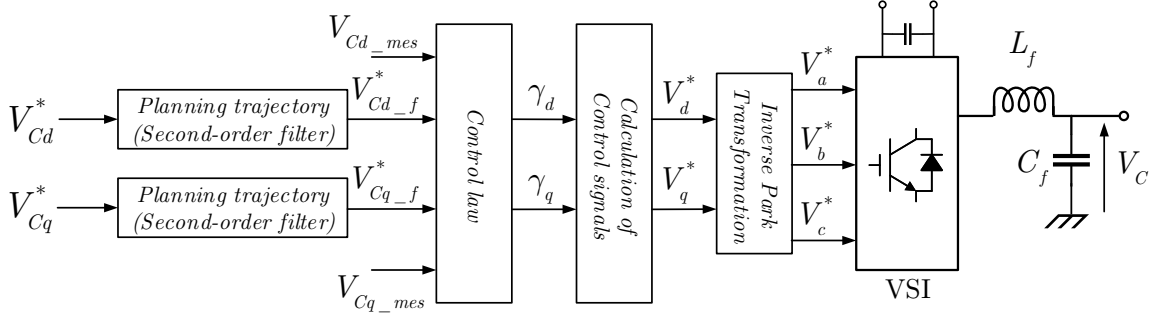
Figure 4.3: Flatness-based Control Functional Diagram.
