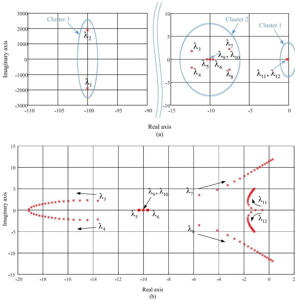
Figure 3.7: Eigenvalue analysis: (a) Eigenvalues for nominal condition ( b_0=10 ): b_1 = 2 \times 10^{-2} , b_2 = 4 \times 10^{-2} ; (b) Eigenvalues locus with harmonic droop coefficients change b_i ( 0 \leq b_0 \leq 170 ): 2 \times 10^{-2} \leq b_1 \leq 3.4 \times 10^{-1} , 4 \times 10^{-2} \leq b_2 \leq 6.8 \times 10^{-1} .
