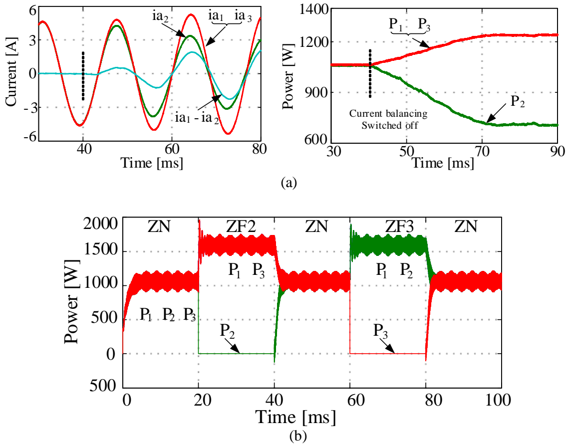
Figure 2.10: Behavior of the parallel inverters system under the proposed control method ( V_{dc} = 500V , V_{rms} = 110V , P_{load} = 3.2kW ). (a) Line currents and power sharing between parallel inverters when the current balancing controller is switched OFF. (b) Load power sharing between parallel inverters for a load of 3.2 kW during healthy and faulty conditions for each inverter with the proposed current balancing method.
