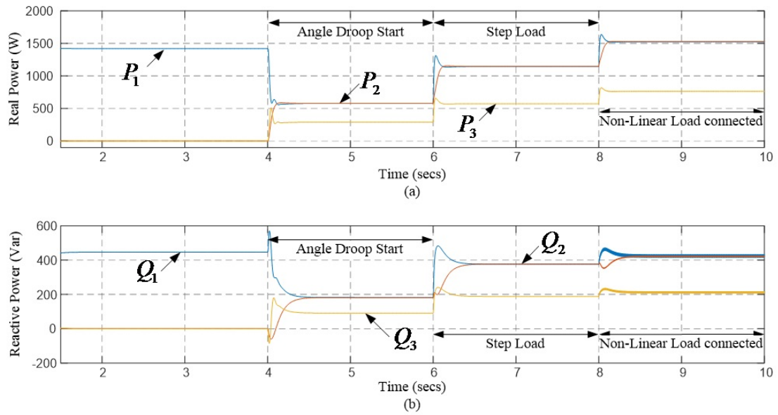
Figure 4.9: Simulation results for Microgrid with three DGs. (a) Real power: P_1 , P_2 and P_3 ; (b) Reactive power: Q_1 , Q_2 and Q_3 .
