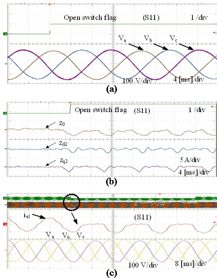
Figure 2.16: Experimental results: (a) waveforms of output ac bus voltages, (b) current errors and (c) output currents under open-switch fault.
