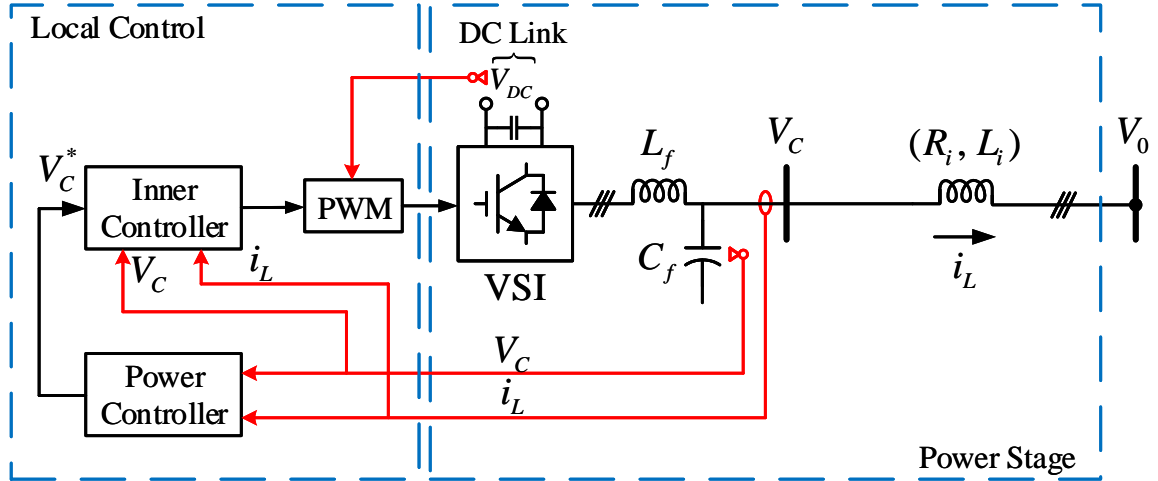
Figure 1.1: Interfaced Converter Control Block Diagram.
