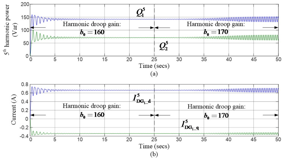
Figure 3.12: Simulation results for system stability: 5th Harmonic power distribution for both DGs with DG 1 harmonic current time response.
