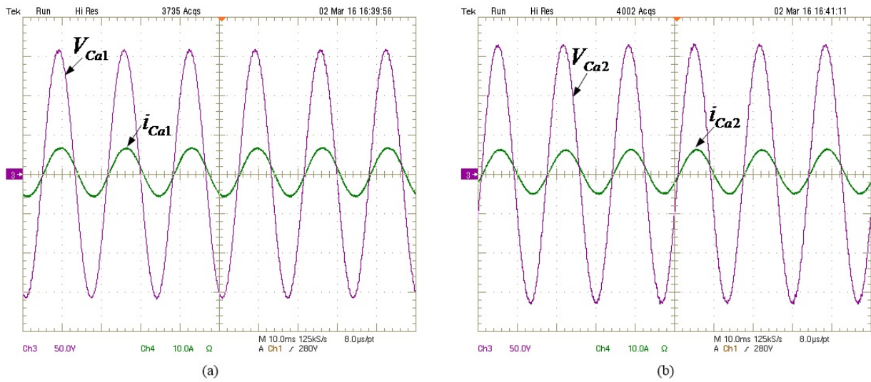
Figure 2.24: Experimental results for Case 1: (a) phase voltage and phase current for DG1; (b) phase voltage and phase current for DG2.
