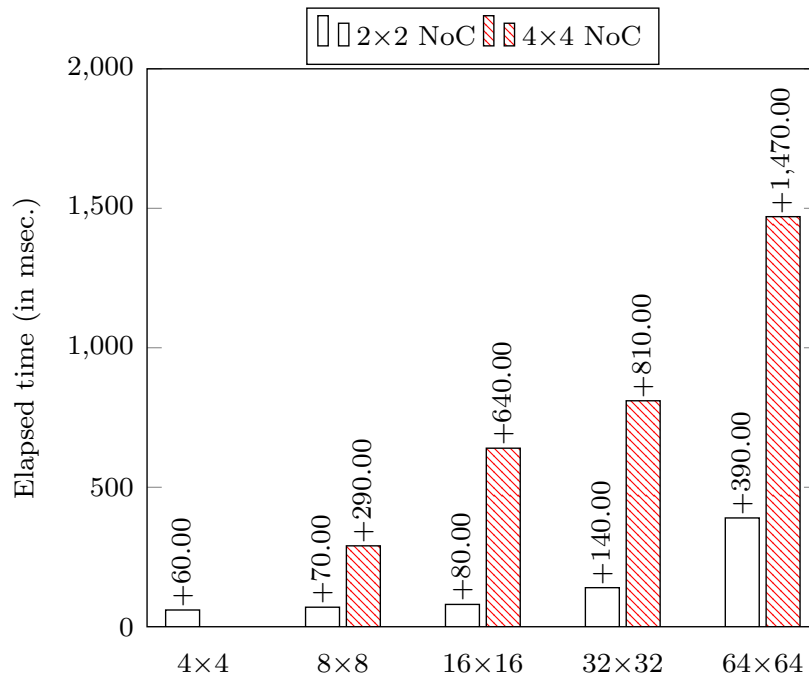
Figure 4.12 – Elapsed time (in msec.) for different sizes of matrix multiplications on 2 \times 2 and 4 \times 4 NoC clustered architectures (12 MicroBlazes and 1 ARM, and 60 MicroBlazes and 1 ARM respectively)
