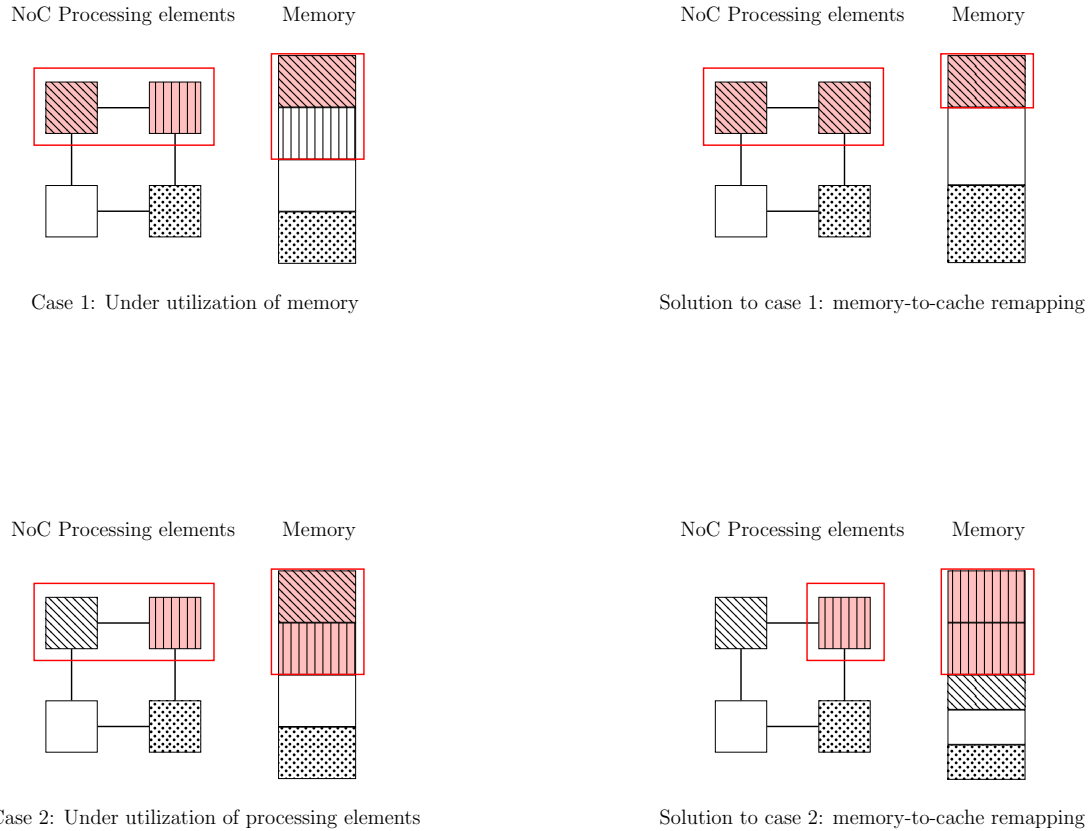
Figure 6.1 – Dynamic memory-to-cache mapping to reduce under-utilization of resources
