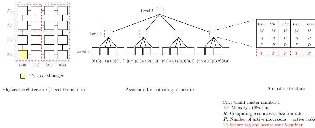
Figure 3.7 – Overview of the kernel monitoring structure
