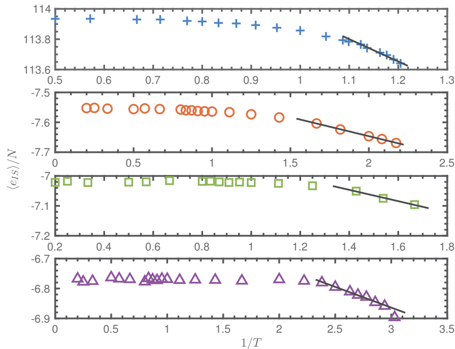
FIGURE 5.3: Evolution of \langle e_{IS} \rangle / N as function of 1/T for the bidisperse Voronoi liquid (+), KA (o), WAHN (□) and AMLJ-0.80 (△). The dark straight line corresponds to a linear fit performed on lowest temperatures.
