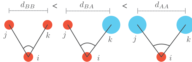
FIGURE 3.6: Representation of the three types of configurations that can be found when the central particle i is small.
