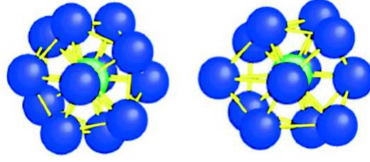
FIGURE 6.2: Left: icosahedron. Right: distorted icosahedron. (Reproduced with permissions from [6], copyright The American Association for the Advancement of Science 2013.)
