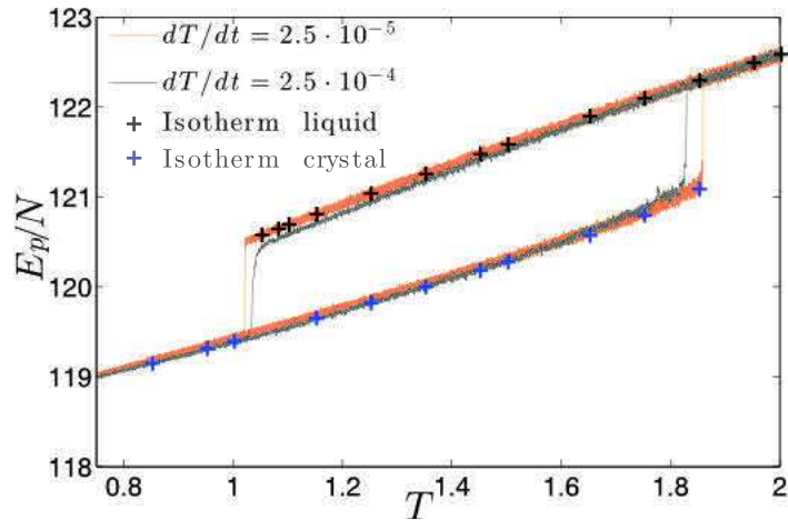
FIGURE 1.12: Representation of the potential energy per particle in the metastability zone for temperatures 1.05 \leq T \leq 1.85 . Grey and orange curves correspond to cooling and heating process at rates respectively dT/dt = 2.5 \cdot 10^{-4} and dT/dt = 2.5 \cdot 10^{-5} . The black and blue crosses are mean values of E_P/N evaluated on several isotherms with respectively N = 8000 and N = 8192 .
