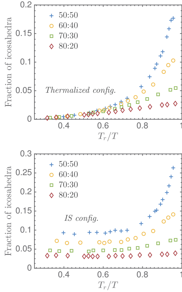
FIGURE 6.5: Evolution of the fraction of icosahedra as a function of T_r/T for different compositions of the bidisperse Voronoi liquid. The upper graph shows the evolution for thermalized configuration whereas the lower graph focuses on IS configurations.
