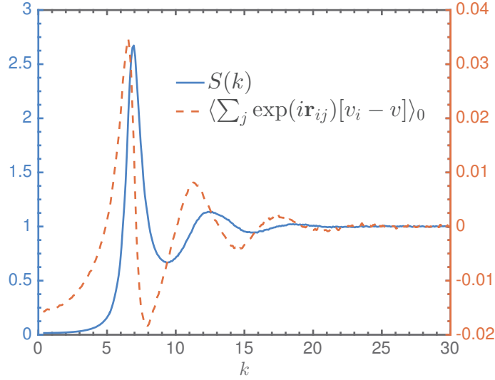
FIGURE 3.14: Representation of the monodisperse structure factor S(k) in blue solid line and \left\langle \sum_j e^{i\mathbf{k} \cdot \mathbf{r}_{ij}} (v_i - v) \right\rangle_0 in dashed red line for T = 2.00 and N = 8000 .
