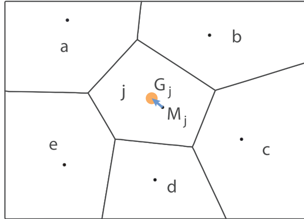
FIGURE 1.1: Representation of 2-dimensional Voronoi tessellation. The polygon associated to the particle j is built from the nearest neighbors of j . Each segment composing the polygon corresponds to the median plane between j and one of its nearest neighbors. The intersection of these median planes defines the polygon.
