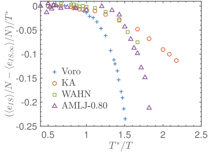
FIGURE 5.2: Evaluation of (\langle e_{IS} \rangle / N - \langle e_{IS,\infty} \rangle / N) / T^* as a function of the scaled temperature T^*/T . Where we recall that T^* is the temperature at which the system enters into the super-Arrhenian regime. T^* = 1.25 for Voronoi, T^* = 1.00 for KA and WAHN and T^* = 0.60 for AMLJ-0.80.
