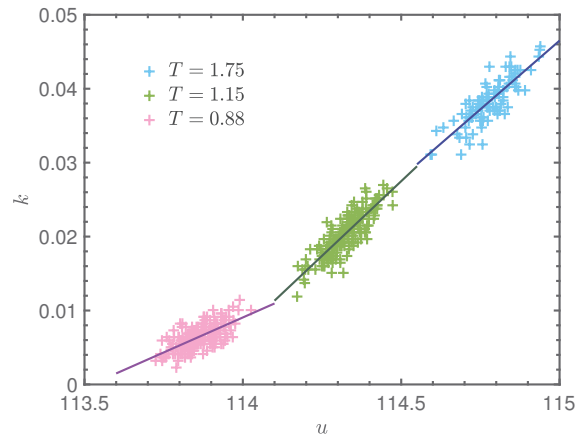
FIGURE 5.20: Representation of the linear regression performed on scatter data. For sake of clarity only 3 temperatures are represented.
