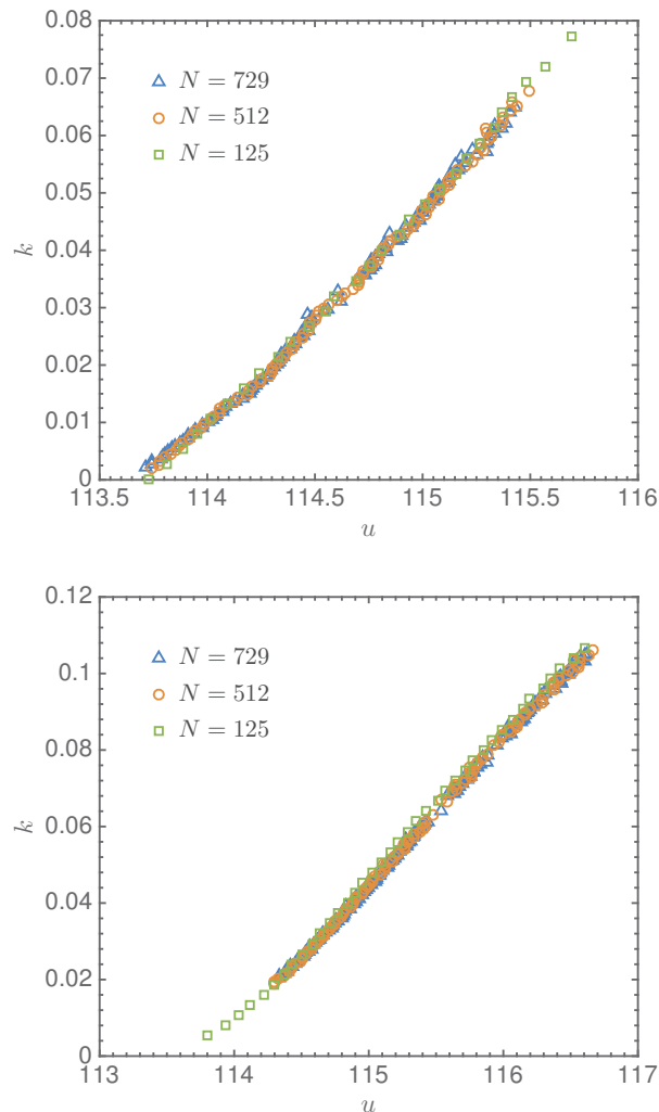
FIGURE 5.18: Representation of the geometric average of k as a function of the energy density u for the 3 systems size. The upper graph is for QS whereas the lower graph is for true saddles.
