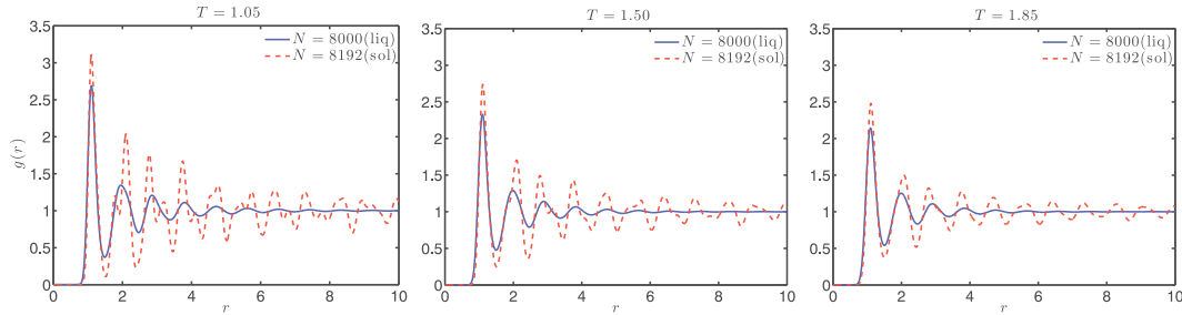
FIGURE 1.13: Representation of the pair correlation function for three temperatures taken in the metastable zone. The straight blue lines correspond to isotherms in the liquid phase with N = 8000 particles whereas the dashed red lines are data from isotherms in the crystalline phase for N = 8192 particles.
