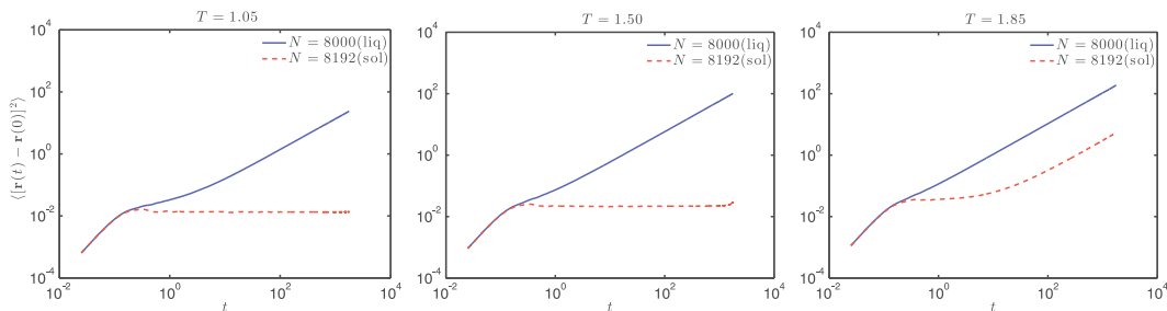
FIGURE 1.14: Representation of the MSD for three temperatures taken in the metastable zone. The straight blue lines correspond to isotherms in the liquid phase with N = 8000 particles whereas the dashed red lines are data from isotherms in the crystalline phase for N = 8192 particles.
